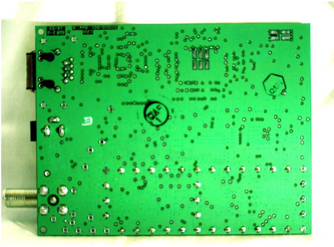
Bottom View
