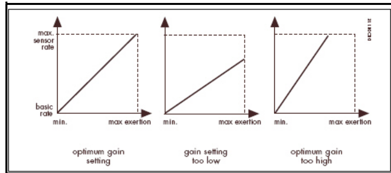
Figure 17: Impact of sensor gain on rate adaptation
