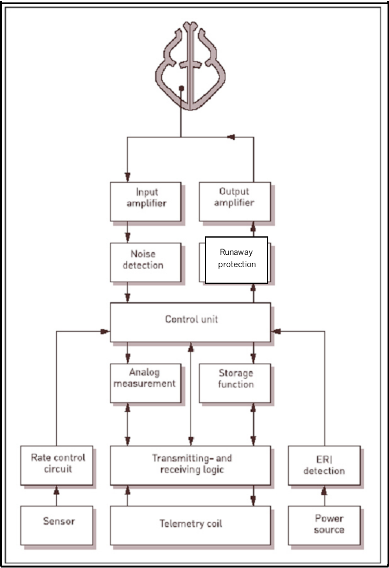
Block Diagram for Cylos VR
