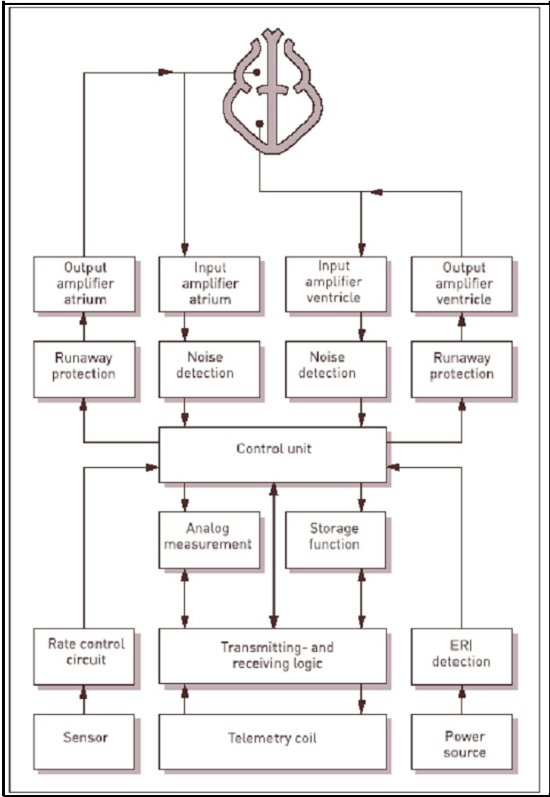
Block Diagram for Cylos DR
