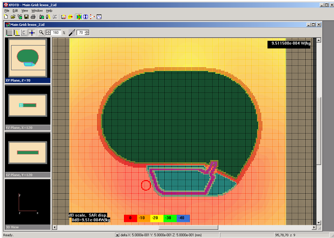
Figure 11 10 gram average maximum SAR depicted by the red circle. The maximum 10 gram average is 951 \mu W/kg.
