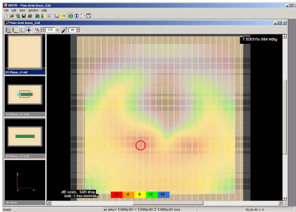
Figure 13 1 gram SAR average 5 mm below Lexos. A maximum SAR of 793 \mu W/kg is indicated.
