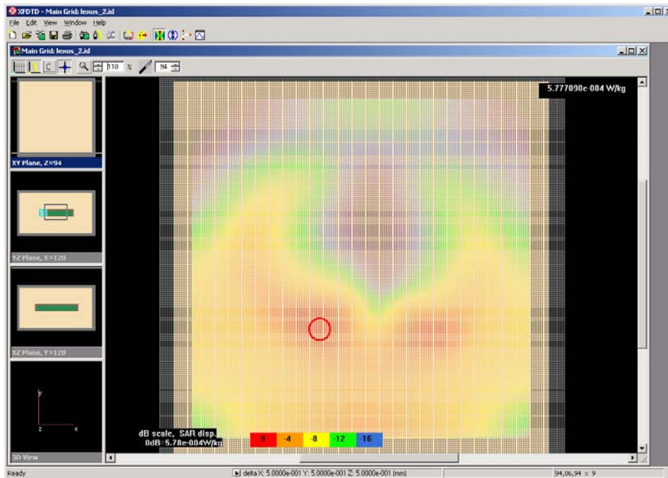
Figure 12 1 gram SAR average 5 mm above Lexos. A maximum SAR of 578 \mu W/kg is indicated.
