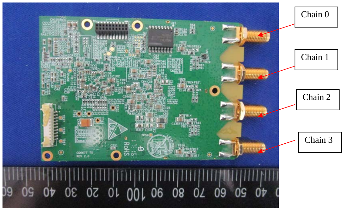
EUT – RX PCB-1 Bottom View
