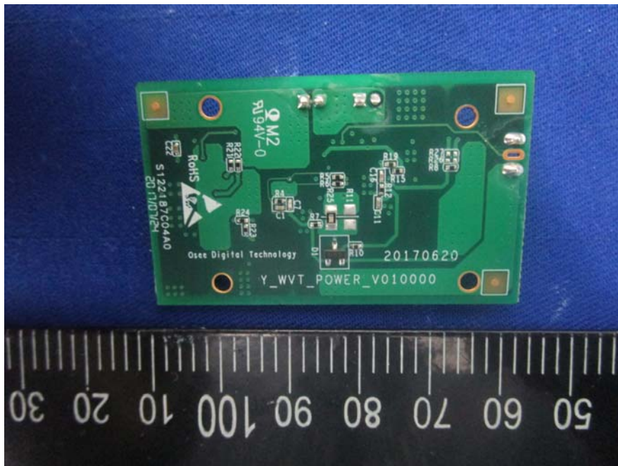
EUT –RX PCB-2 Bottom View
