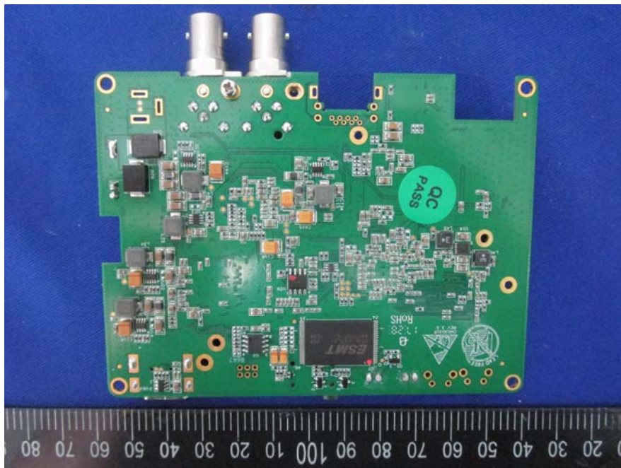
EUT – RX Main Board Bottom View
