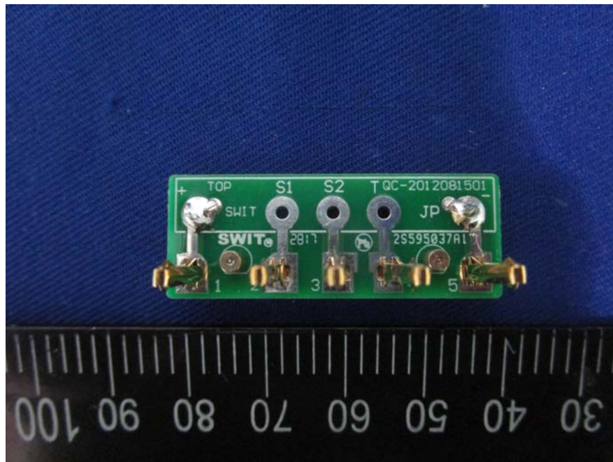
EUT –RX PCB-5 Top View
