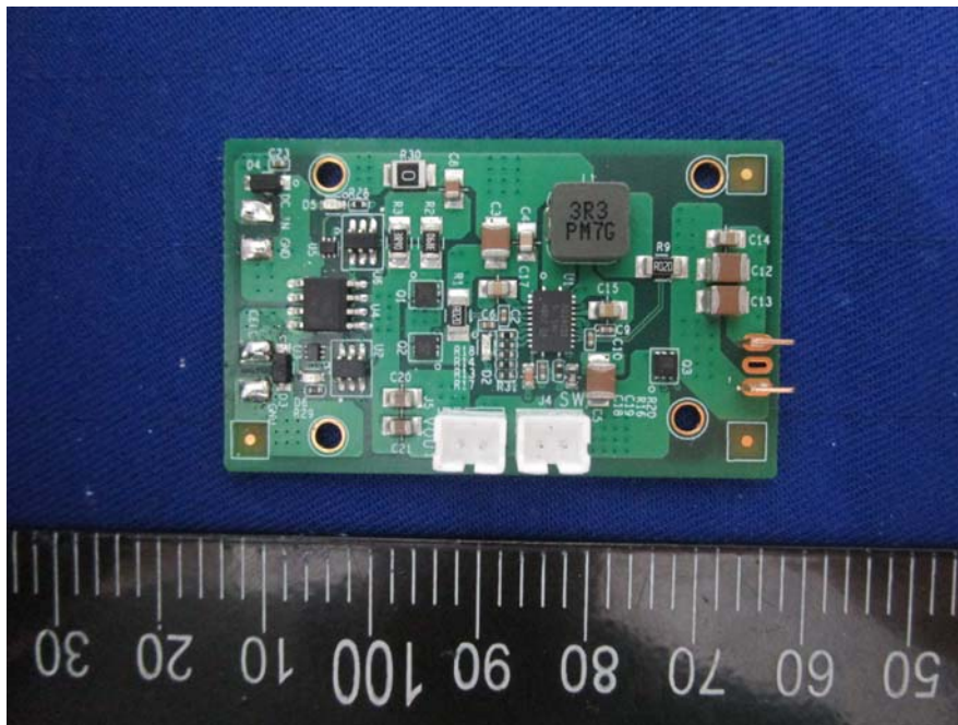
EUT – RX PCB-2 Top View
