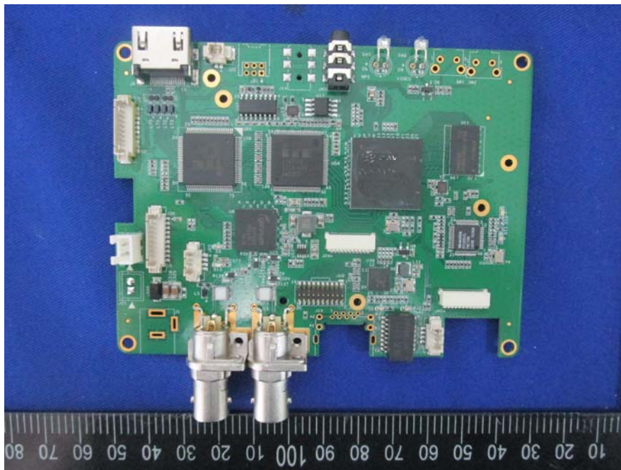
EUT –RX Main Board Top Uncover View
