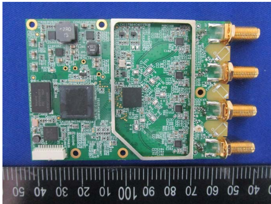
EUT –RX PCB-1 Top Uncover View
