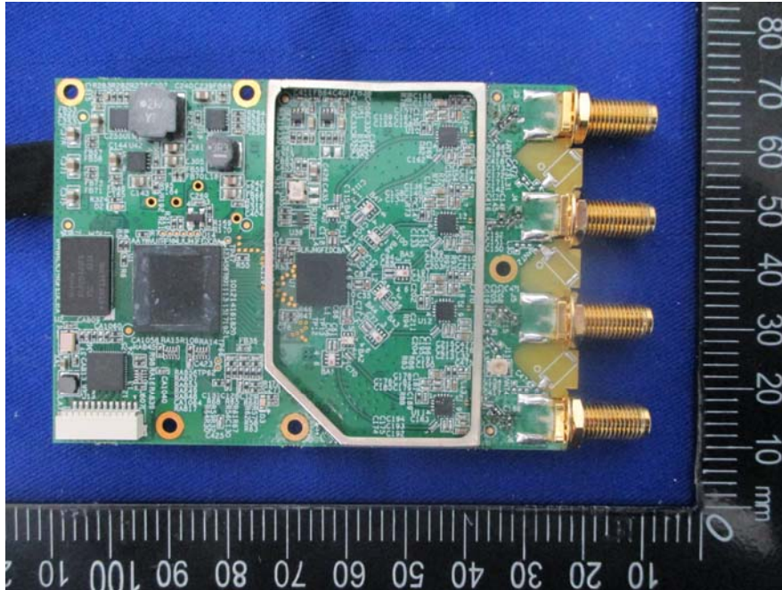
EUT – PCB1 Top Uncover View
