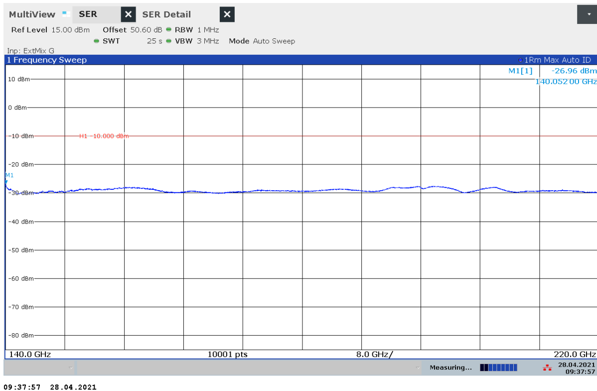
Plot 34: 140 GHz – 220 GHz, stopped mode (sweep stopped in the middle of the range of operation)
