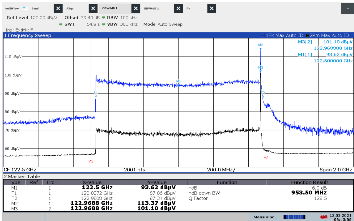
Plot 2: Sample 5 (Delta-Test), 6 dB OBW
