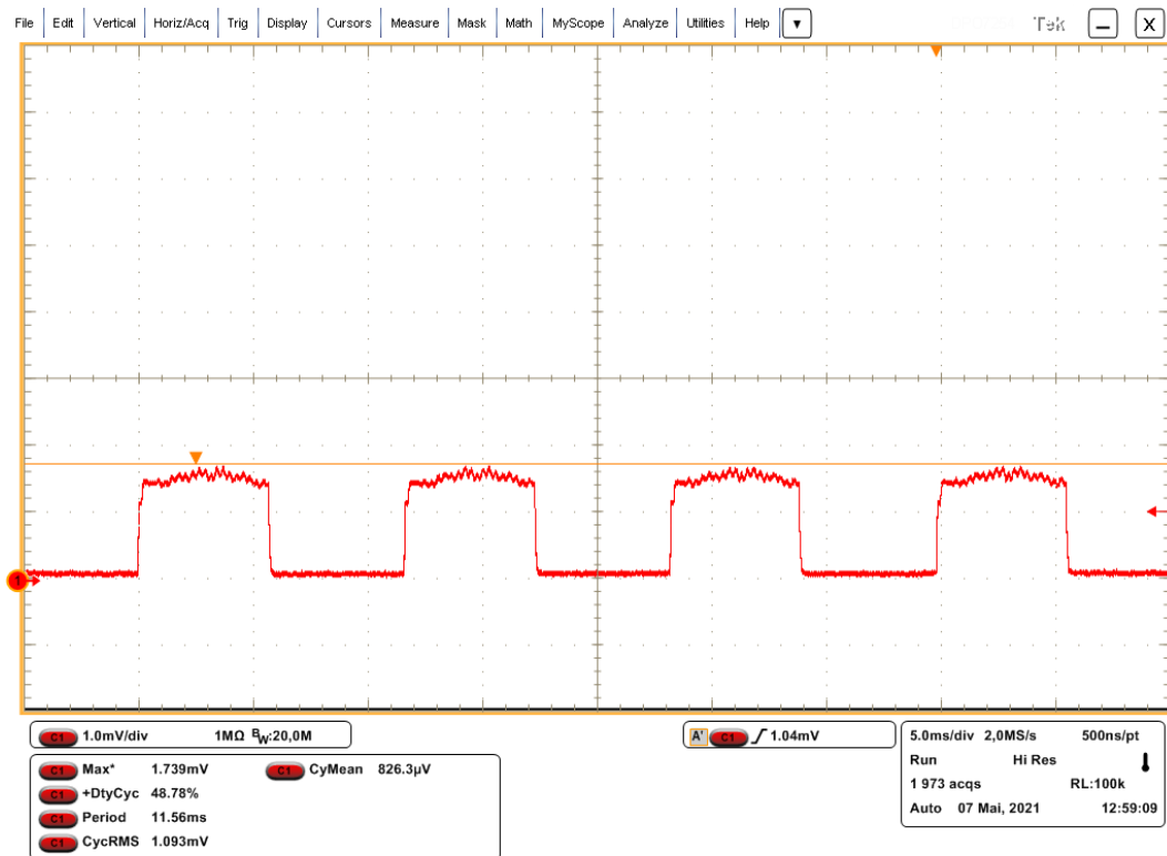
Plot 7: Sample 6, Duty cycle
