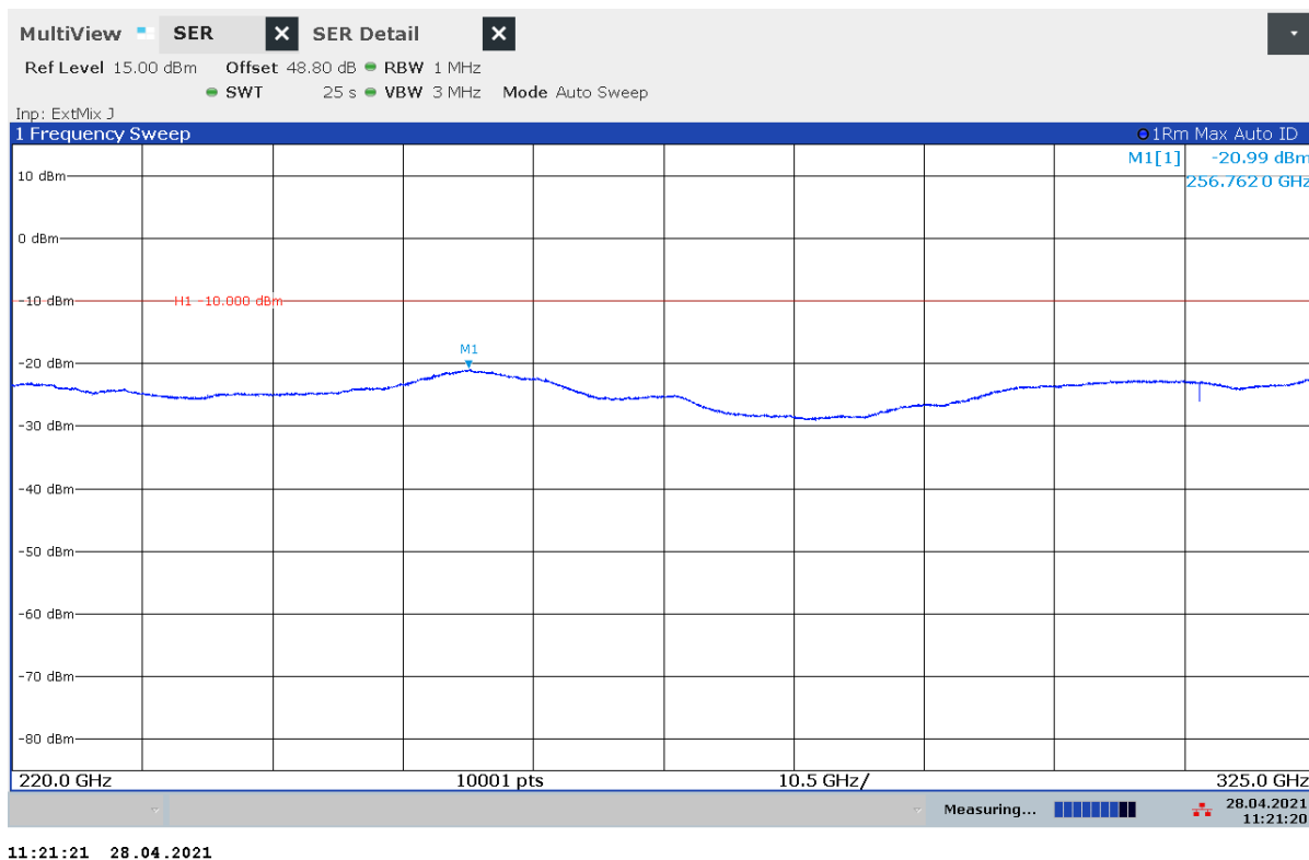
Plot 36: 220 GHz – 325 GHz, stopped mode (sweep stopped in the middle of the range of operation)
