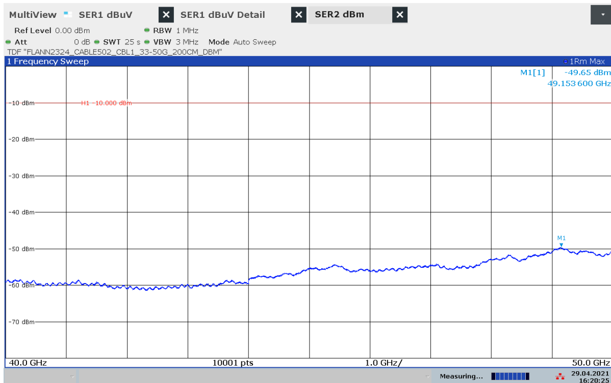
Plot 20: 40 GHz – 50 GHz, stopped mode (sweep stopped in the middle of the range of operation)
