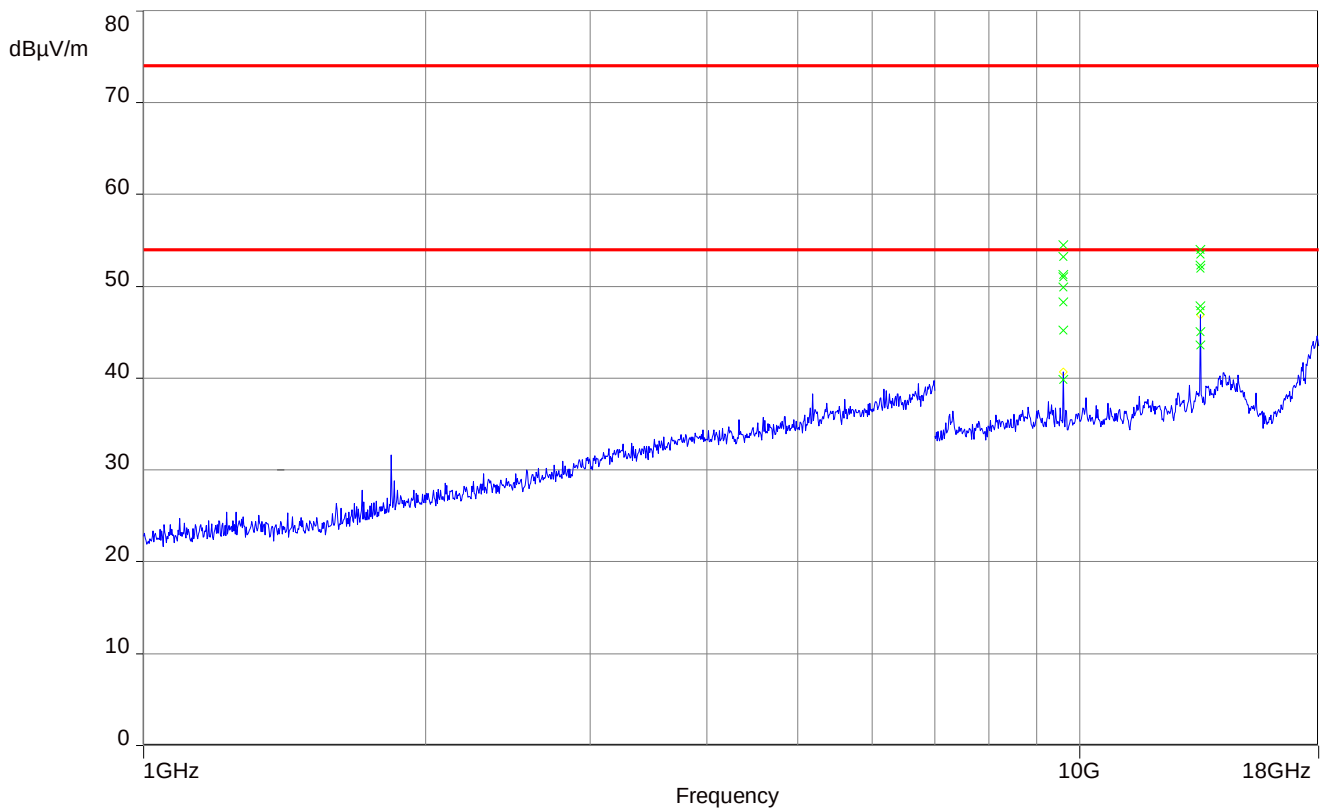
Plot 16: 1 GHz – 18 GHz, stopped mode (sweep stopped near the top of the range of operation)
