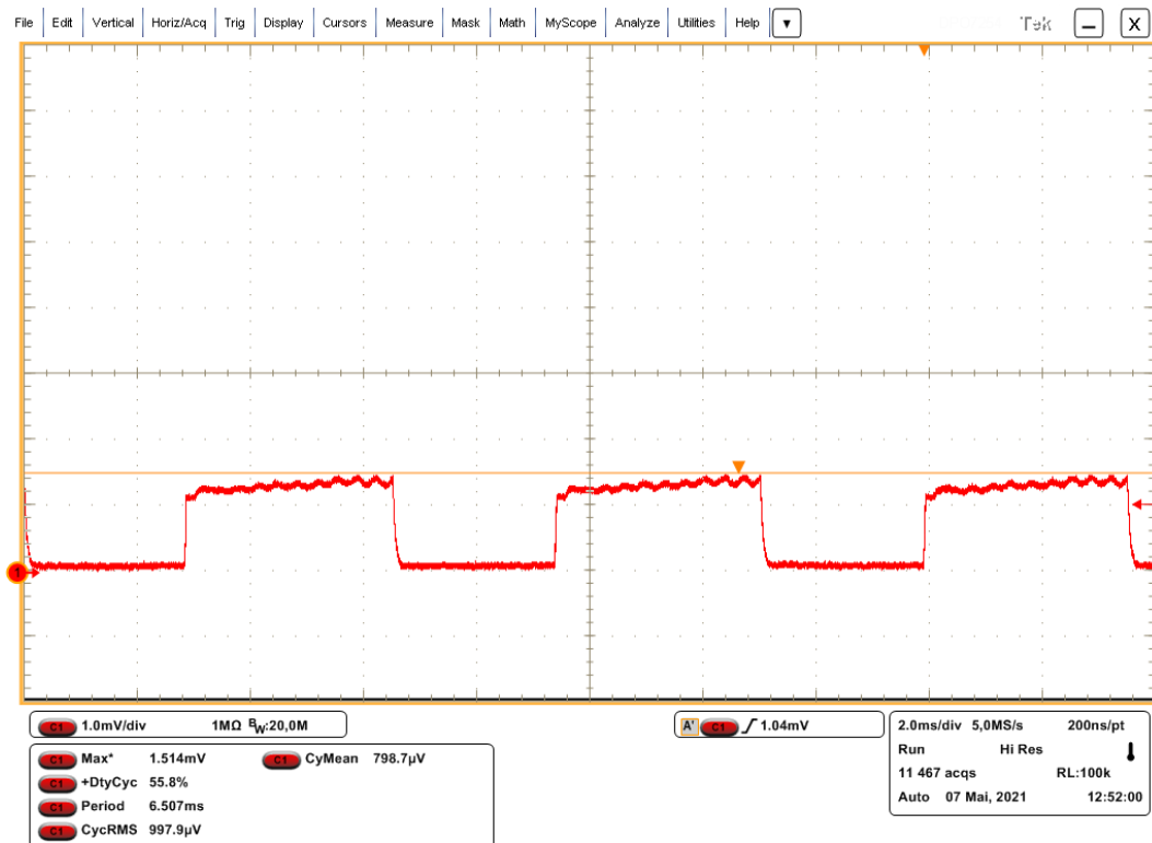
Plot 8: Sample 11, Duty cycle
