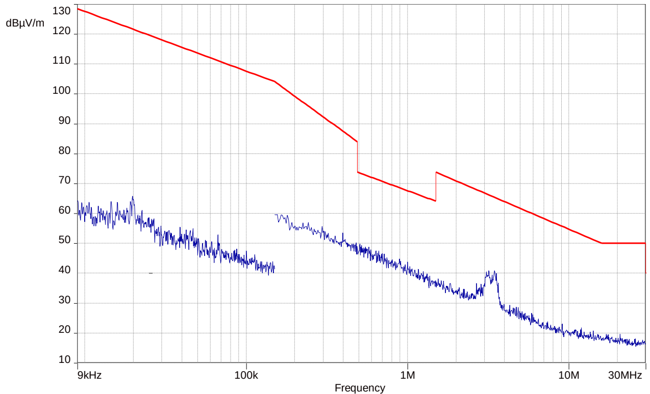
Plot 10: 9 kHz – 30 MHz, stopped mode (sweep stopped in the middle of the range of operation)
