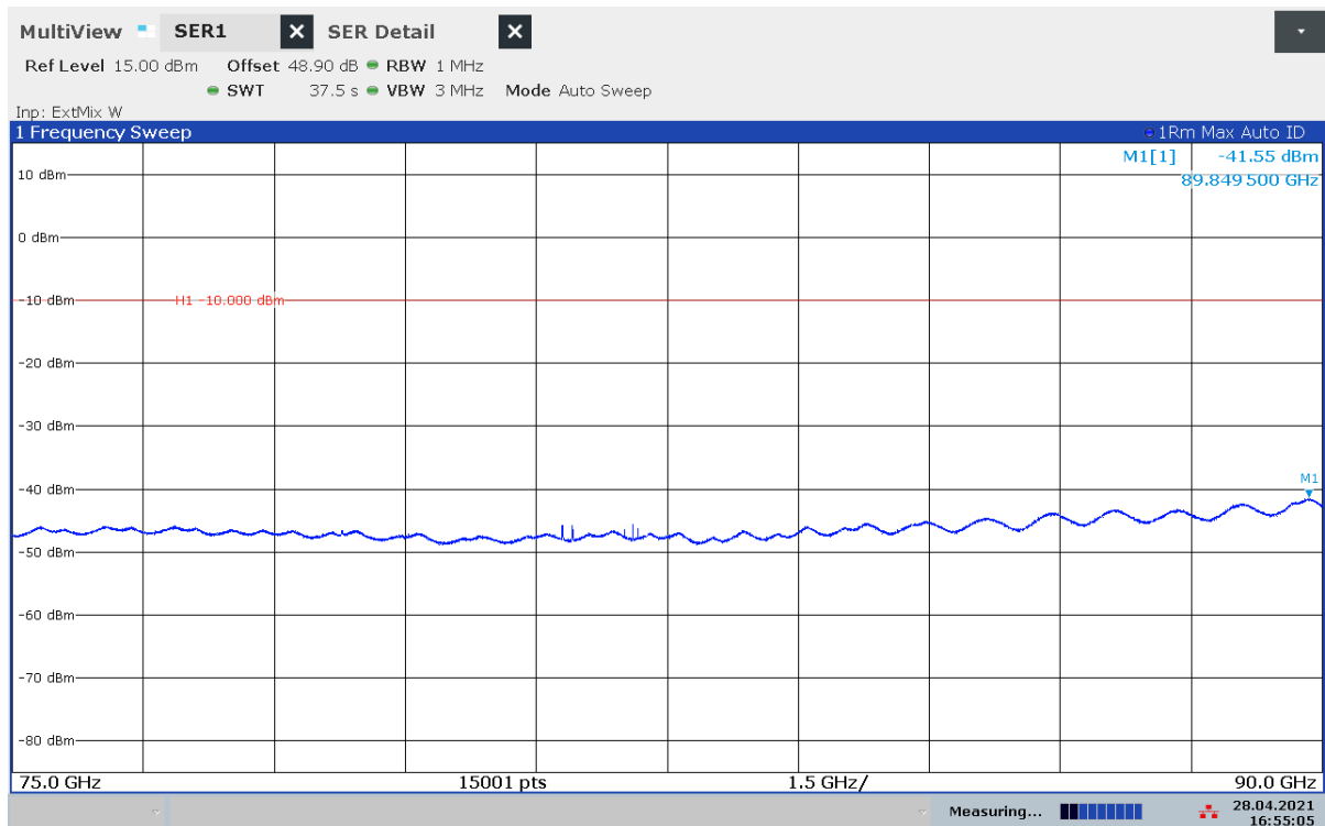
Plot 24: 75 GHz – 90 GHz, stopped mode (sweep stopped in the middle of the range of operation)
