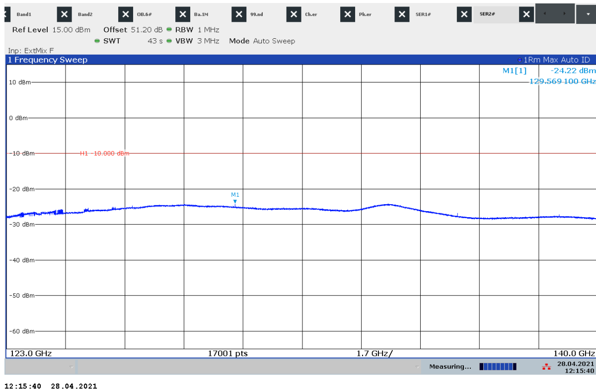
Plot 32: 123 GHz – 140 GHz, stopped mode (sweep stopped in the middle of the range of operation)
