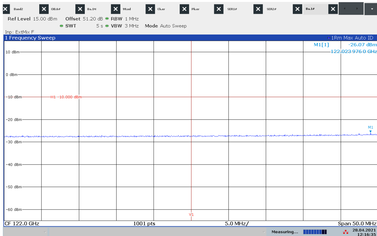
Plot 28: lower band edge compliance, stopped mode (sweep stopped in the middle of the range of operation)
