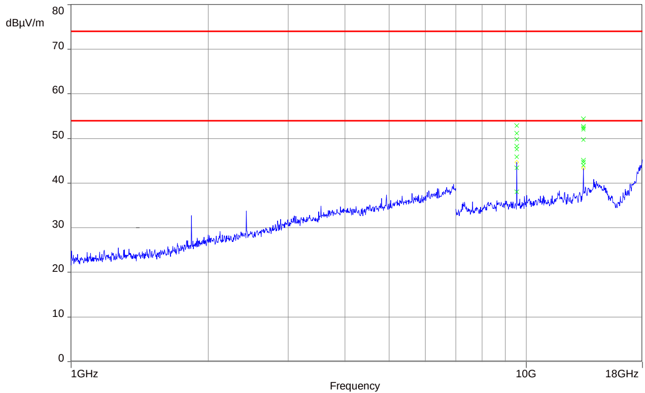
Plot 14: 1 GHz – 18 GHz, stopped mode (sweep stopped near the bottom of the range of operation)
