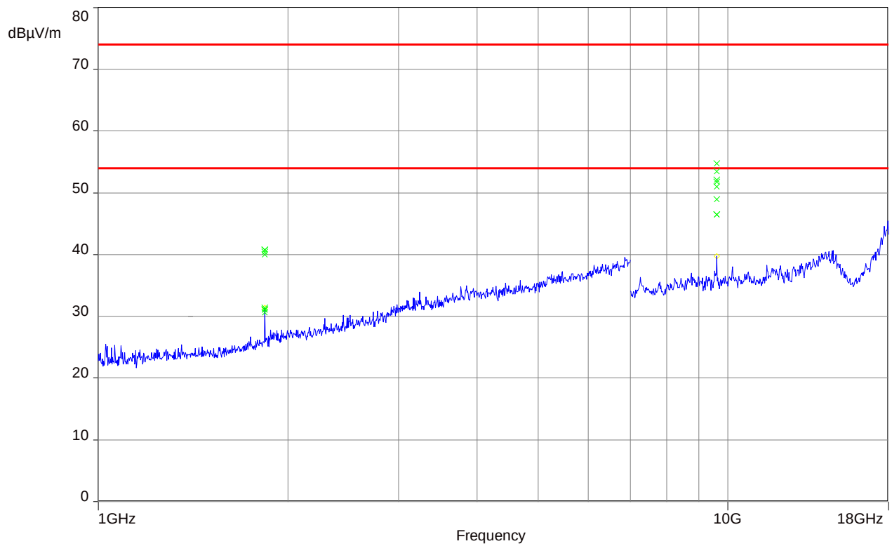
Plot 13: 1 GHz – 18 GHz, normal mode
