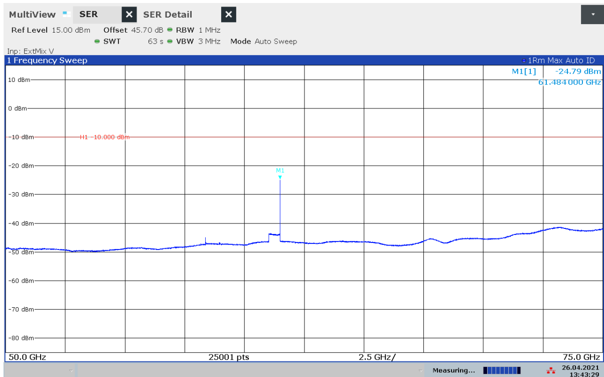
Plot 21: 50 GHz – 75 GHz, normal mode
