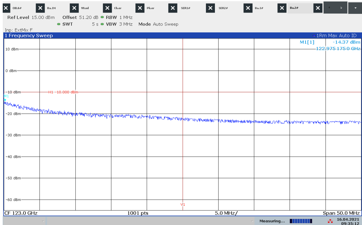
Plot 29: upper band edge compliance, normal mode
