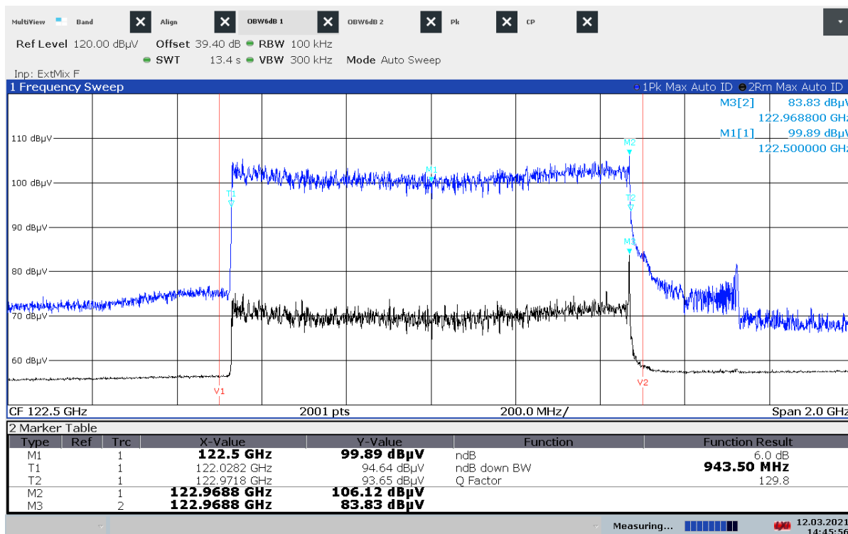
Plot 4: Sample 11 (Delta-Test), 6 dB OBW
