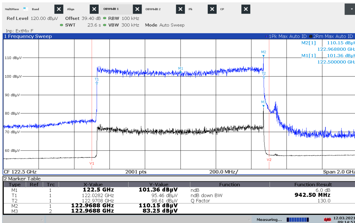
Plot 3: Sample 6 (Delta-Test), 6 dB OBW
