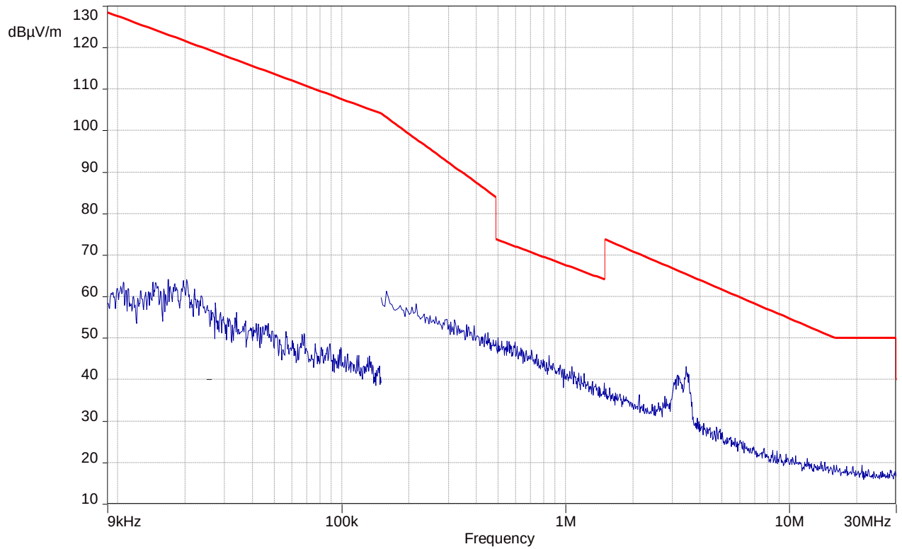
Plot 9: 9 kHz – 30 MHz, normal mode
