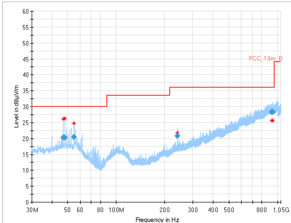
Plot 12: 30 MHz – 1 GHz, stopped mode (sweep stopped in the middle of the range of operation)
