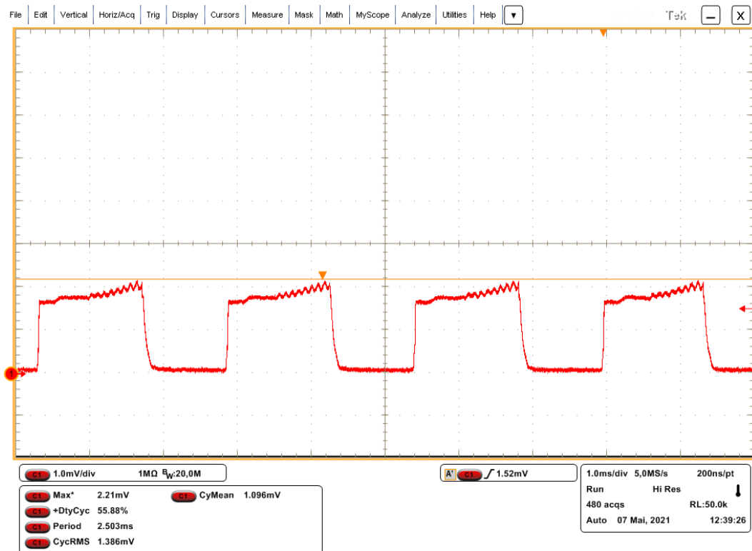
Plot 5: Sample 7b, Duty cycle
