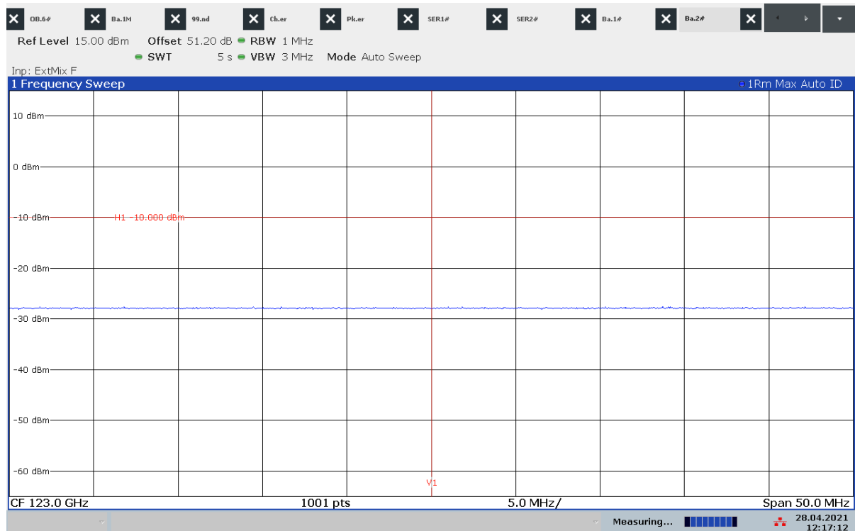
Plot 30: upper band edge compliance, stopped mode (sweep stopped in the middle of the range of operation)
