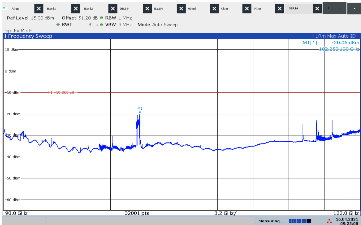
Plot 25: 90 GHz – 122 GHz, normal mode
