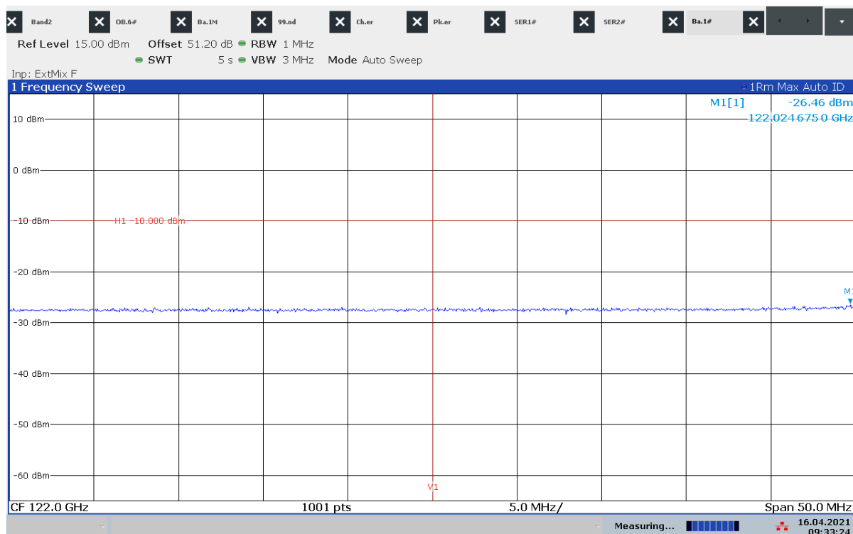
Plot 27: lower band edge compliance, normal mode
