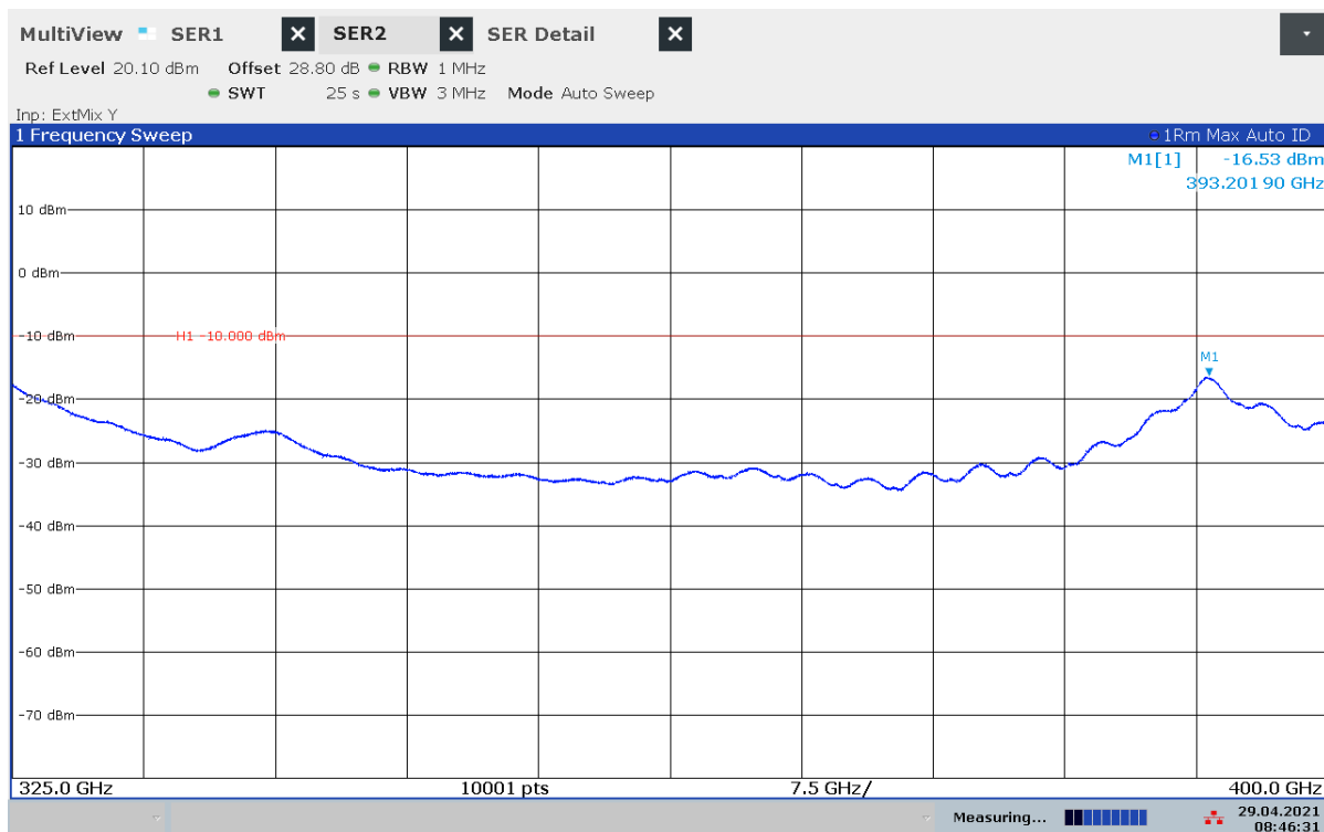
Plot 38: 325 GHz – 400 GHz, stopped mode (sweep stopped in the middle of the range of operation)
