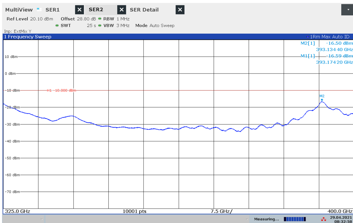
Plot 37: 325 GHz – 400 GHz, normal mode
