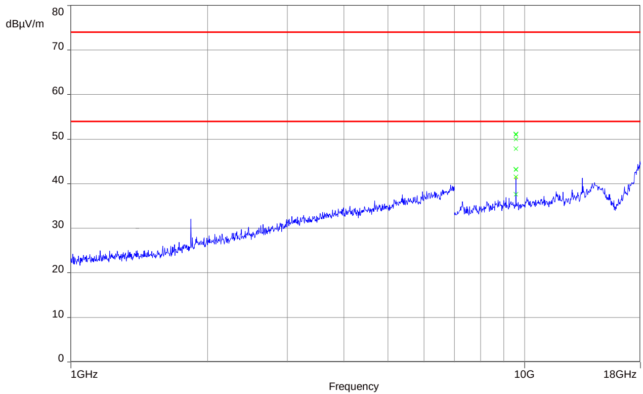
Plot 15: 1 GHz – 18 GHz, stopped mode (sweep stopped in the middle of the range of operation)
