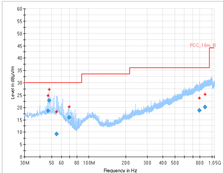
Plot 11: 30 MHz – 1 GHz, normal mode
