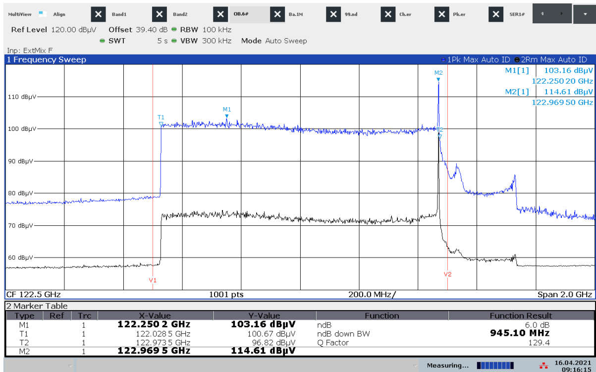
Plot 1: Sample 7b, 6 dB OBW
