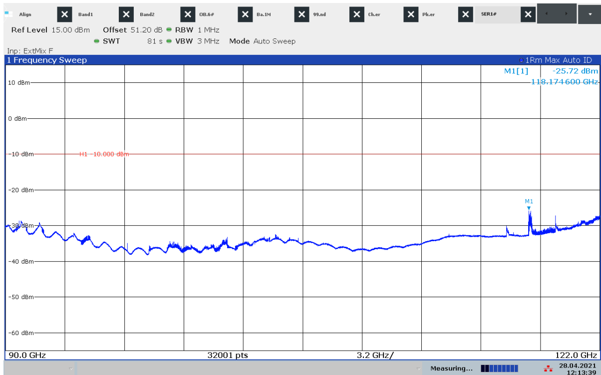
Plot 26: 90 GHz – 122 GHz, stopped mode (sweep stopped in the middle of the range of operation)
