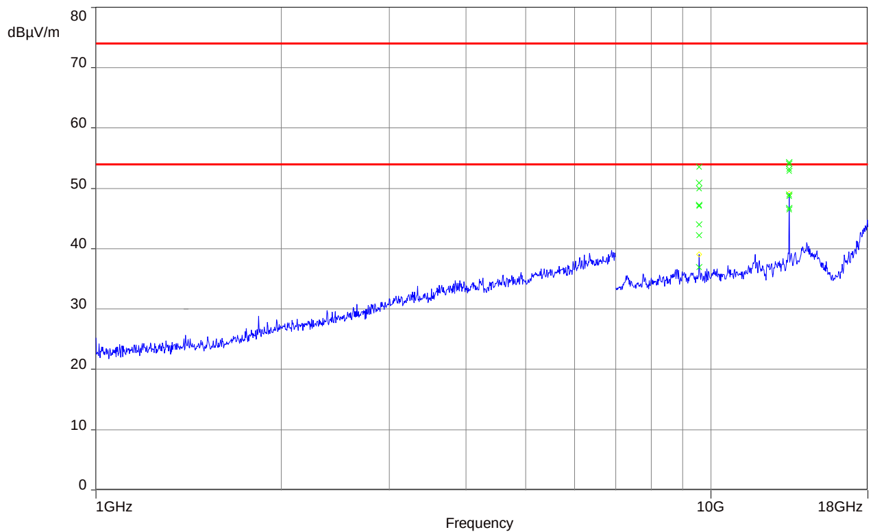
Plot 9: 1 GHz – 18 GHz, stopped mode (sweep stopped in the middle of the range of operation)
