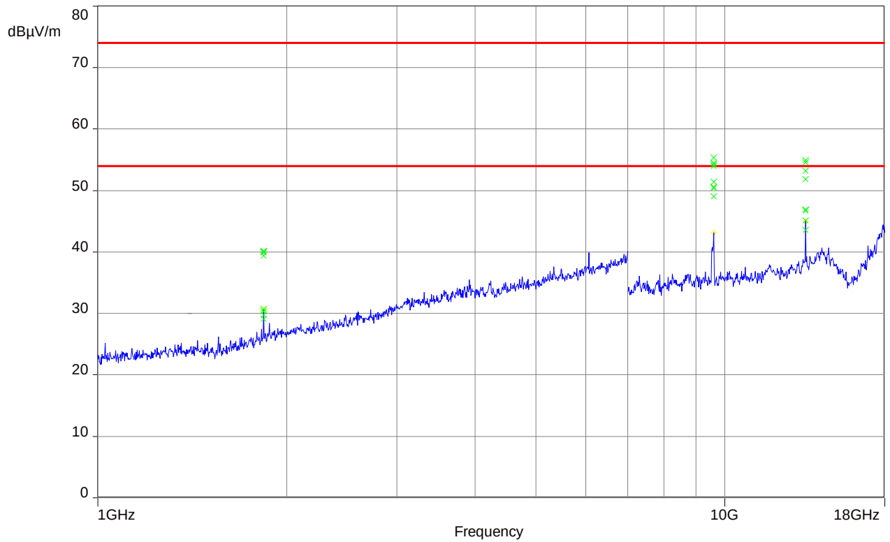
Plot 7: 1 GHz – 18 GHz, normal mode
