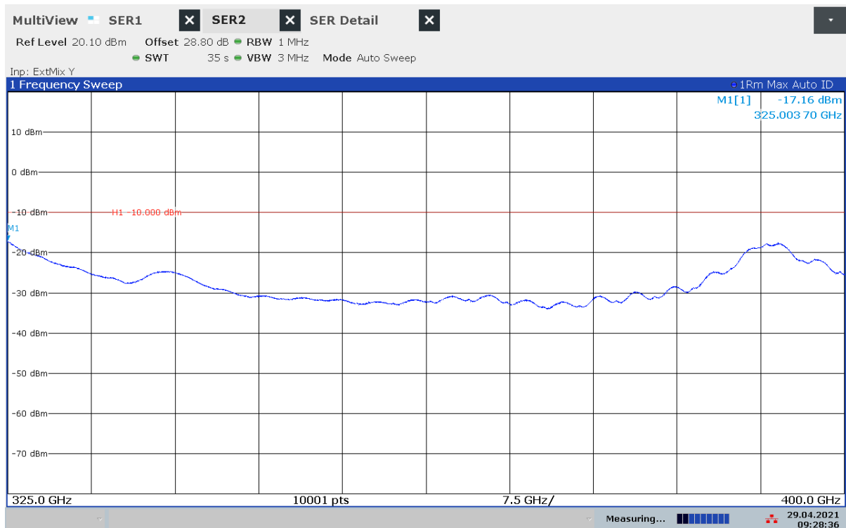
Plot 31: 325 GHz – 400 GHz, normal mode
