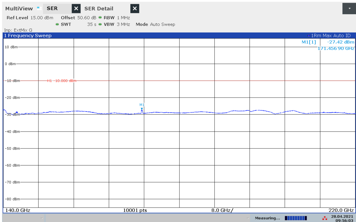
Plot 27: 140 GHz – 220 GHz, normal mode
