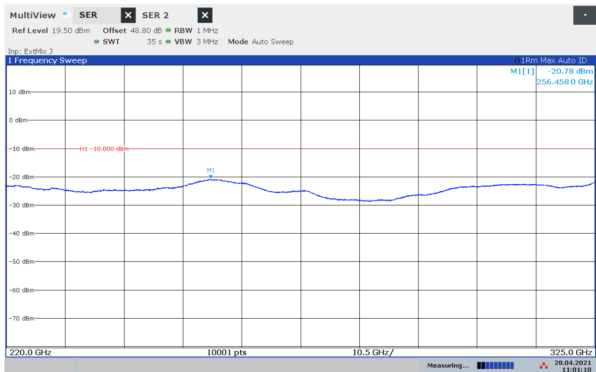
Plot 30: 220 GHz – 325 GHz, stopped mode (sweep stopped in the middle of the range of operation)
