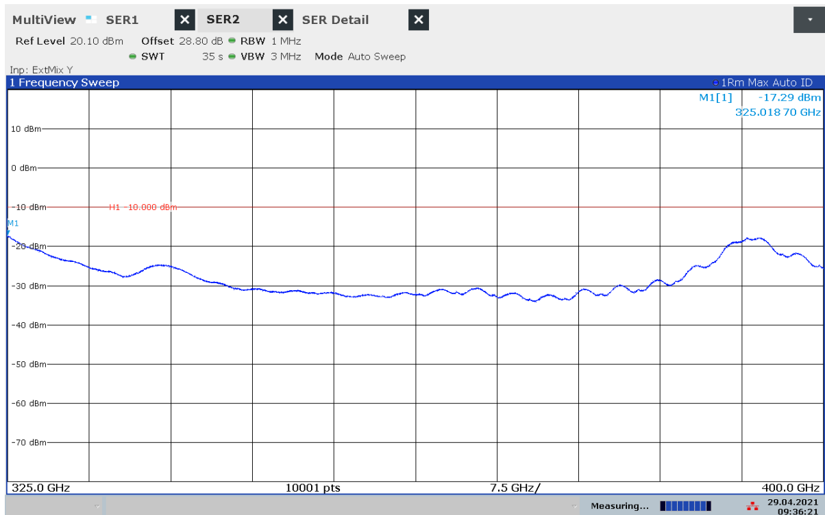
Plot 32: 325 GHz – 400 GHz, stopped mode (sweep stopped in the middle of the range of operation)
