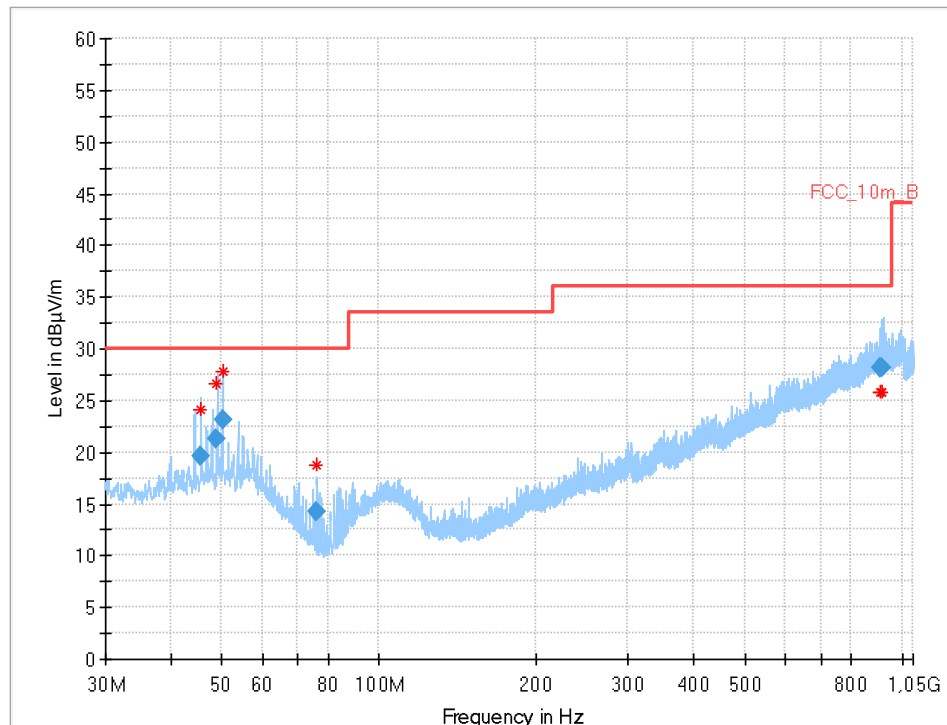
Plot 6: 30 MHz – 1 GHz, stopped mode (sweep stopped in the middle of the range of operation)
