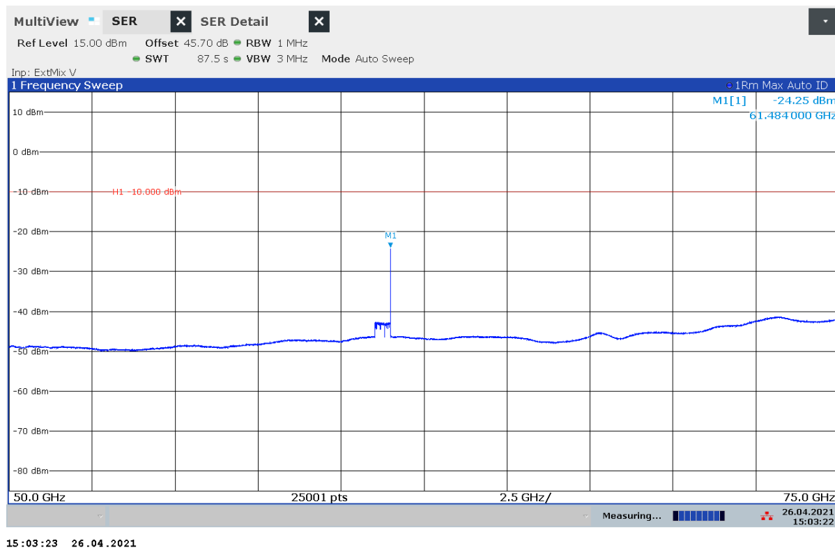
Plot 16: 50 GHz – 75 GHz, stopped mode (sweep stopped near the middle of the range of operation)
