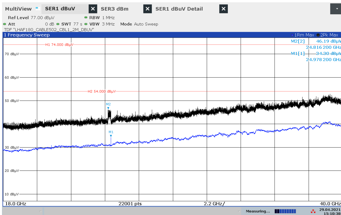
Plot 11: 18 GHz – 40 GHz, normal mode
