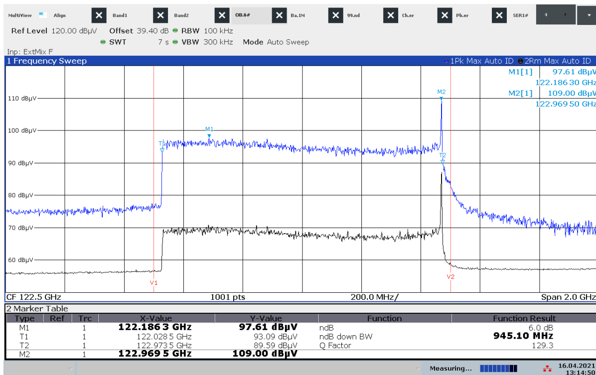
Plot 1: Sample 1b, 6 dB OBW
