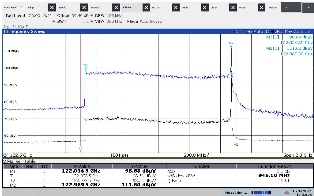
Plot 36: T_{nom} / V_{min}
