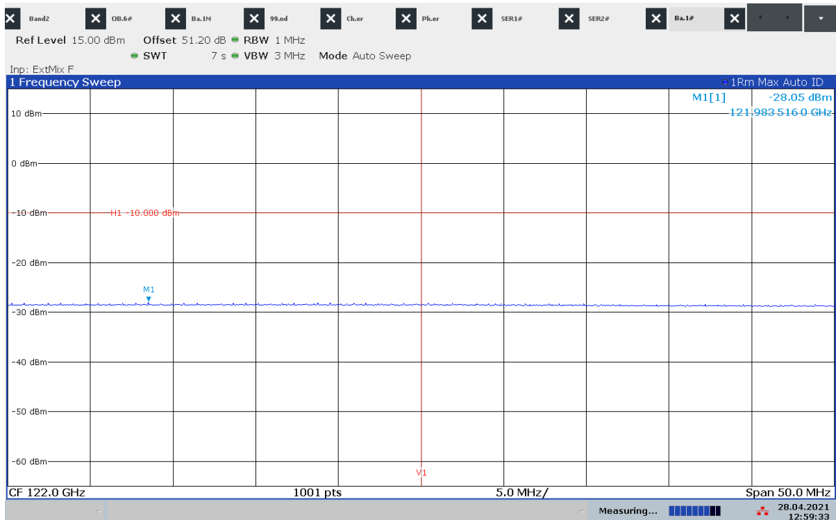
Plot 22: lower band edge compliance, stopped mode (sweep stopped in the middle of the range of operation)
