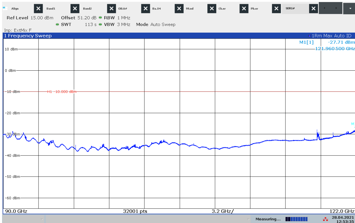
Plot 20: 90 GHz – 122 GHz, stopped mode (sweep stopped in the middle of the range of operation)
