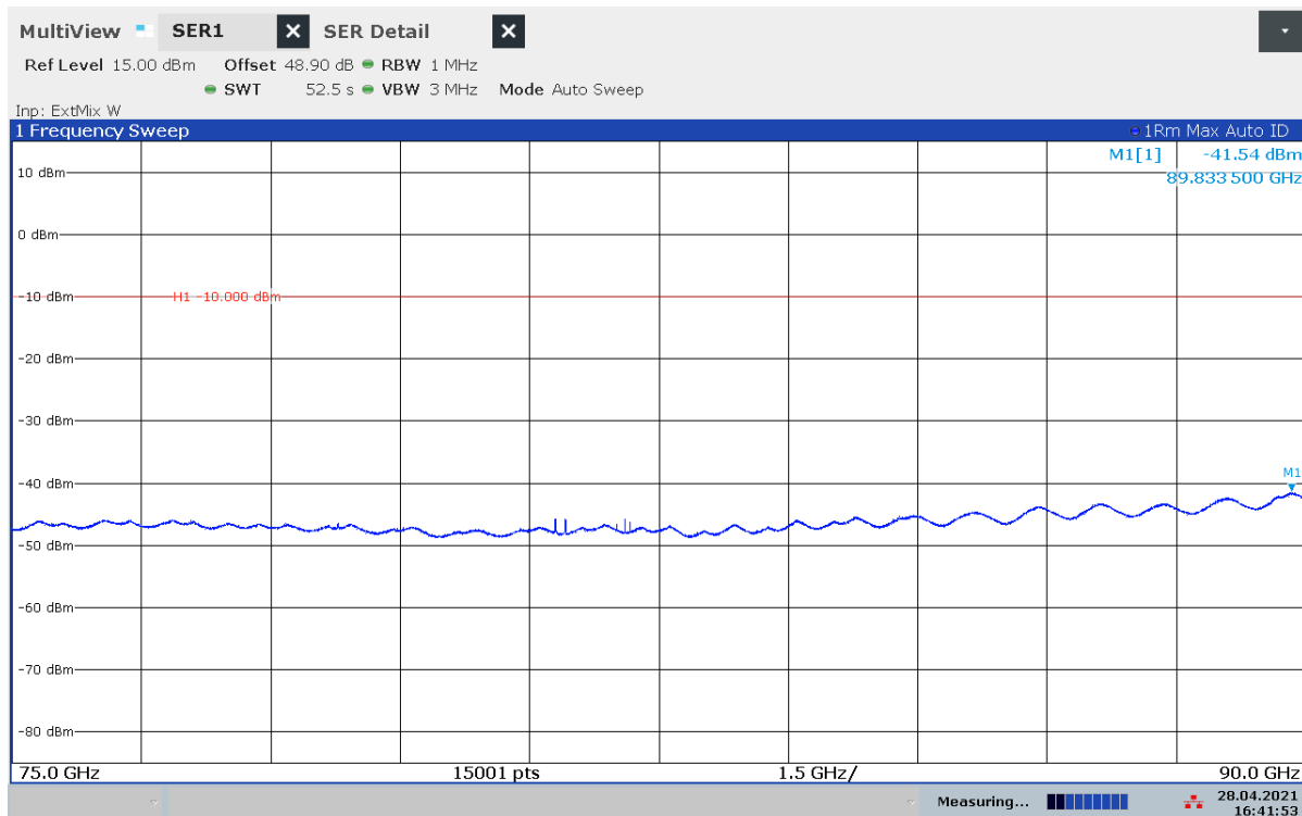
Plot 18: 75 GHz – 90 GHz, stopped mode (sweep stopped in the middle of the range of operation)
