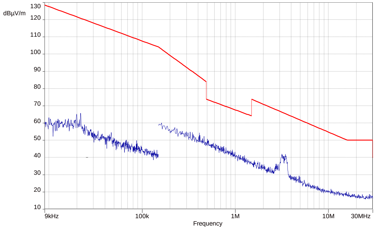
Plot 4: 9 kHz – 30 MHz, stopped mode (sweep stopped in the middle of the range of operation)
