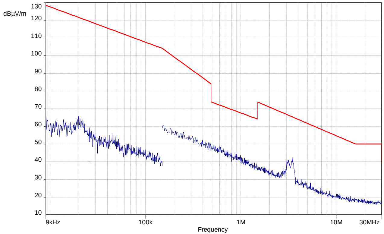
Plot 3: 9 kHz – 30 MHz, normal mode
