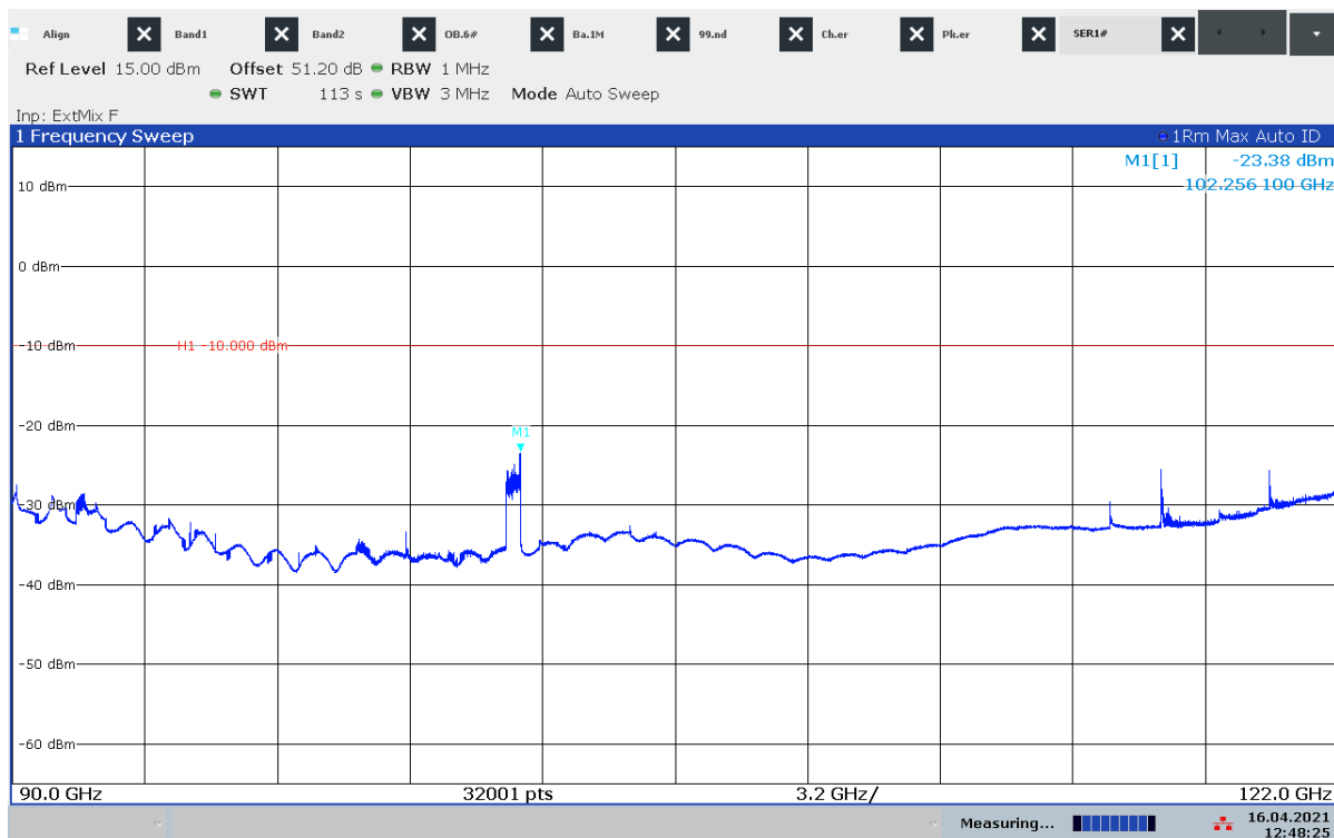
Plot 19: 90 GHz – 122 GHz, normal mode
