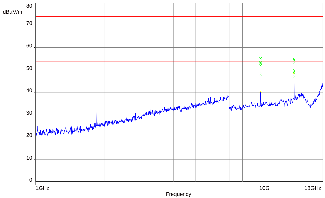
Plot 10: 1 GHz – 18 GHz, stopped mode (sweep stopped near the top of the range of operation)
