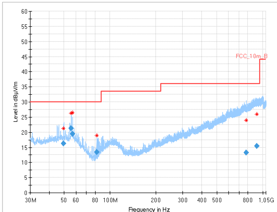
Plot 5: 30 MHz – 1 GHz, normal mode
