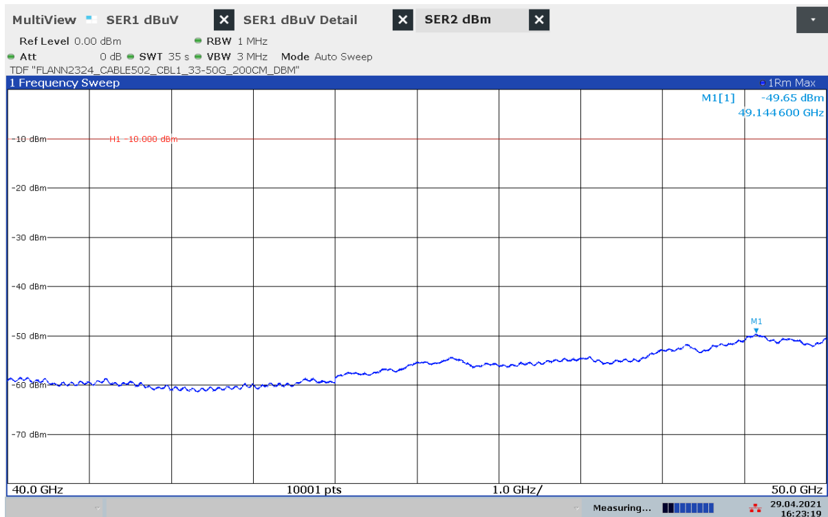
Plot 13: 40 GHz – 50 GHz, normal mode
