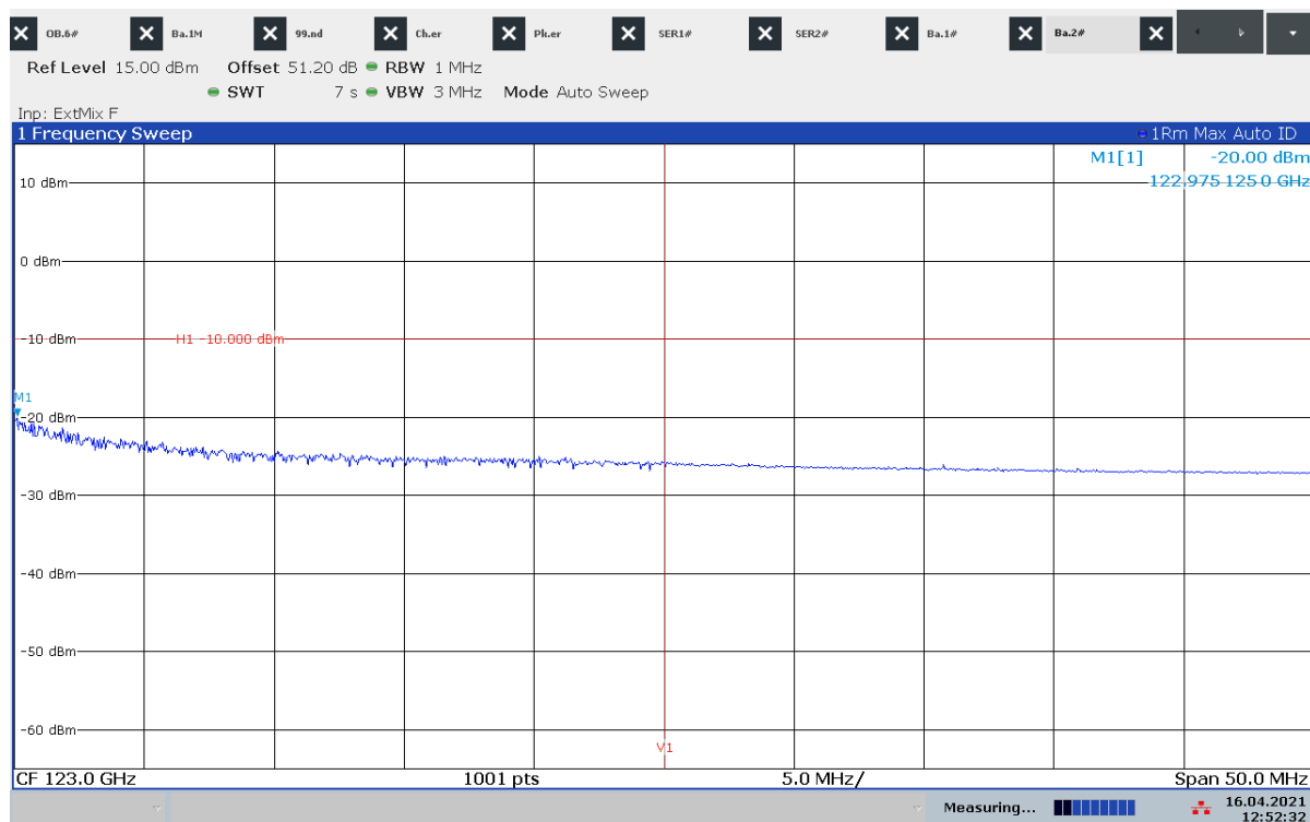
Plot 23: upper band edge compliance, normal mode
