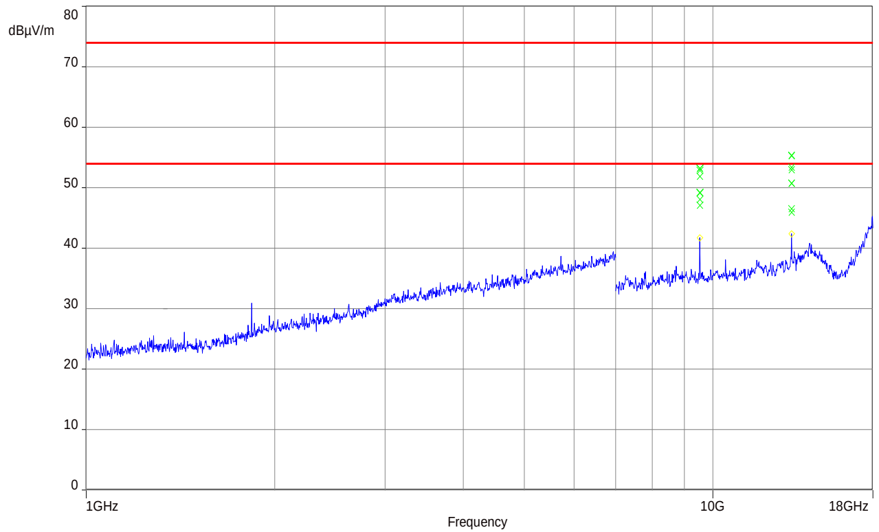
Plot 8: 1 GHz – 18 GHz, stopped mode (sweep stopped near the bottom of the range of operation)
