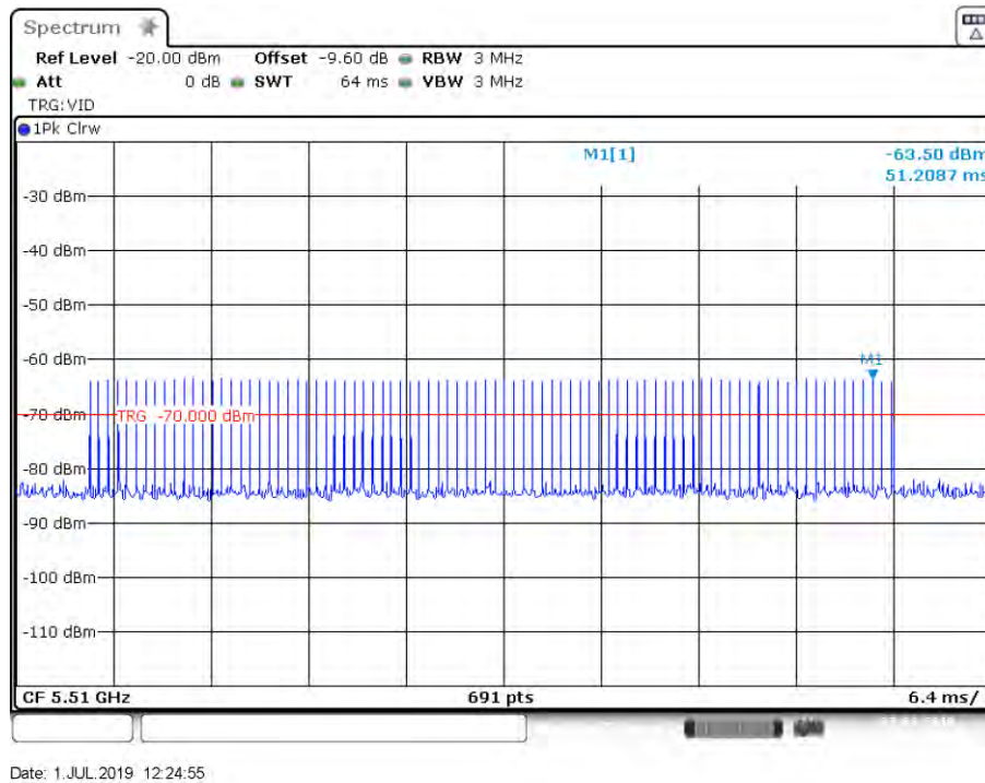
Figure 6: Radar Type 1A DFS Detection Threshold Level at 5510 MHz
