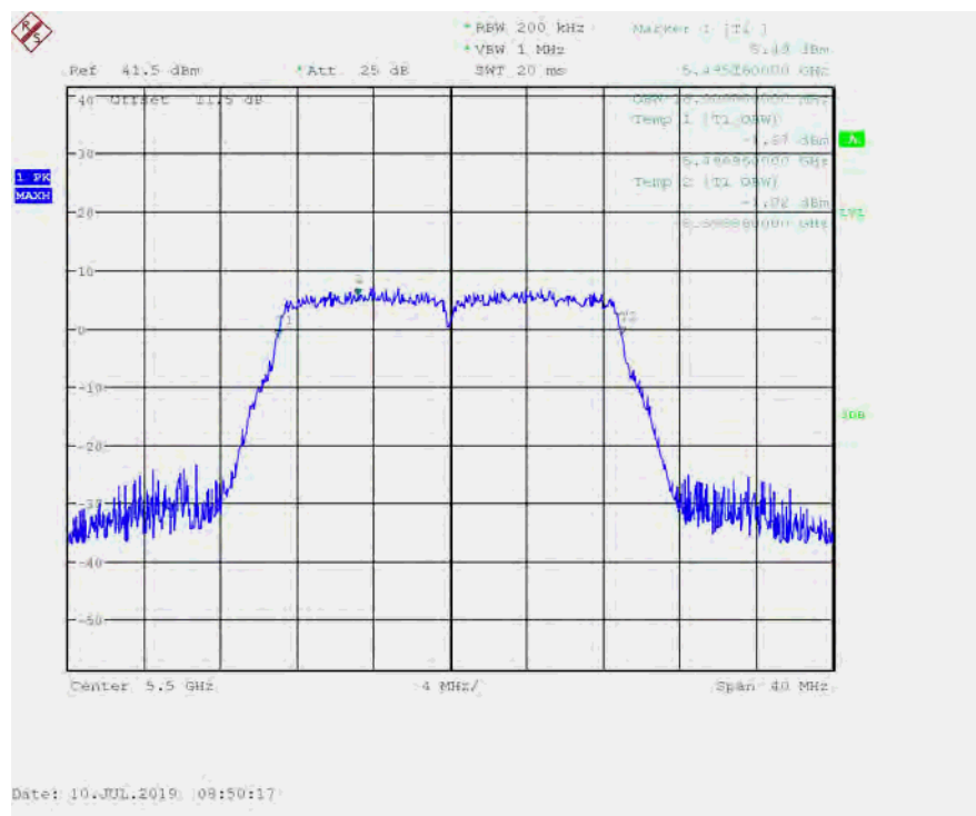
Figure 29: 99% Bandwidth at 5500 MHz (18.00 MHz)
