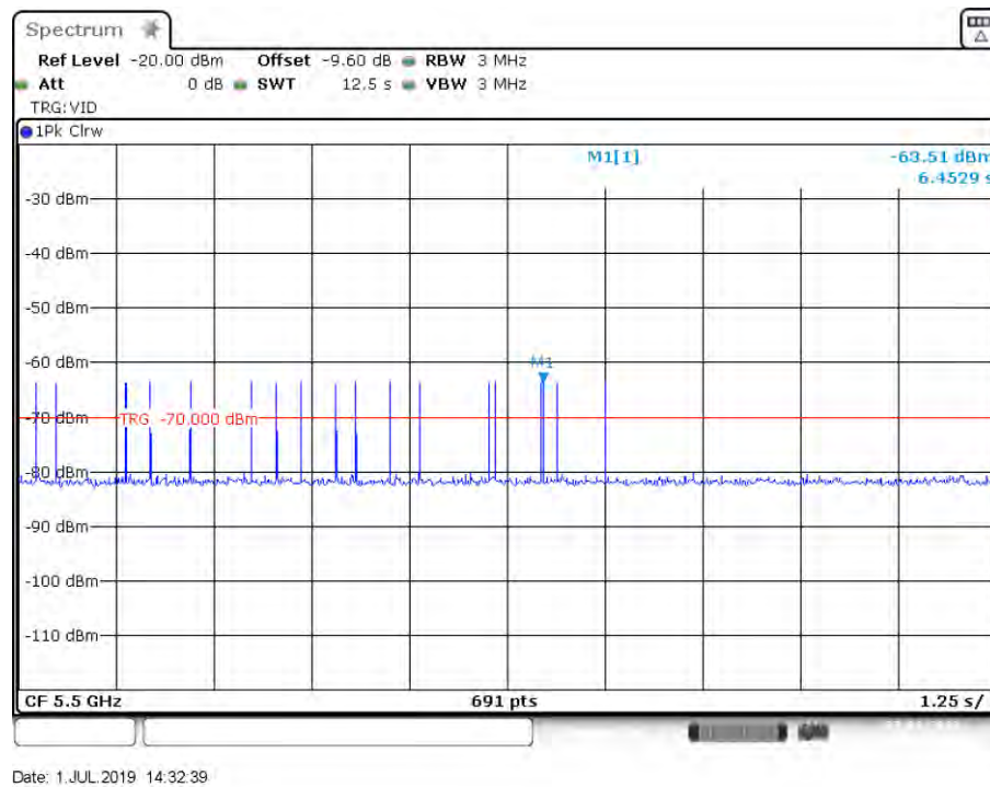
Figure 20: Radar Type 5 DFS Detection Threshold Level at 5500 MHz
