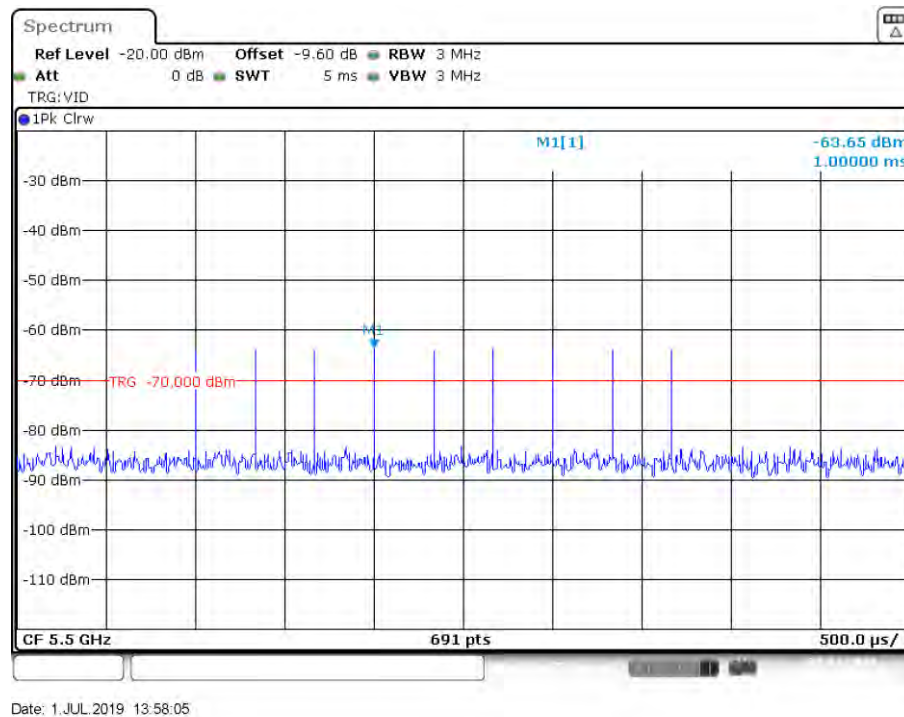
Figure 23: Radar Type 6 DFS Detection Threshold Level at 5500 MHz
