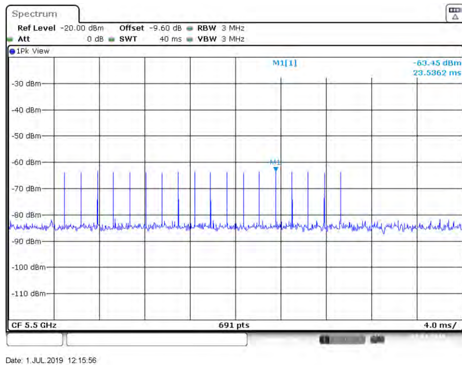
Figure 2: Radar Type 0 DFS Detection Threshold Level at 5500 MHz
