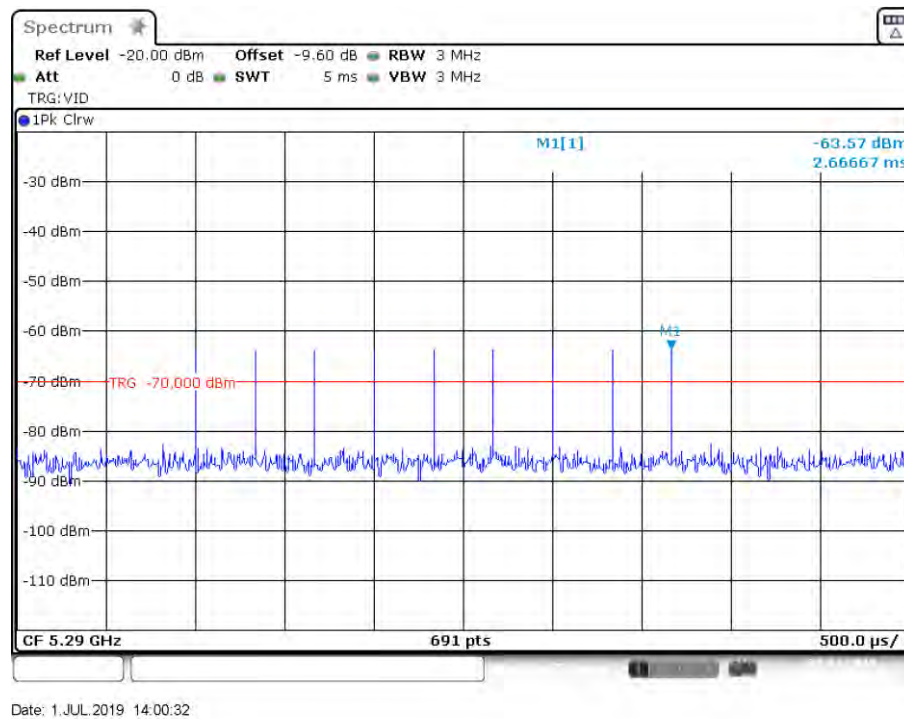
Figure 22: Radar Type 6 DFS Detection Threshold Level at 5290 MHz
