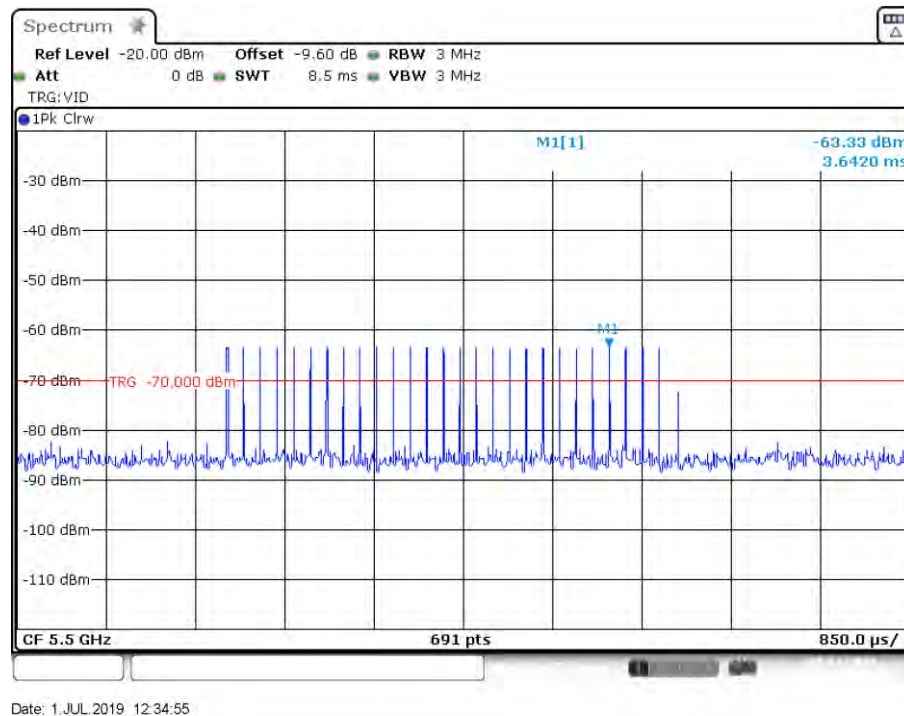
Figure 11: Radar Type 2 DFS Detection Threshold Level at 5500 MHz
