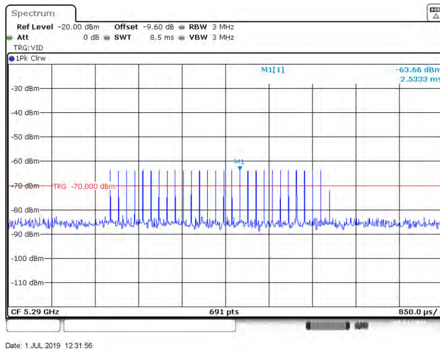
Figure 10: Radar Type 2 DFS Detection Threshold Level at 5290 MHz
