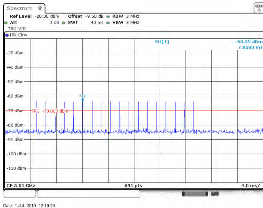
Figure 3: Radar Type 0 DFS Detection Threshold Level at 5510 MHz
