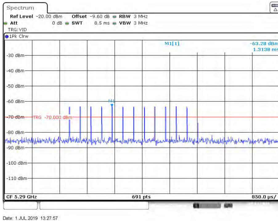
Figure 16: Radar Type 4 DFS Detection Threshold Level at 5290 MHz
