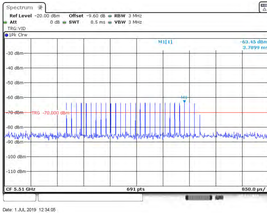
Figure 12: Radar Type 2 DFS Detection Threshold Level at 5510 MHz
