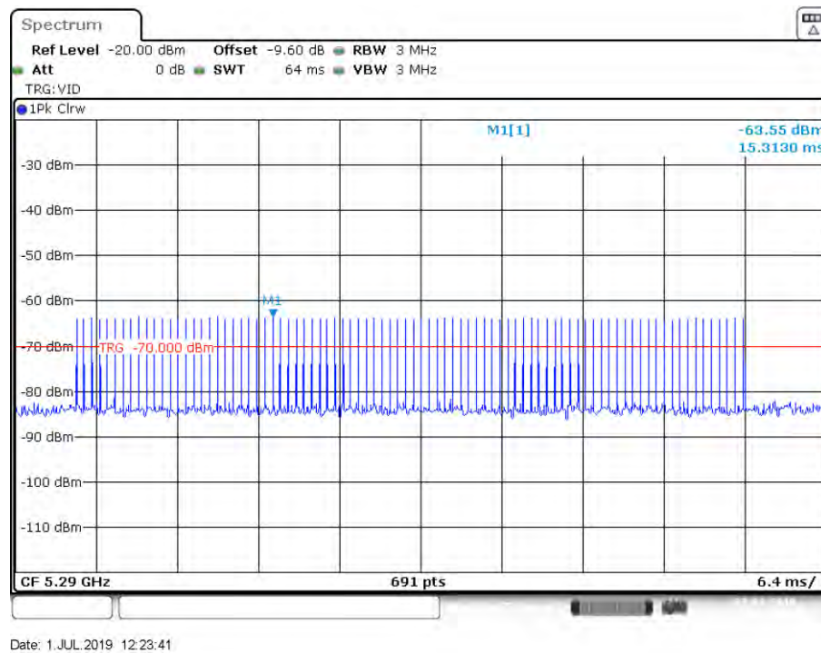
Figure 4: Radar Type 1A DFS Detection Threshold Level at 5290 MHz
