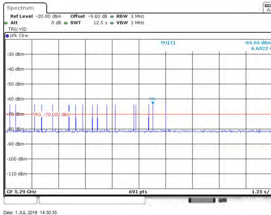
Figure 19: Radar Type 5 DFS Detection Threshold Level at 5290 MHz
