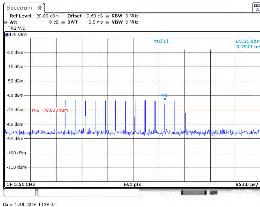
Figure 18: Radar Type 4 DFS Detection Threshold Level at 5510 MHz
