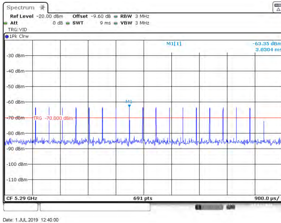
Figure 13: Radar Type 3 DFS Detection Threshold Level at 5290 MHz
