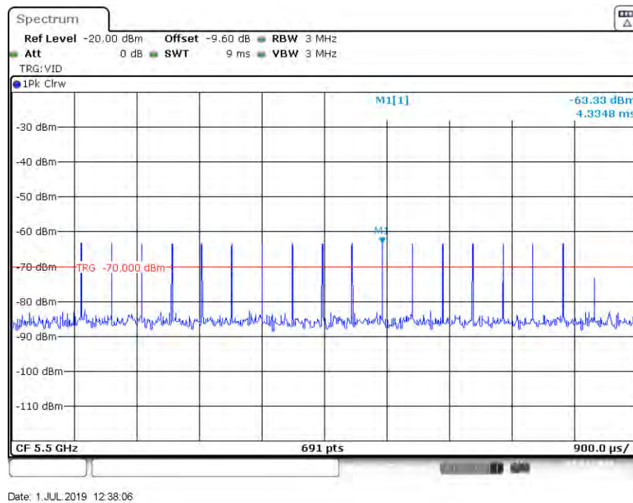
Figure 14: Radar Type 3 DFS Detection Threshold Level at 5500 MHz
