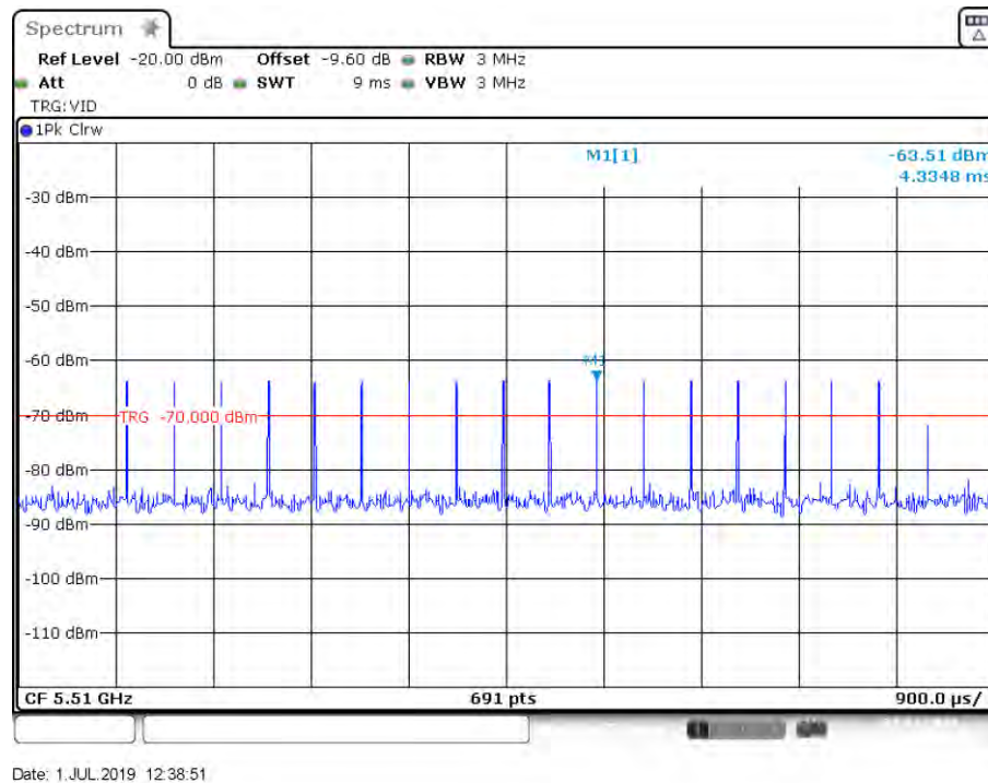
Figure 15: Radar Type 3 DFS Detection Threshold Level at 5510 MHz
