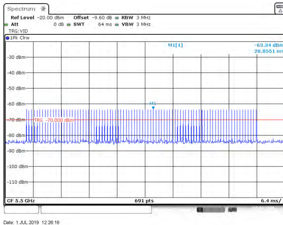
Figure 5: Radar Type 1A DFS Detection Threshold Level at 5500 MHz
