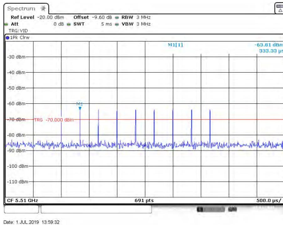
Figure 24: Radar Type 6 DFS Detection Threshold Level at 5510 MHz
