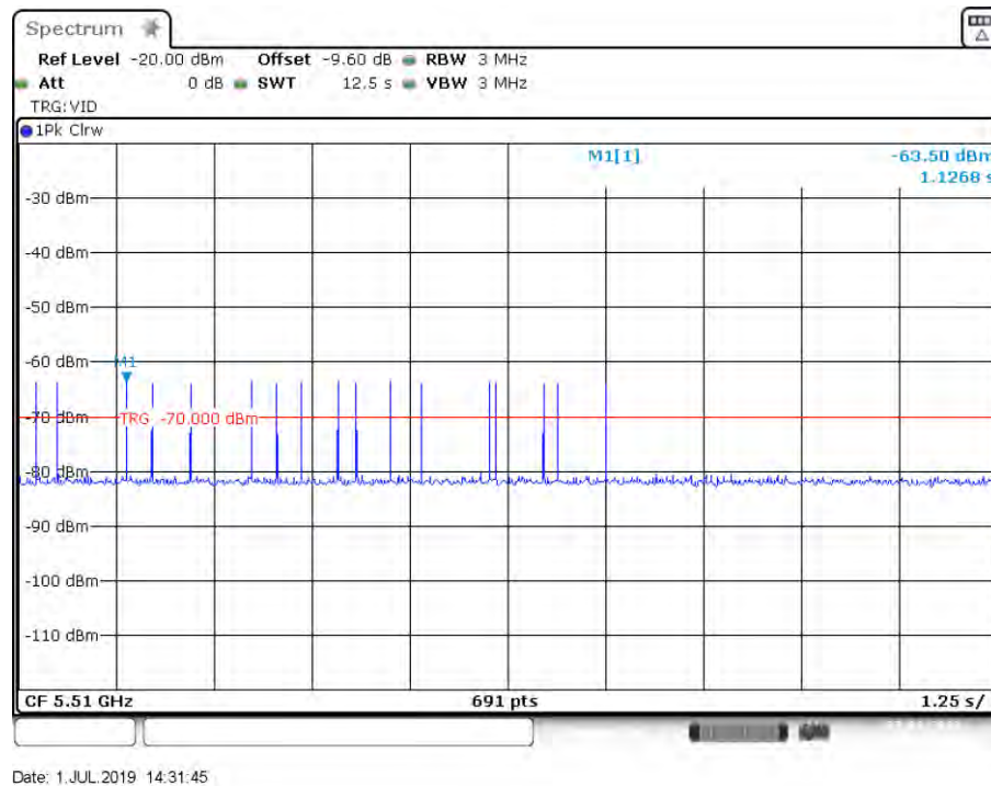
Figure 21: Radar Type 5 DFS Detection Threshold Level at 5510 MHz
