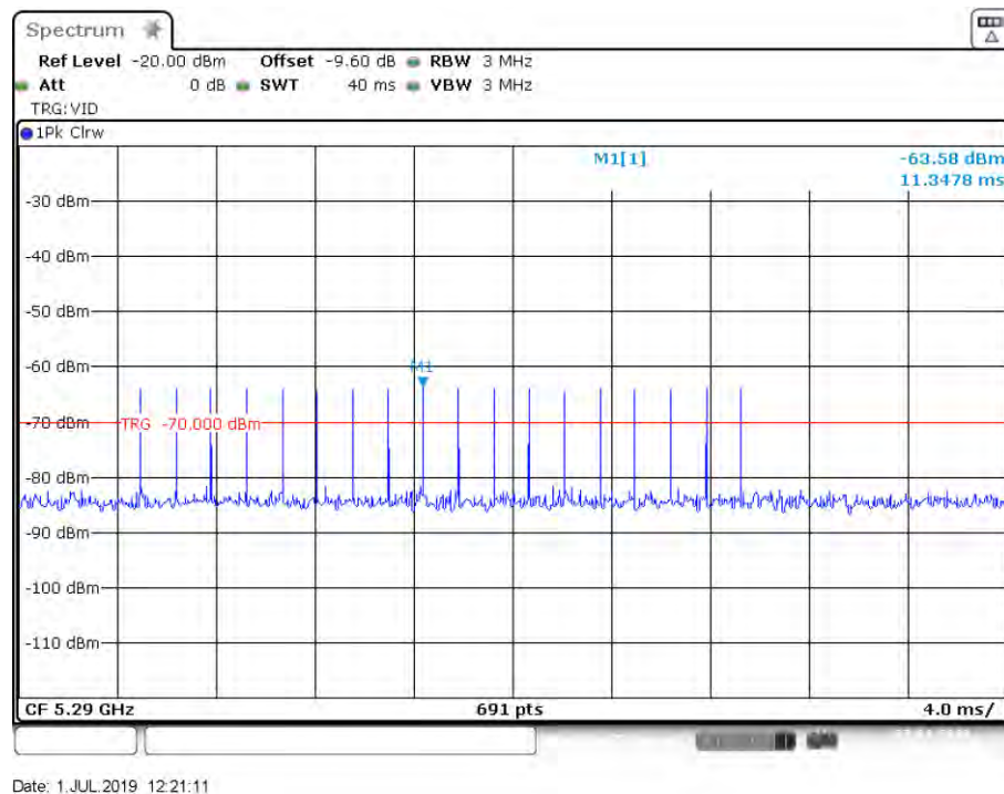
Figure 1: Radar Type 0 DFS Detection Threshold Level at 5290 MHz
