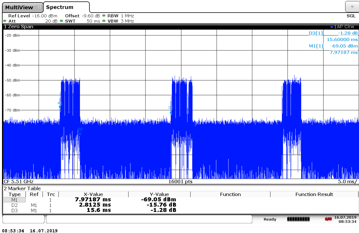
Figure 27: EUT Channel Loading at 5510 MHz (40 MHz bandwidth)
