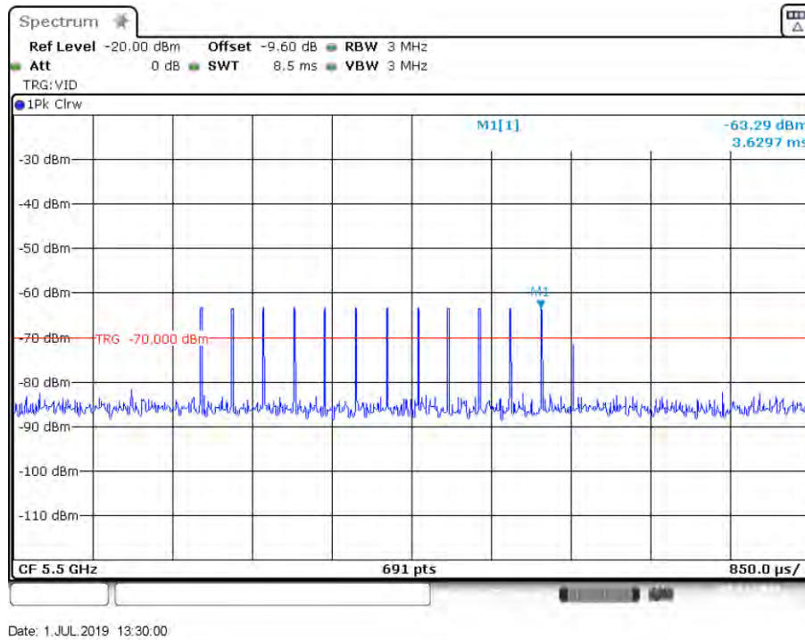
Figure 17: Radar Type 4 DFS Detection Threshold Level at 5500 MHz
