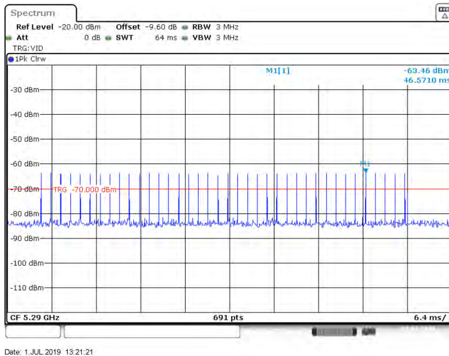
Figure 7: Radar Type 1B DFS Detection Threshold Level at 5290 MHz
