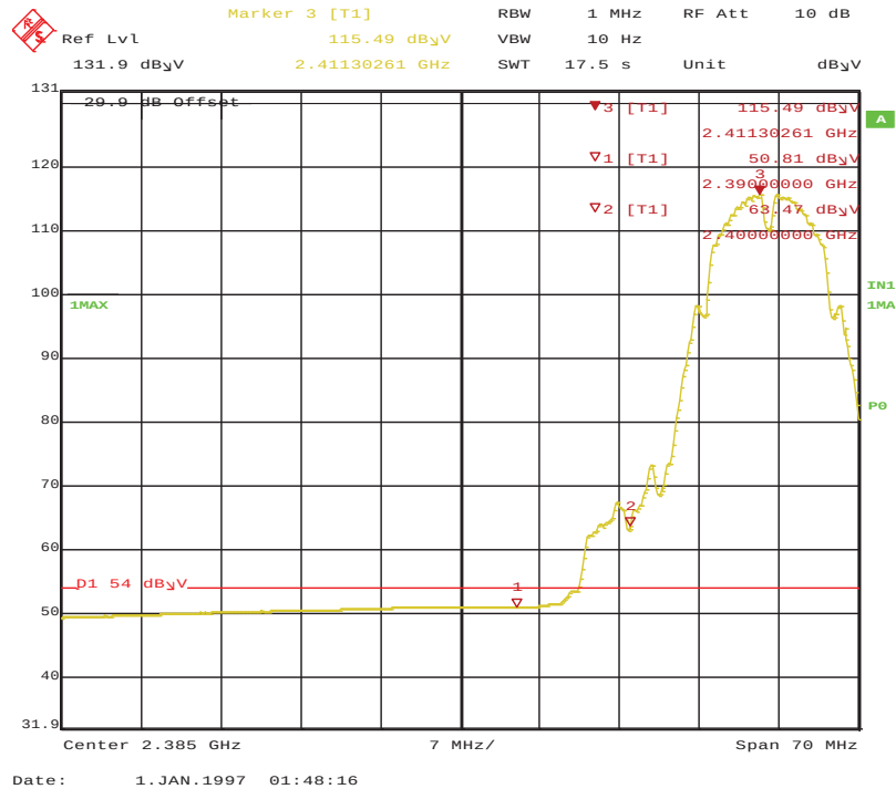
Figure 214: 11b Radiated Emission at the Edge of 2390 MHz Vert-Ave
