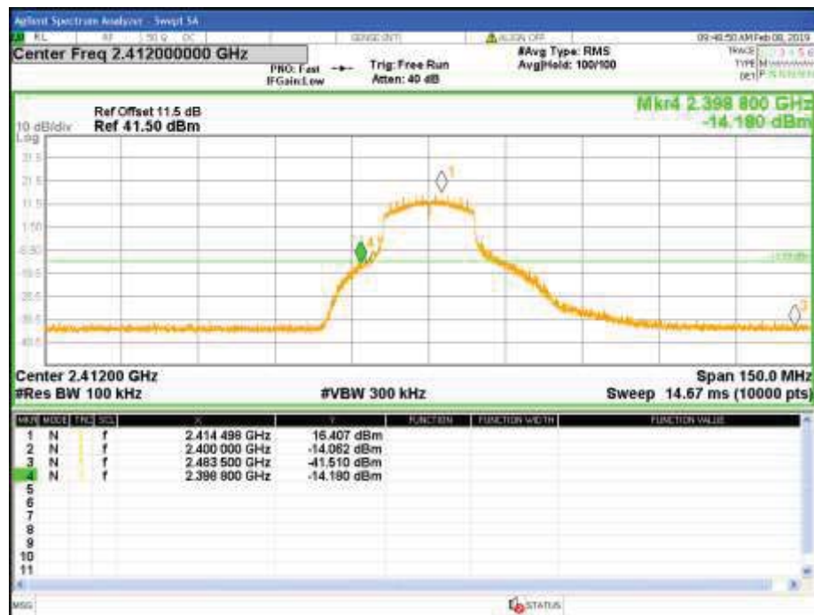
Figure 195: Measured Bandedge at 2400MHz-2412MHz-HT20-1x4- Ch1
