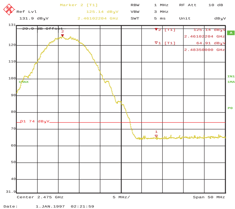
Figure 215: 11b Radiated Emission at the Edge of 2483.5 MHz Horz-Pk
