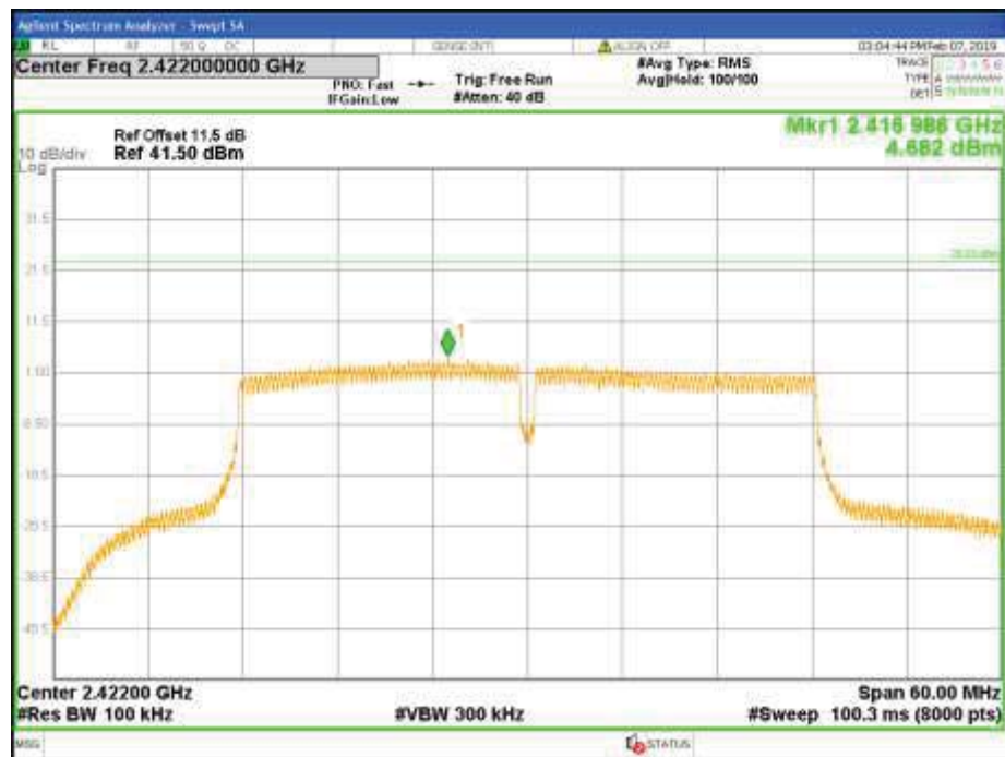
Figure 182: FCC-PPSD-2422MHz-HT40-1x4-q104-Ch2
