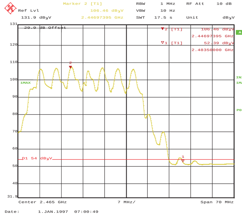
Figure 232: HT40 Radiated Emission at the Edge of 2483.5 MHz Horz-Ave
