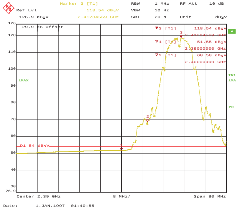
Figure 212: 11b Radiated Emission at the Edge of 2390 MHz Horz-Ave
