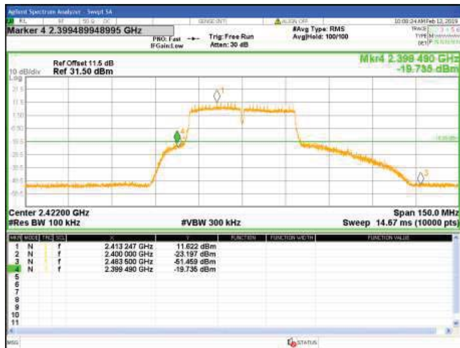
Figure 199: Measured Bandedge at 2400MHz-2422MHz-HT40-1x4-Ch1
