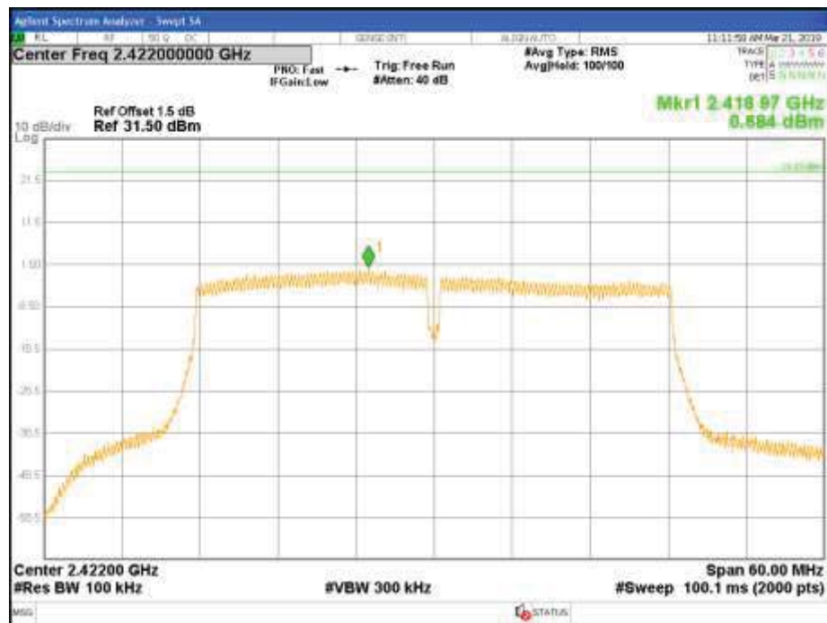
Figure 186: FCC-PPSD-2422MHz-HT40-4x4-q88-Ch2
