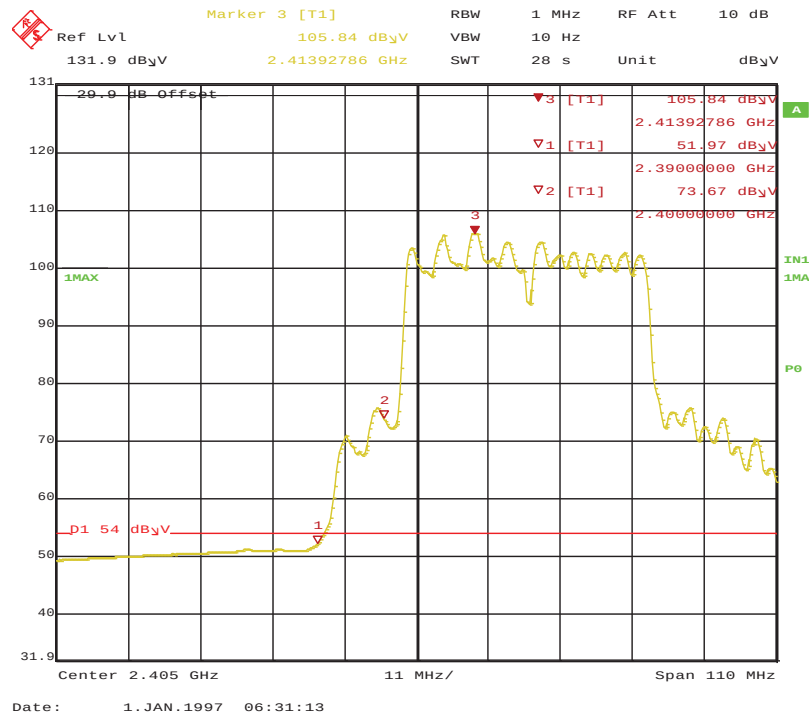
Figure 230: HT40 Radiated Emission at the Edge of 2390 MHz Horz-Ave
