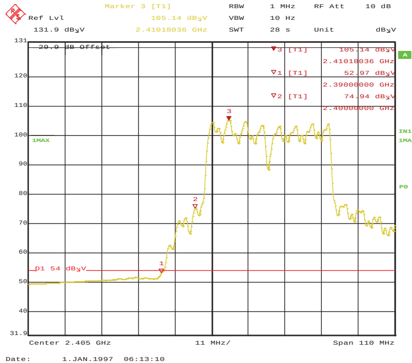
Figure 228: HT40 Radiated Emission at the Edge of 2390 MHz Vert-Ave
