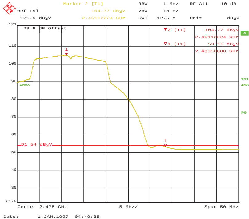
Figure 226: 11g Radiated Emission at the Edge of 2483.5 MHz Vert-Ave
