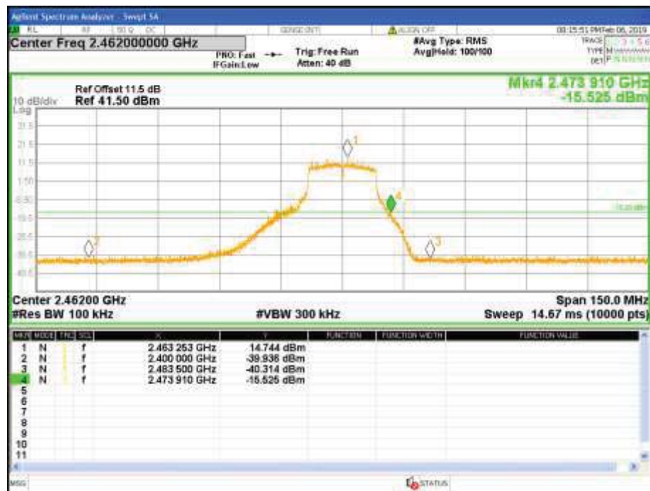
Figure 193: Measured Bandedge at 2483.5MHz-2462MHz-11g-1x4-Ch0
