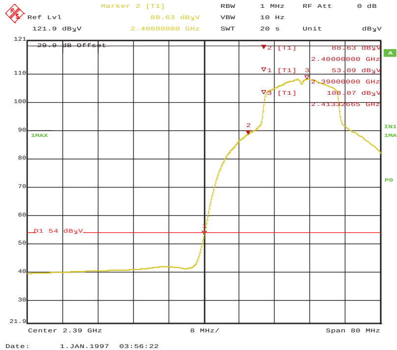
Figure 222: 11g Radiated Emission at the Edge of 2390 MHz Horz-Ave
