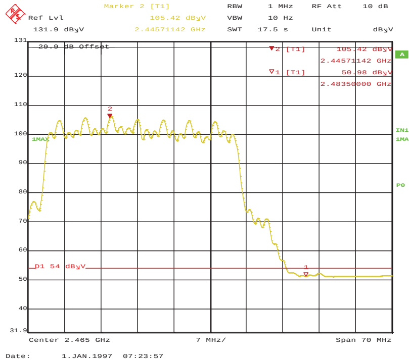
Figure 234: HT40 Radiated Emission at the Edge of 2483.5 MHz Vert-Ave
