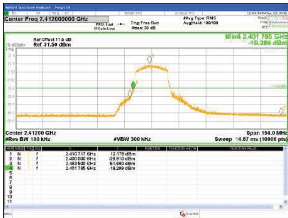
Figure 203: Measured Bandedge at 2400MHz-2412MHz-HT20-4x4-Ch1
