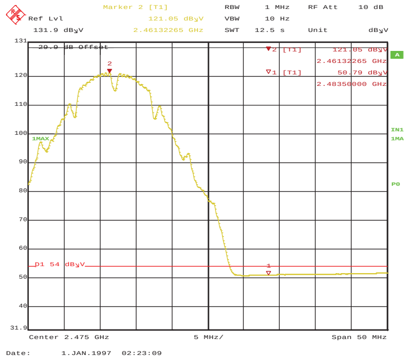
Figure 216: 11b Radiated Emission at the Edge of 2483.5 MHz Horz-Ave
