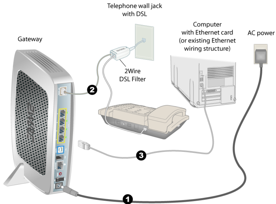
Figure 1. Gateway Connected Via Ethernet
