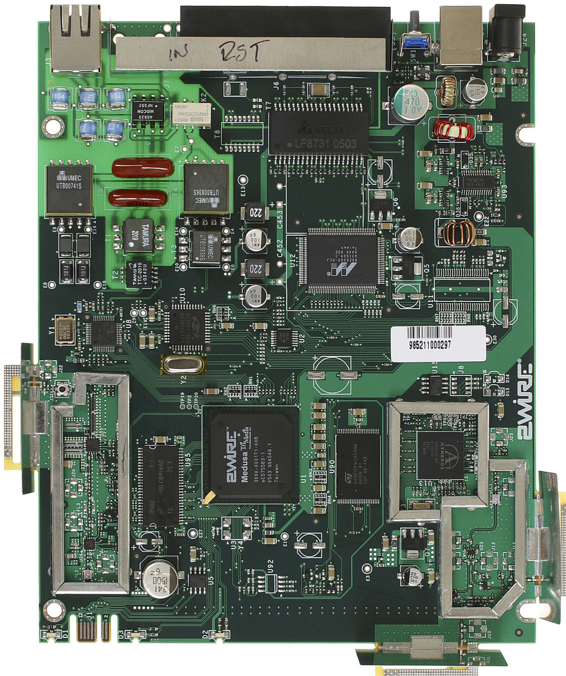
Fig. 5 Printed Circuit Board, Top, w/o Covers
