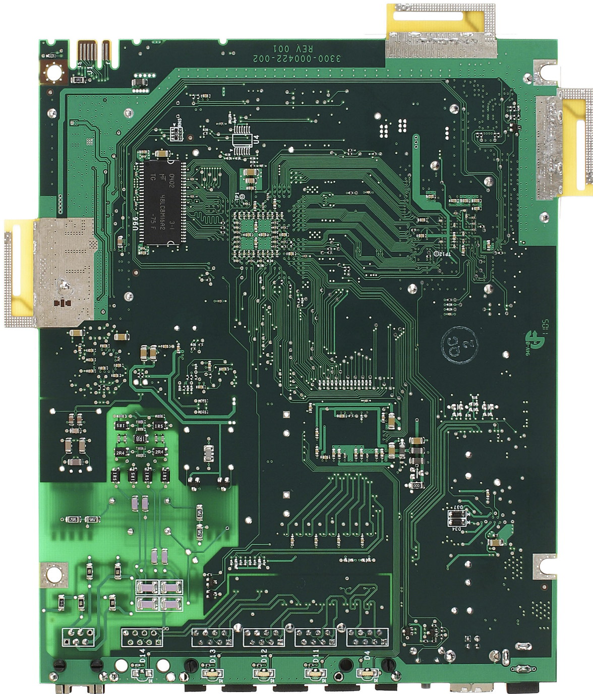
Fig. 6 Printed Circuit Board, Bottom
