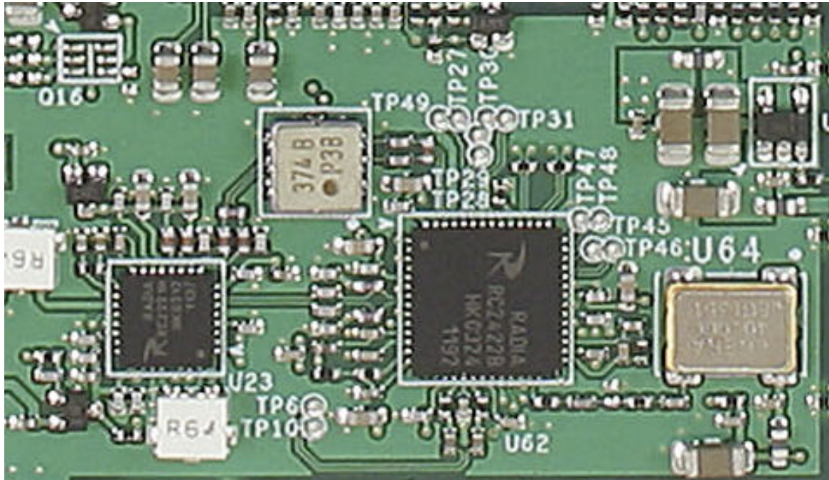
802.11b/g RF Transceiver Circuit Portion
