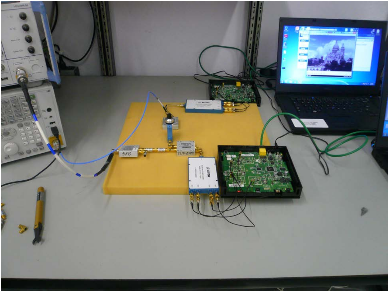
Figure 18: DFS Test Setup Photo for Slave Mode – Close-up
