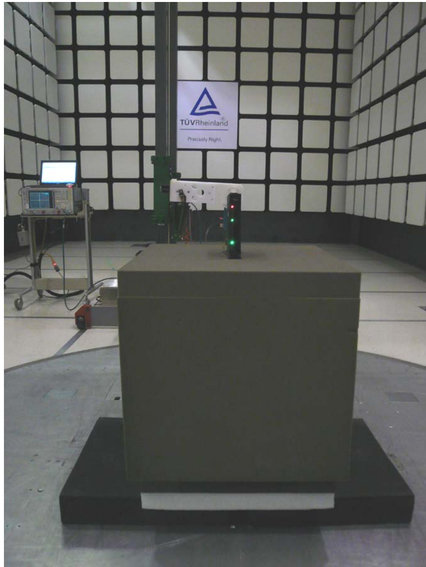
Figure 5: Test Setup for 18 GHz to 26GHz (Front View) – Y-Axis
