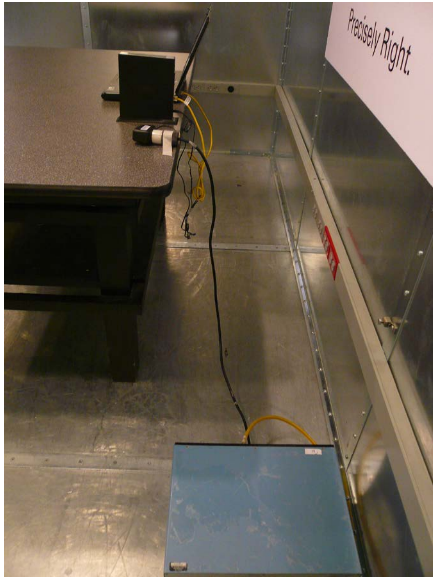
Figure 15: AC Conducted Emission Test Setup (Side View)
