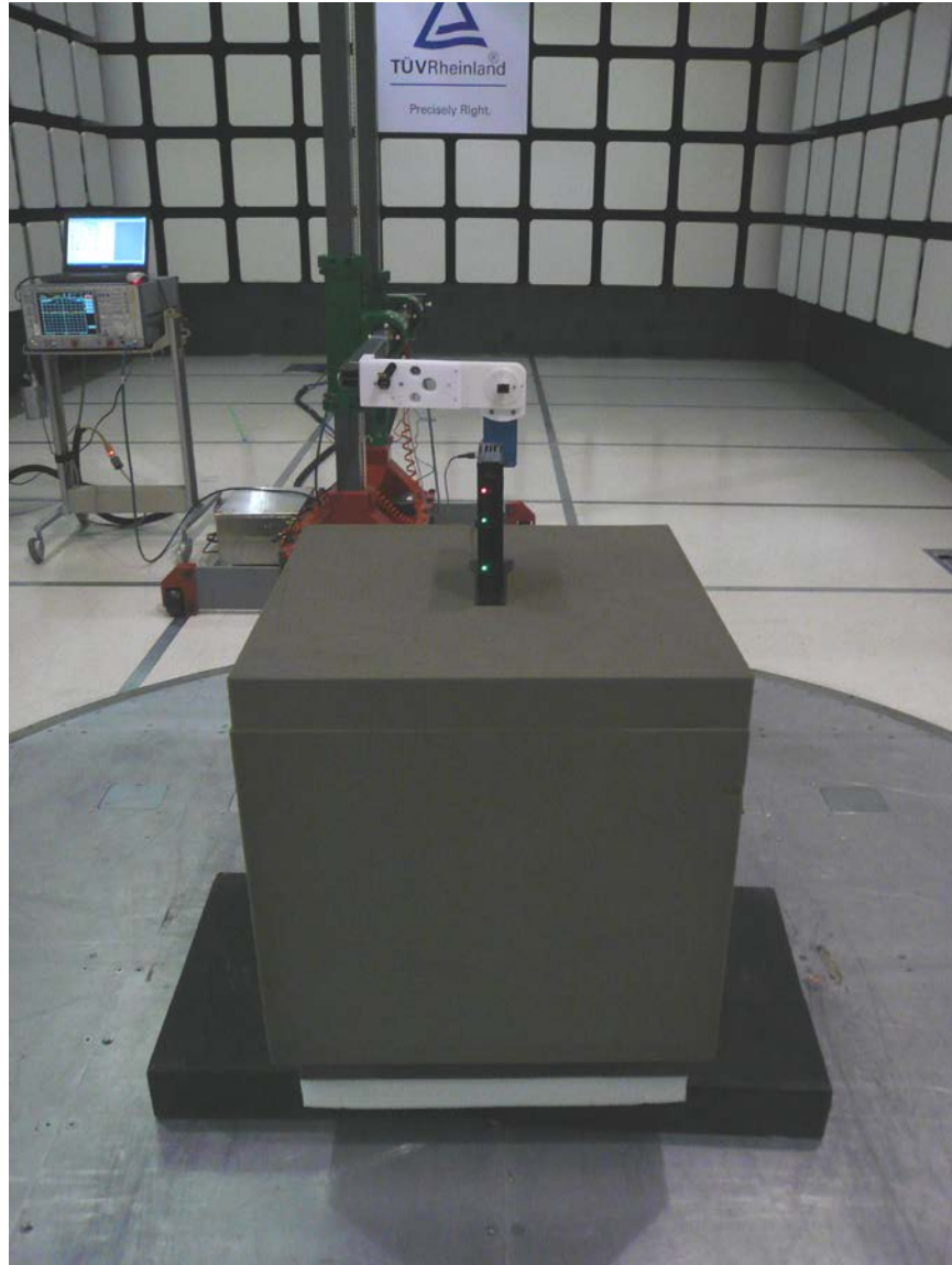
Figure 7: Test Setup for 26 GHz to 40GHz (Front View) - Y-Axis
