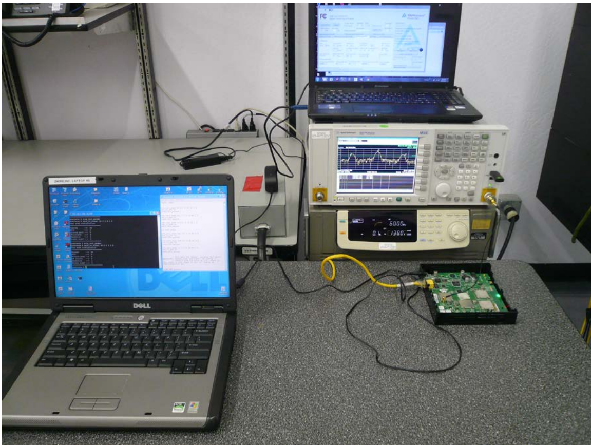
Figure 13: Voltage Variation Test Setup
