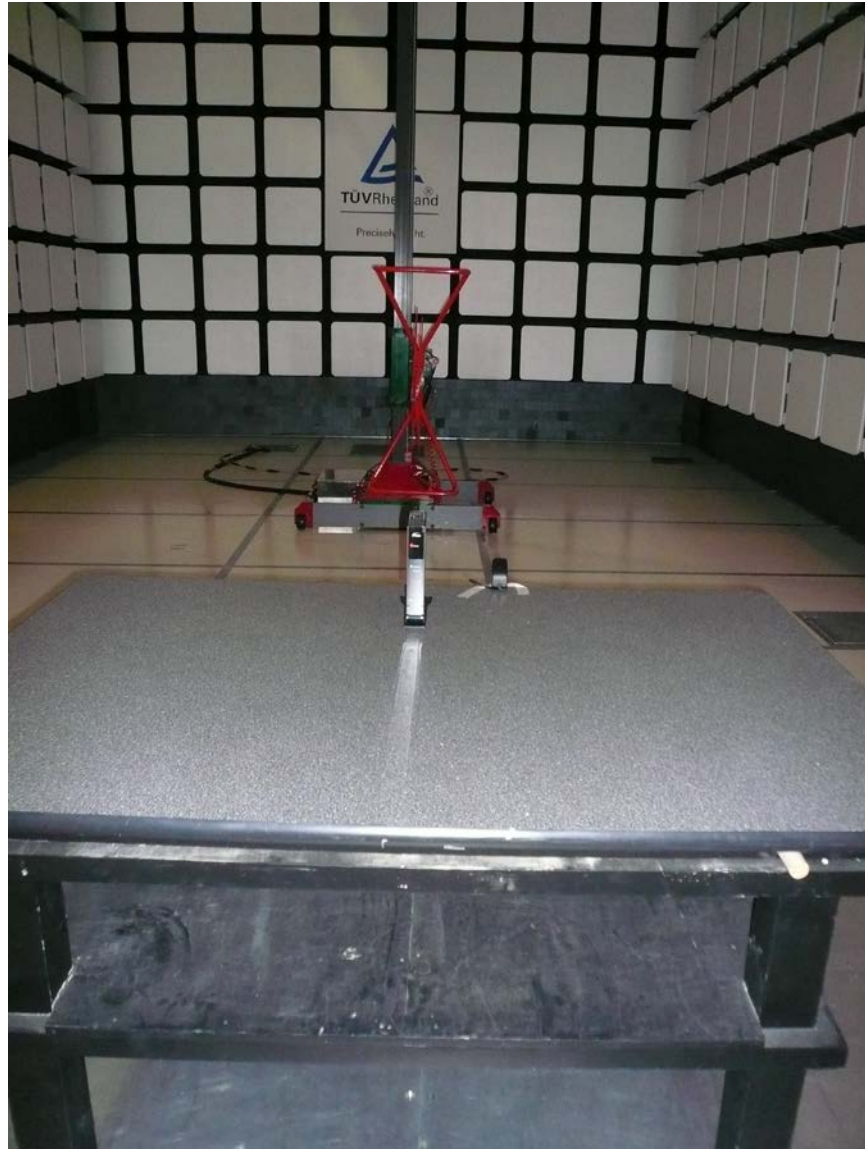
Figure 1: Test Setup for 30 MHz to 1000MHz (Front View) – Y-Axis
