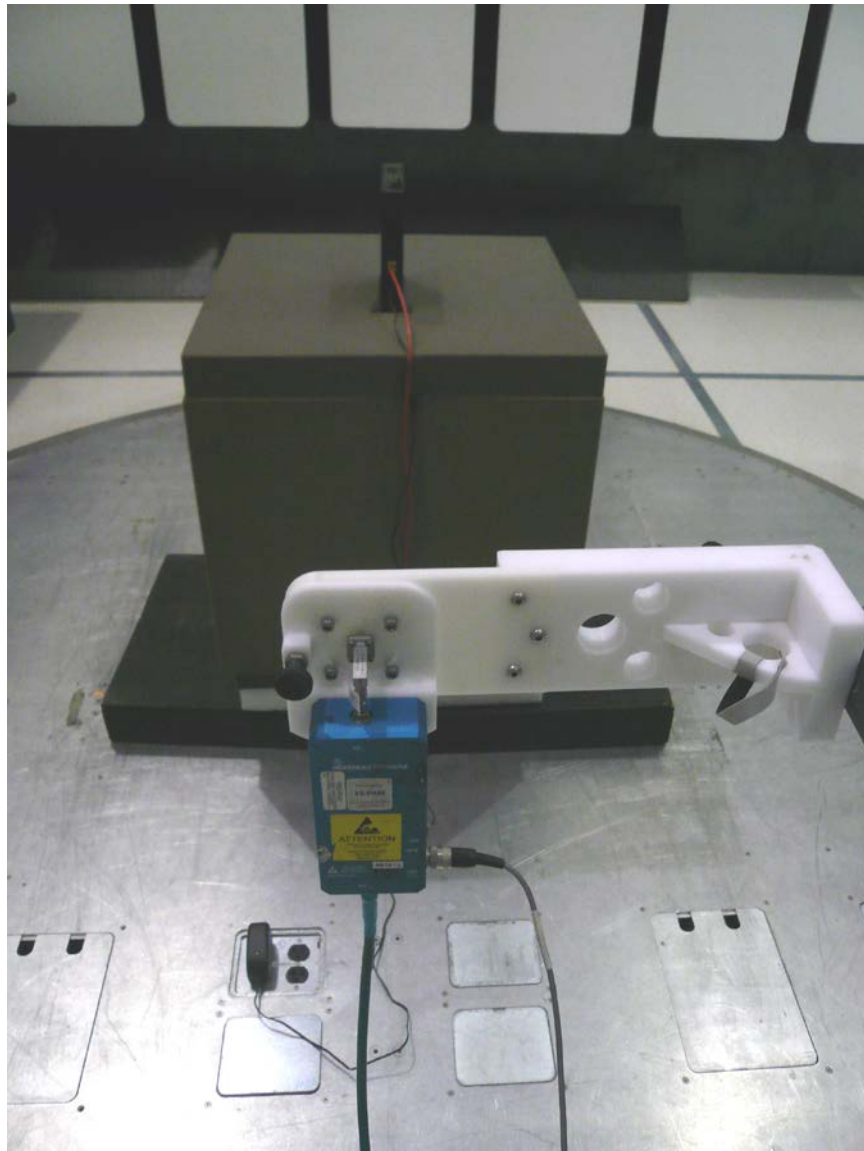
Figure 8: Test Setup for 26 GHz to 40GHz (Rear View) - Y-Axis
