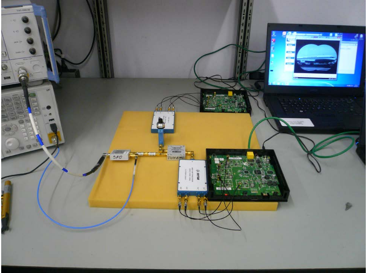
Figure 17: DFS Test Setup Photo for Master Mode – Close-up
