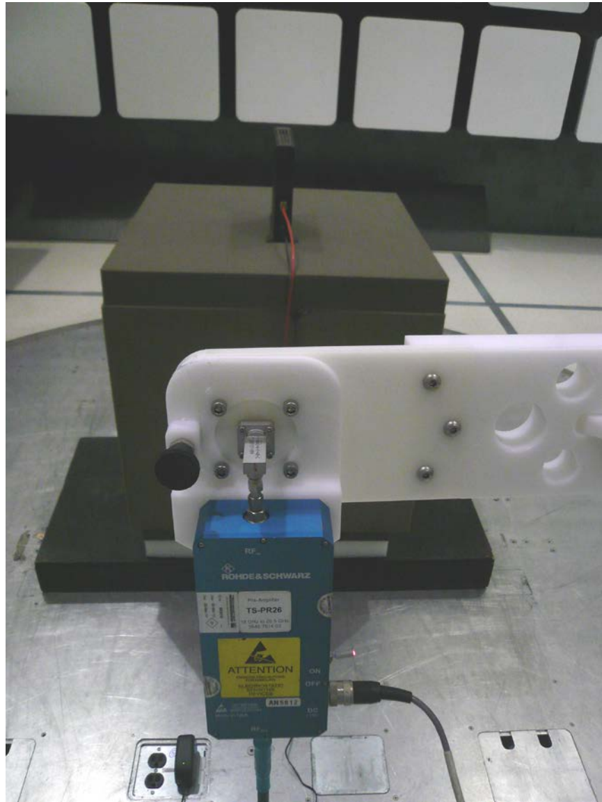
Figure 6: Test Setup for 18 GHz to 26GHz (Rear View) - Y-Axis
