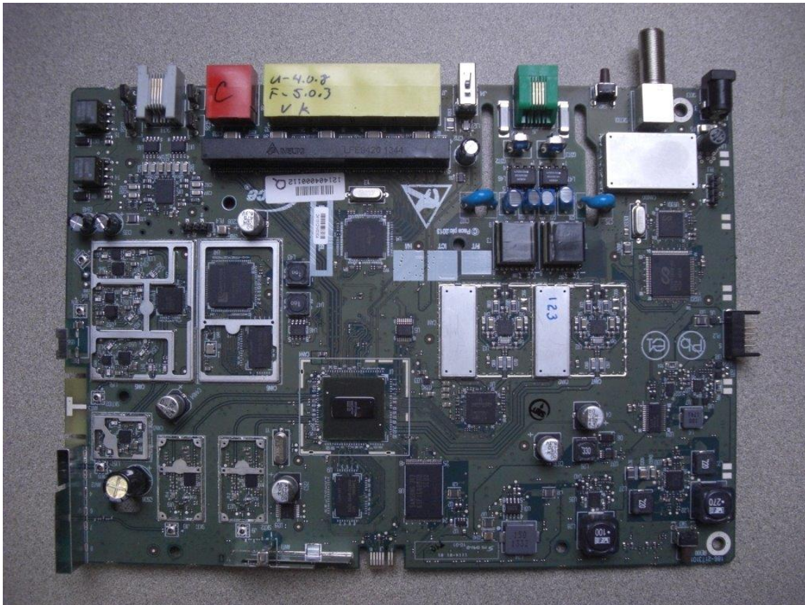
Figure 3: Photo without RF Shielding
