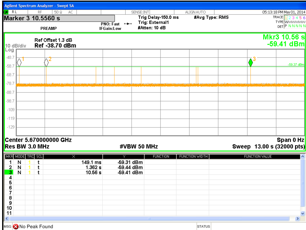
Figure 14: Long Pulse Radar Type at 5670 MHz (11-20 \mu s Pulse Width, 200-500 \mu s PRI, 8-20 Bursts)
