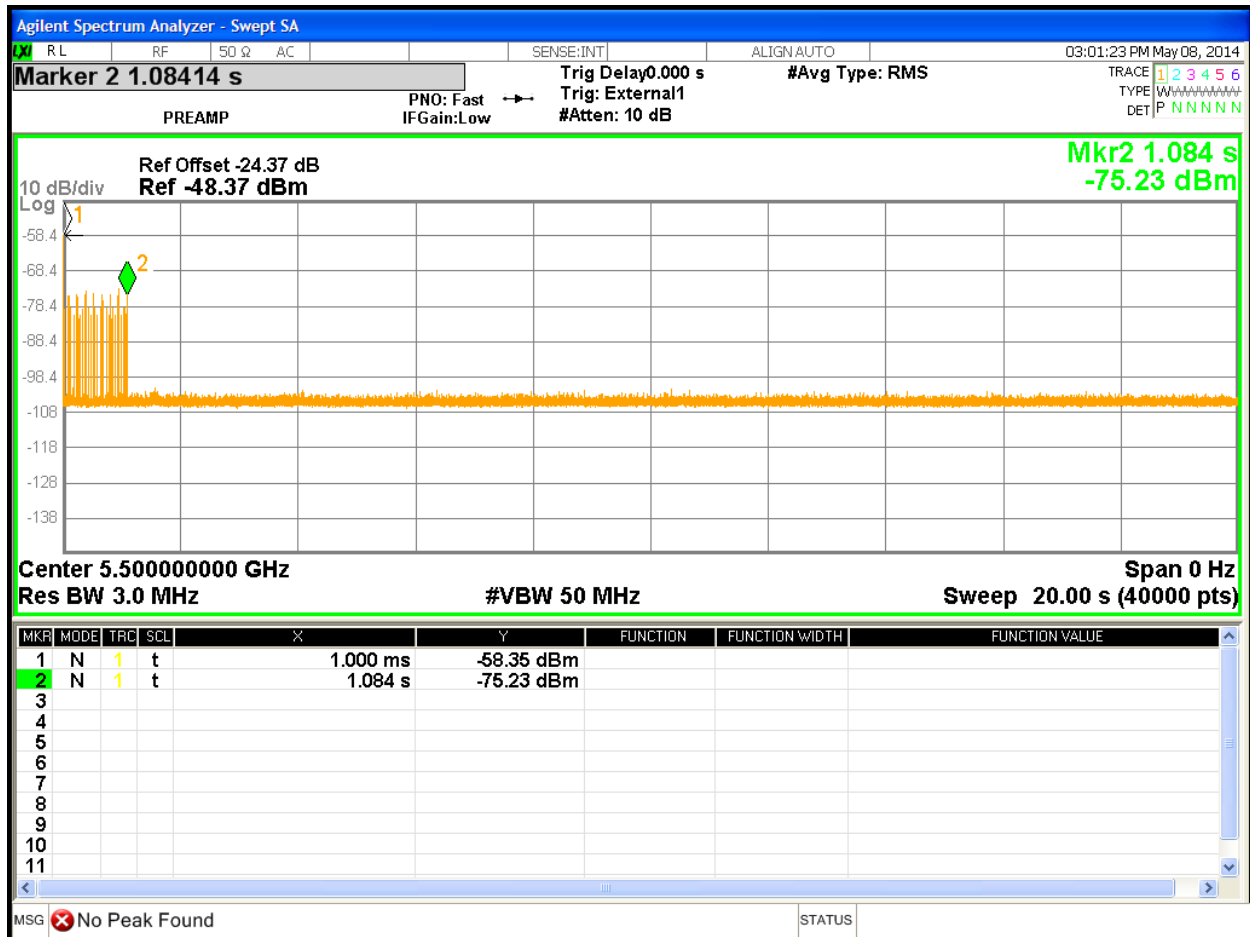
Figure 33: Channel Move Time and Channel Closing Transmission Time using Long Pulse Radar Waveform 5 in Master Mode for 20 MHz Bandwidth
