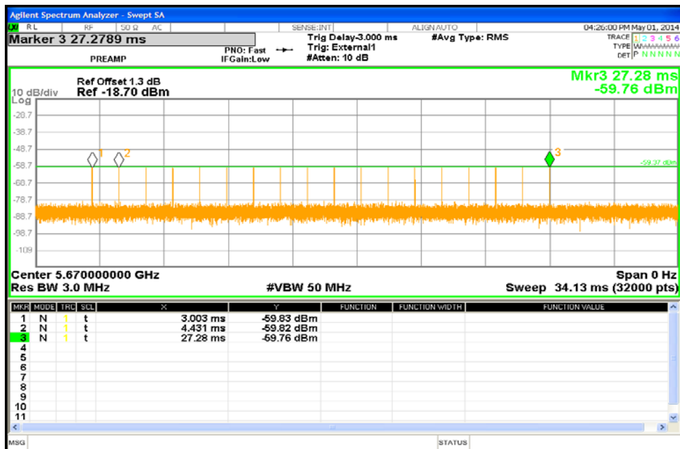
Figure 2: Short Pulse Radar Type 1 at 5670 MHz (1μS Pulse Width, 1428μS PRI, 18 Pulses)
