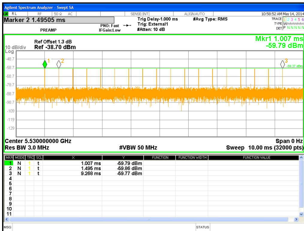
Figure 9: Short Pulse Radar Type 3 at 5530 MHz (6-10 \mu S Pulse Width, 200-500 \mu S PRI, 16-18 Pulses)
