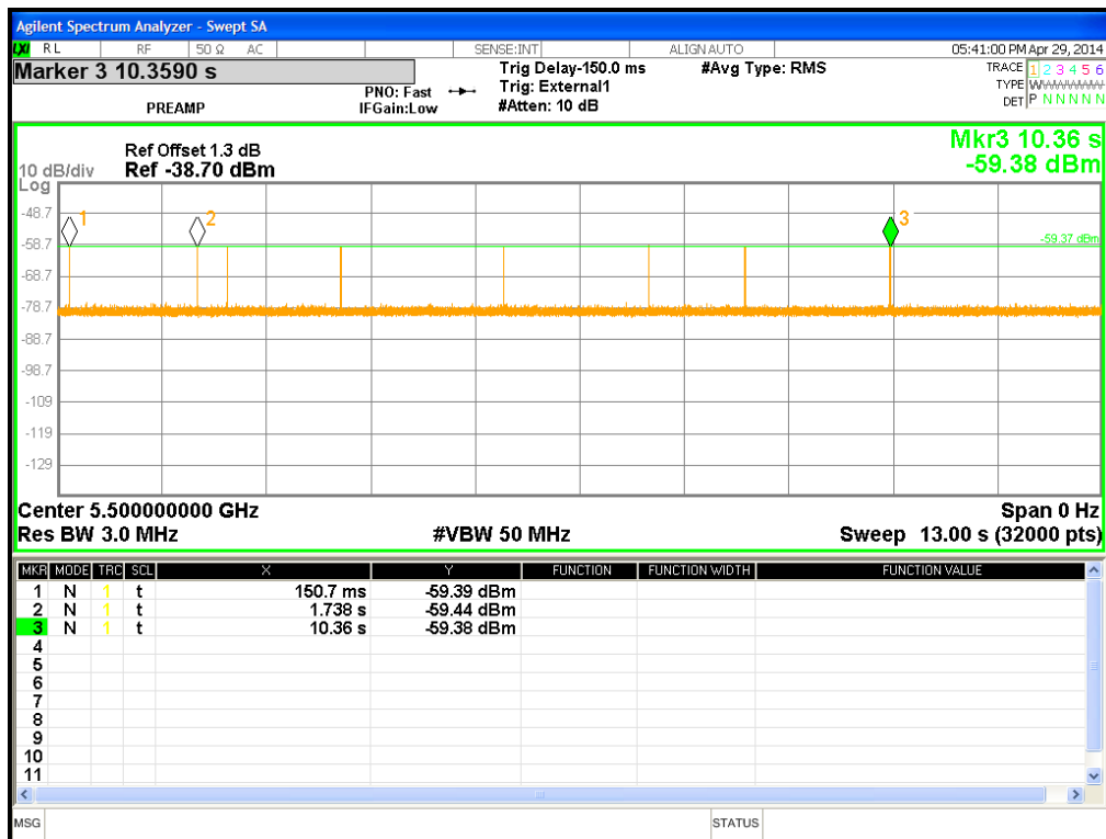
Figure 13: Long Pulse Radar Type 5at 5500MHz (11-20 \mu s Pulse Width, 200-500 \mu s PRI, 8-20 Bursts)
