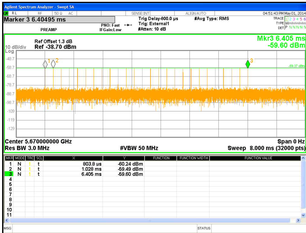
Figure 5: Short Pulse Radar Type 2 at 5670 MHz (1-5 \mu s Pulse Width, 150-230 \mu s PRI, 23-29 Pulses)
