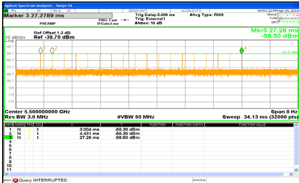
Figure 1: Short Pulse Radar Type 1 at 5500MHz (1μS Pulse Width, 1428μS PRI, 18 Pulses)
