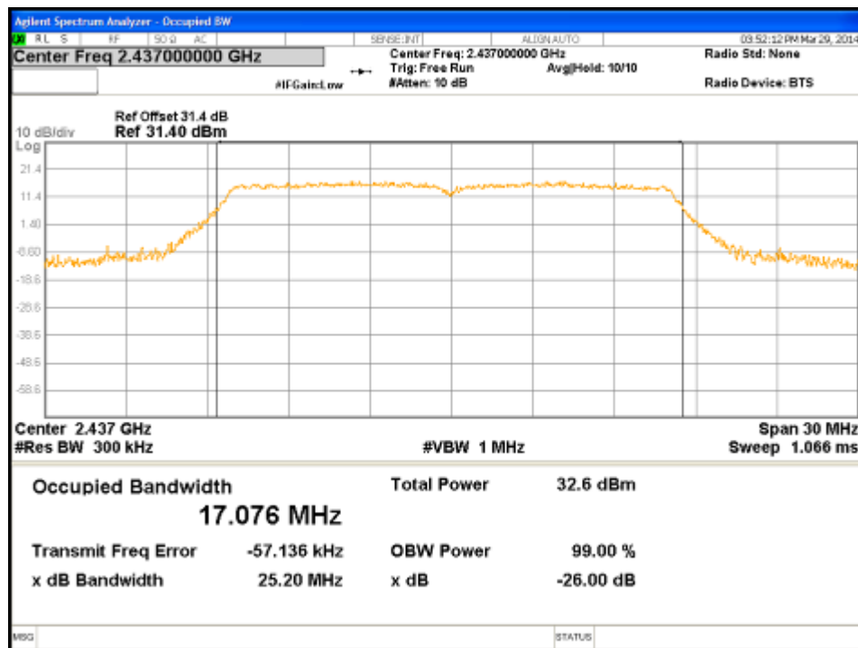
Figure 35: 99% Bandwidth-802.11g-2437 MHz-Ch0
