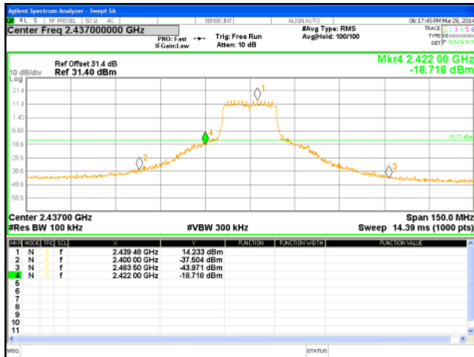
Figure 63: Conducted Band Edge-2437 MHz-HT20-MCS0-Ch0
