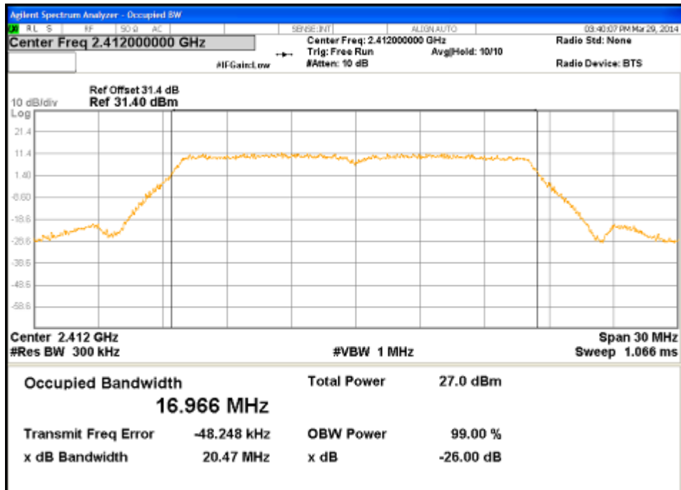
Figure 34: 99% Bandwidth-802.11g-2412 MHz-Ch0
