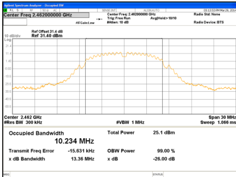
Figure 30: 99% Bandwidth-802.11b-2462 MHz-Ch0
