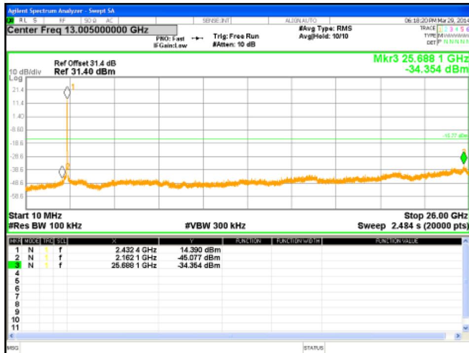
Figure 64: Out of band Emission-2437 MHz-HT20-MCS0-Ch0
