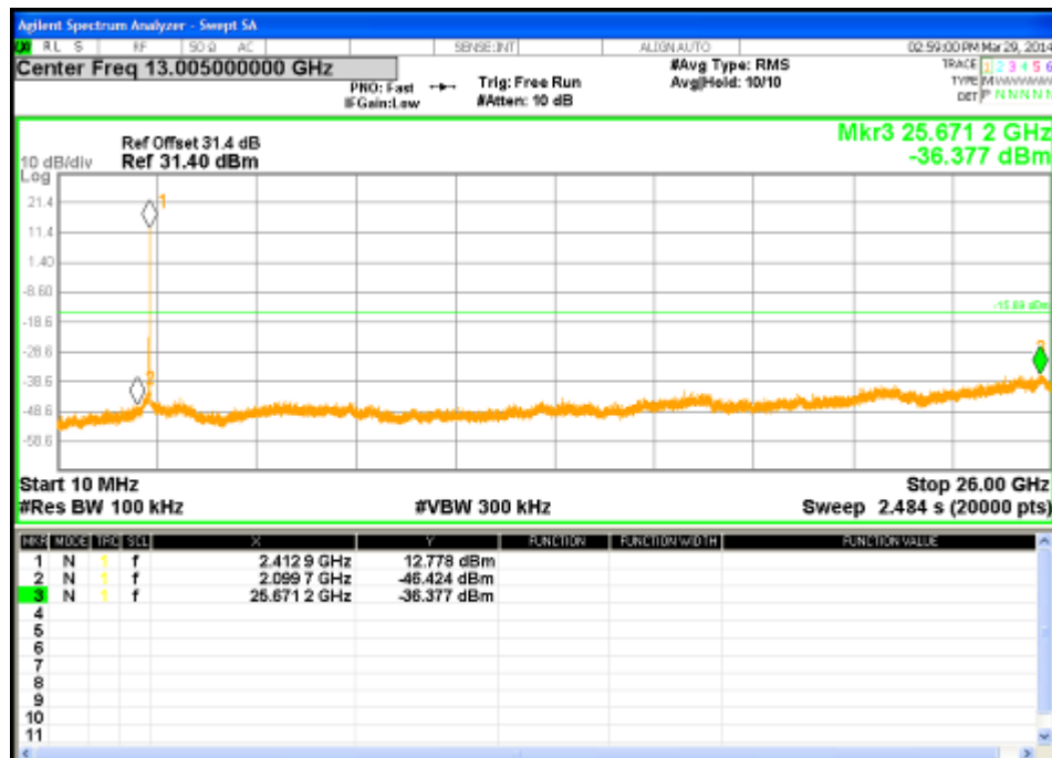
Figure 50: Out of band Emission-2412 MHz-11b-1Mbps-Ch0
