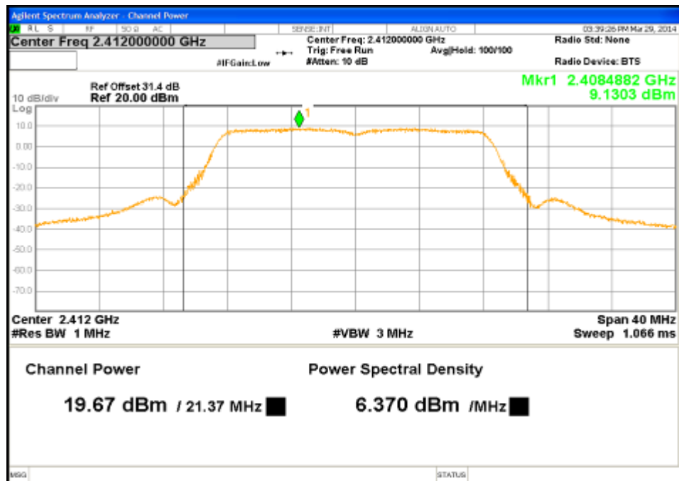
Figure 4: Maximum Conducted Output Power-2412 MHz-11g-6Mbps-Ch0
