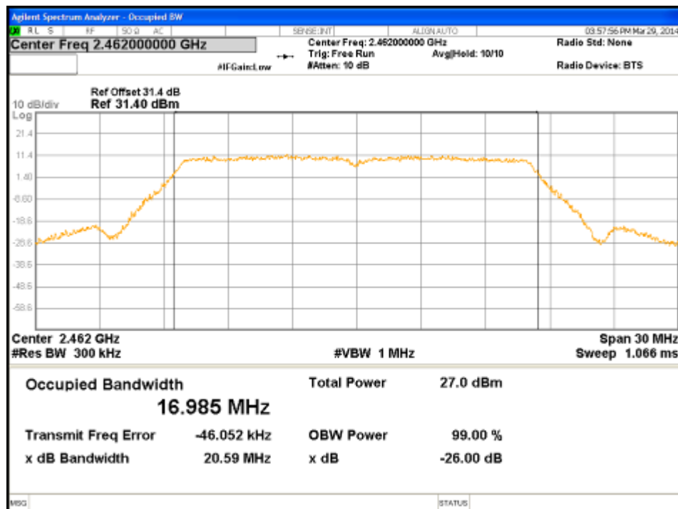
Figure 36: 99% Bandwidth-802.11g-2462 MHz-Ch0
