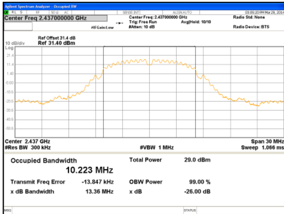
Figure 29: 99% Bandwidth-802.11b-2437 MHz-Ch0
