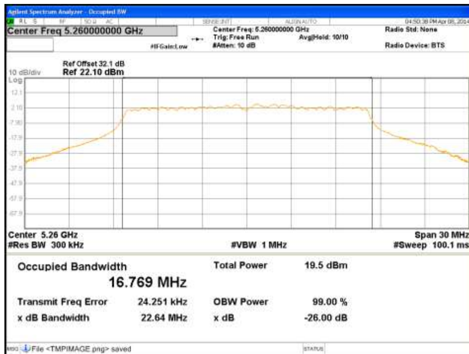
Figure 60: Occupied Bandwidth-5260MHz-11a-6Mbps-Ch3
