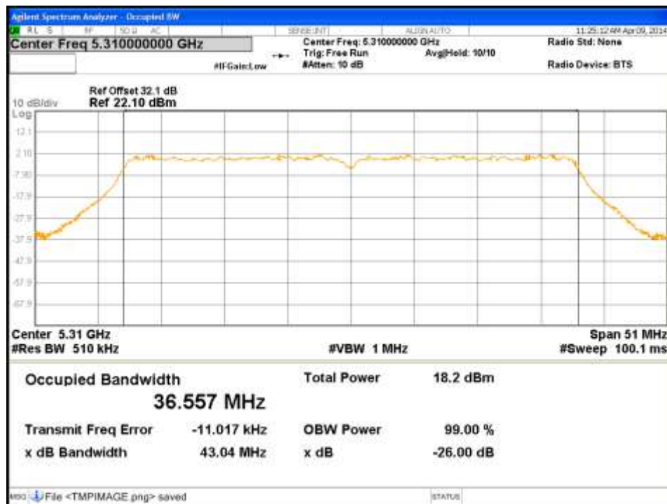
Figure 88: Occupied Bandwidth-5310MHz-HT40-MCS0-Ch3
