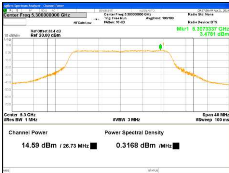
Figure 38: Maximum Conducted Output Power-5300MHz-VHT20-MCS0-Ch1
