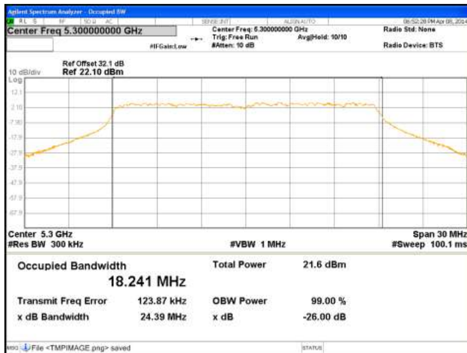
Figure 94: Occupied Bandwidth-5300MHz-VHT20-MCS0-Ch1
