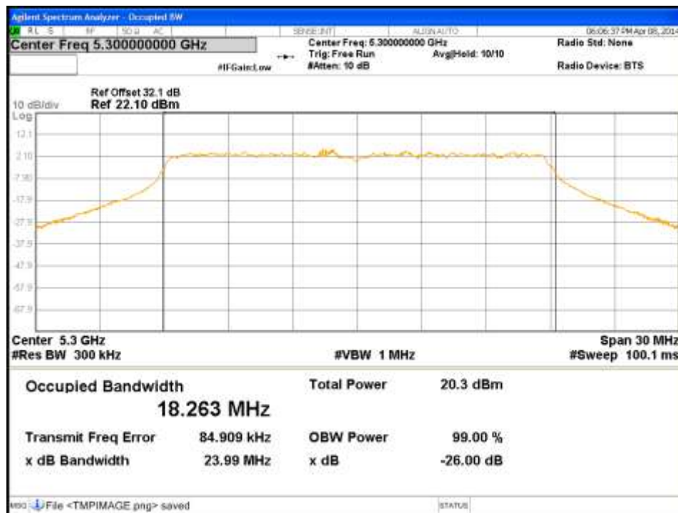
Figure 76: Occupied Bandwidth-5300MHz-HT20-MCS0-Ch3
