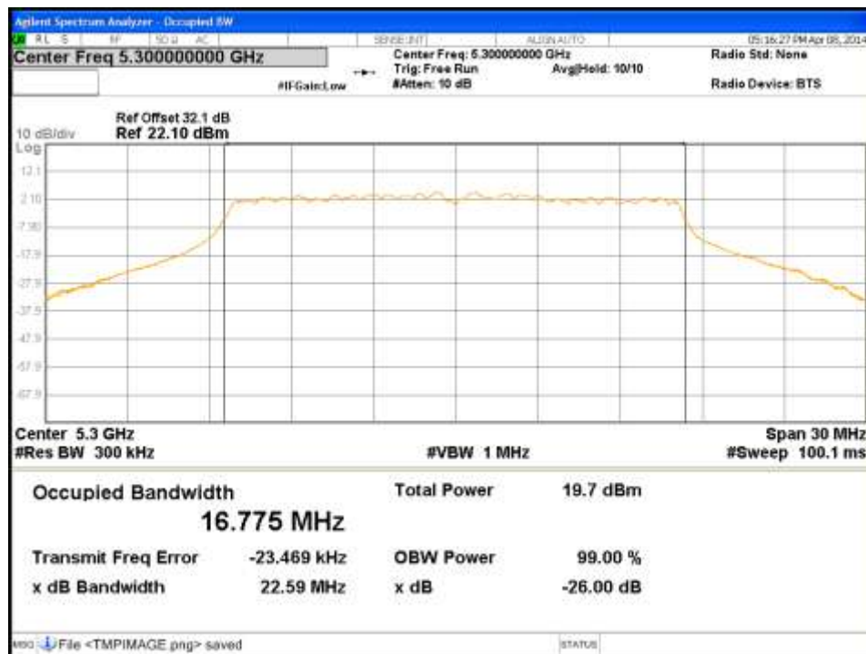
Figure 64: Occupied Bandwidth-5300MHz-11a-6Mbps-Ch3
