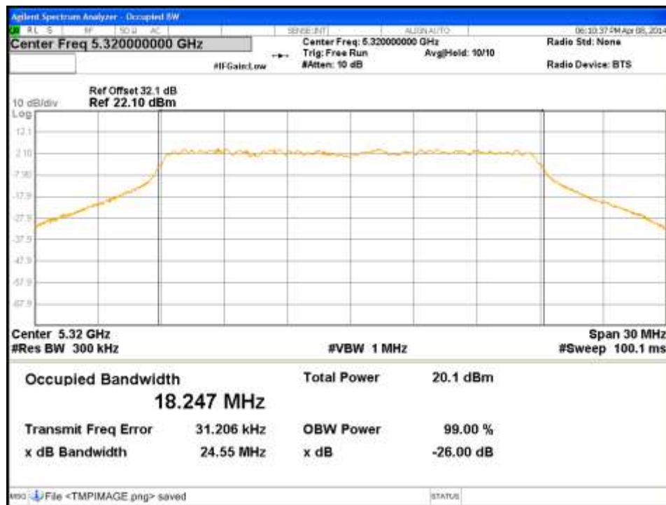
Figure 77: Occupied Bandwidth-5320MHz-HT20-MCS0-Ch0
