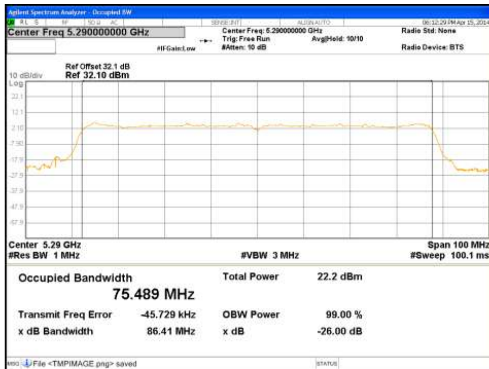
Figure 112: Occupied Bandwidth-5290MHz-VHT80-MCS0-Ch3
