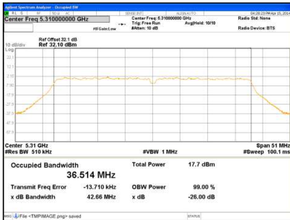
Figure 105: Occupied Bandwidth-5310MHz-VHT40-MCS0-Ch0
