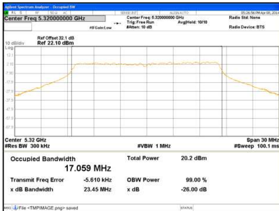
Figure 66: Occupied Bandwidth-5320MHz-11a-6Mbps-Ch1
