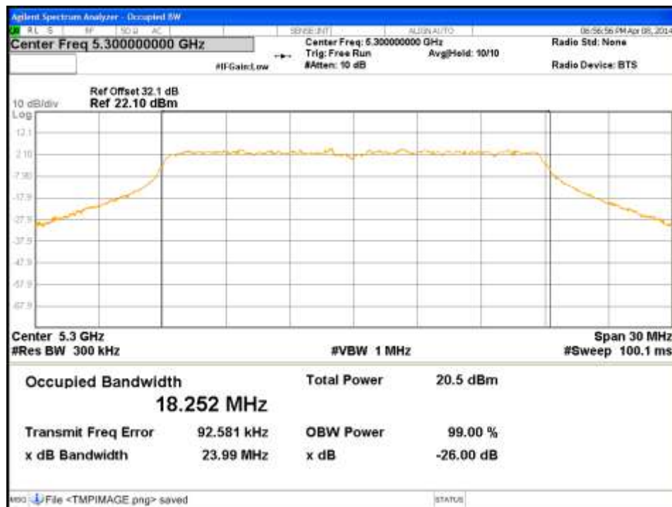
Figure 96: Occupied Bandwidth-5300MHz-VHT20-MCS0-Ch3
