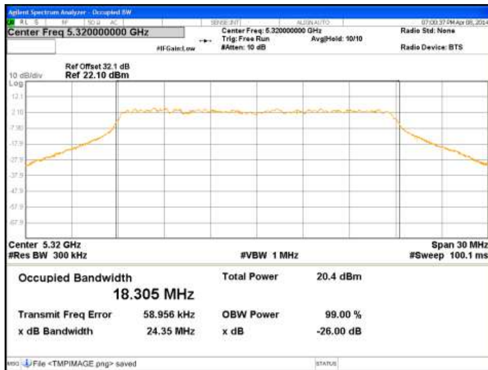
Figure 97: Occupied Bandwidth-5320MHz-VHT20-MCS0-Ch0
