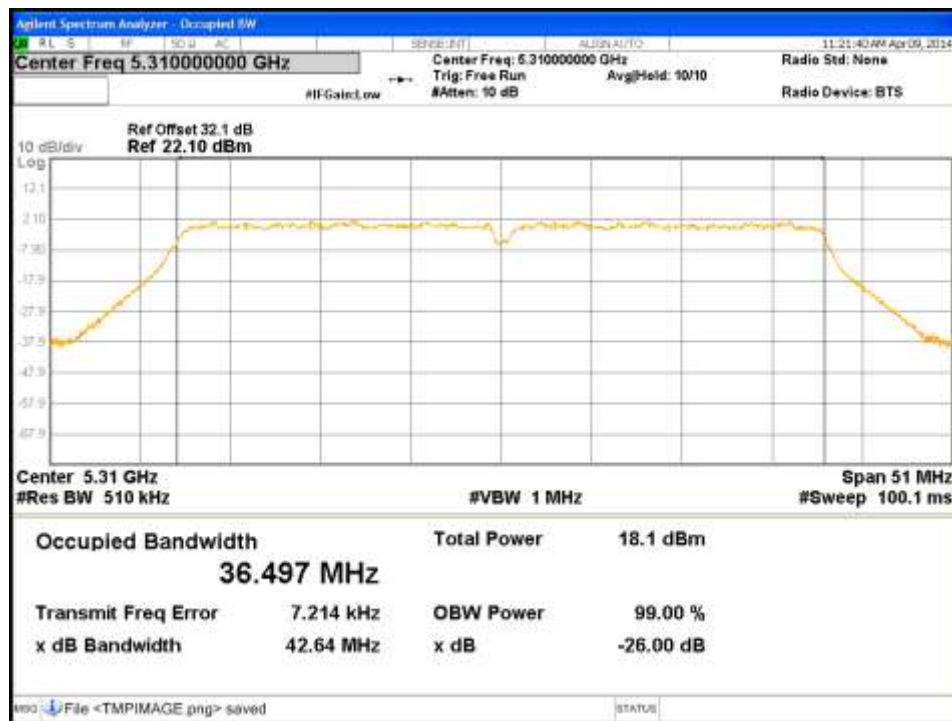
Figure 87: Occupied Bandwidth-5310MHz-HT40-MCS0-Ch2
