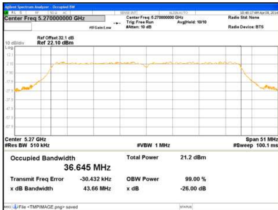
Figure 84: Occupied Bandwidth-5270MHz-HT40-MCS0-Ch3
