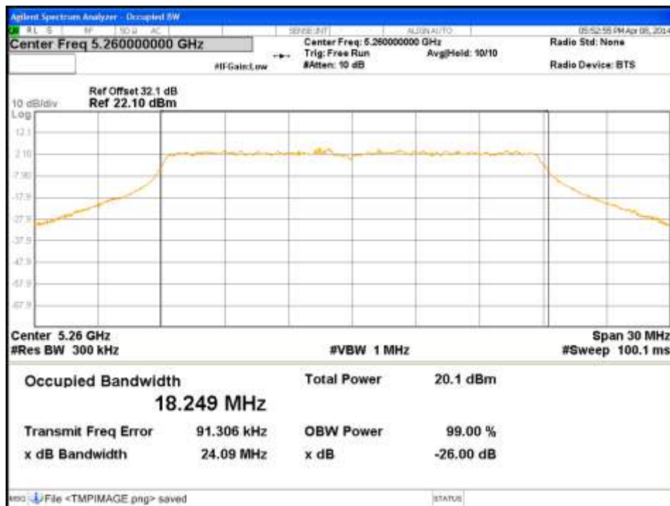
Figure 72: Occupied Bandwidth-5260MHz-HT20-MCS0-Ch3
