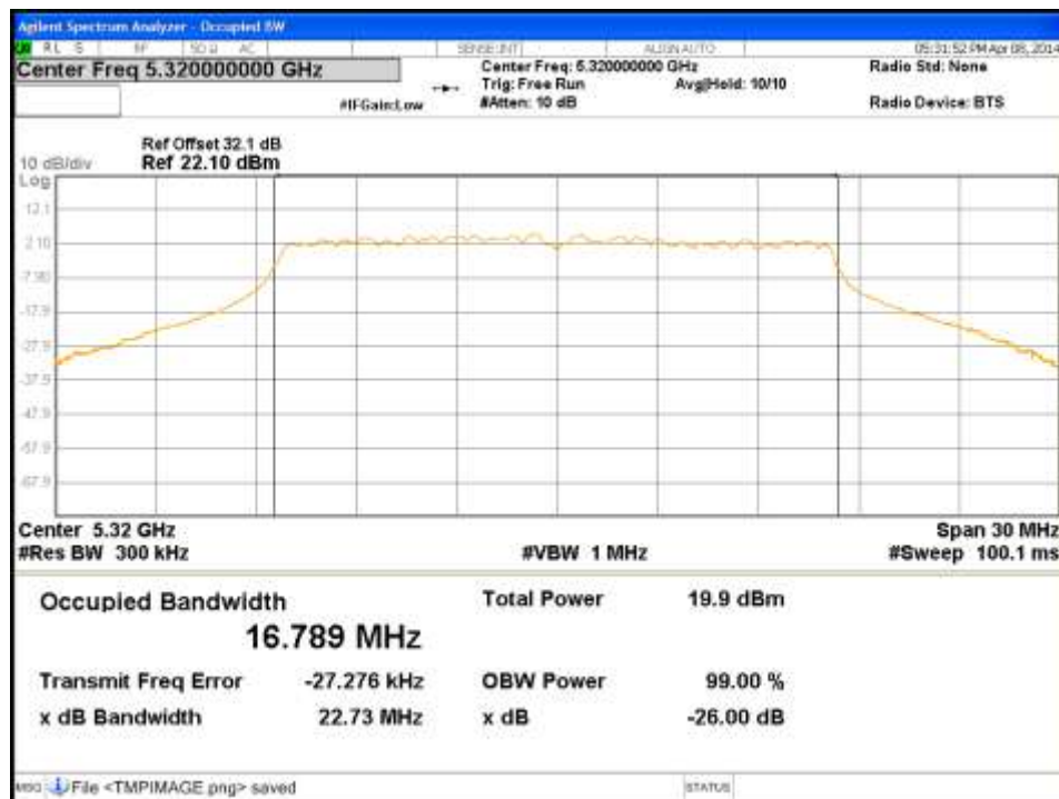
Figure 68: Occupied Bandwidth-5320MHz-11a-6Mbps-Ch3
