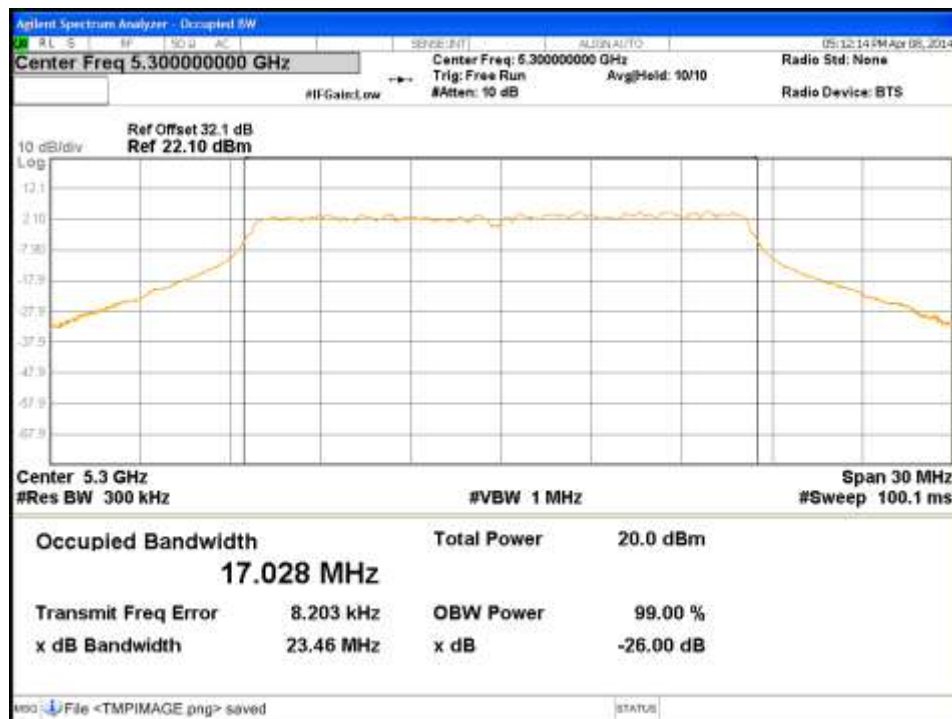
Figure 62: Occupied Bandwidth-5300MHz-11a-6Mbps-Ch1
