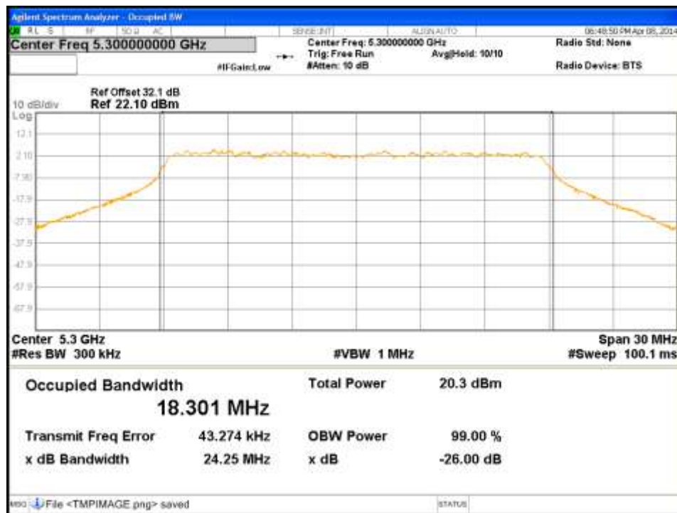
Figure 93: Occupied Bandwidth-5300MHz-VHT20-MCS0-Ch0
