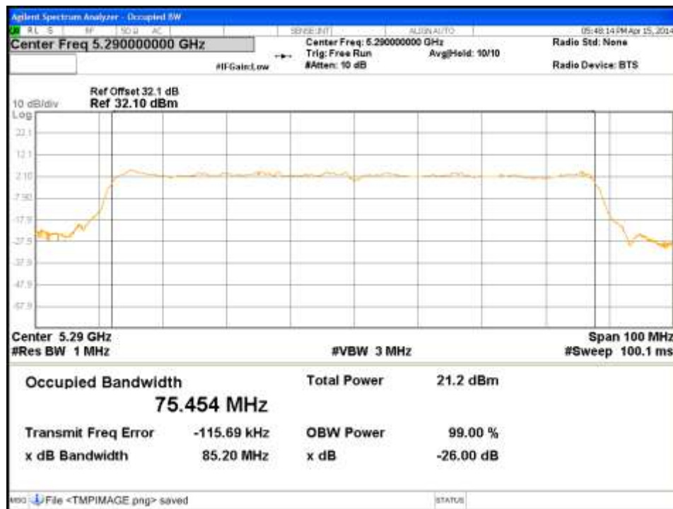
Figure 109: Occupied Bandwidth-5290MHz-VHT80-MCS0-Ch0
