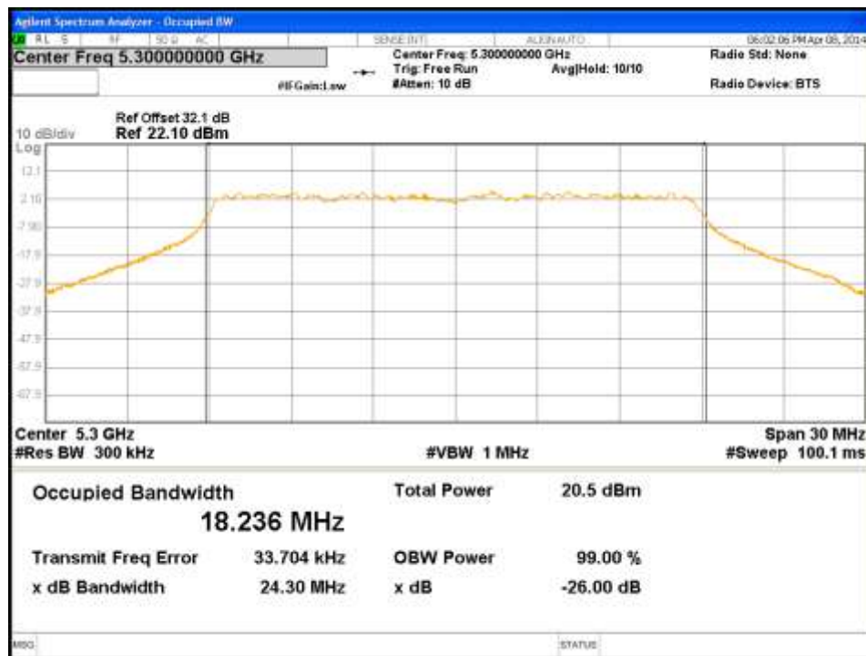
Figure 75: Occupied Bandwidth-5300MHz-HT20-MCS0-Ch2
