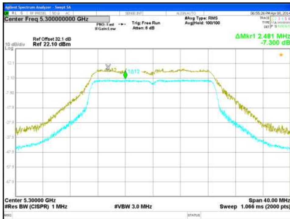
Figure 151: Peak Excursion-5300MHz-VHT20-MCS0-Ch2
