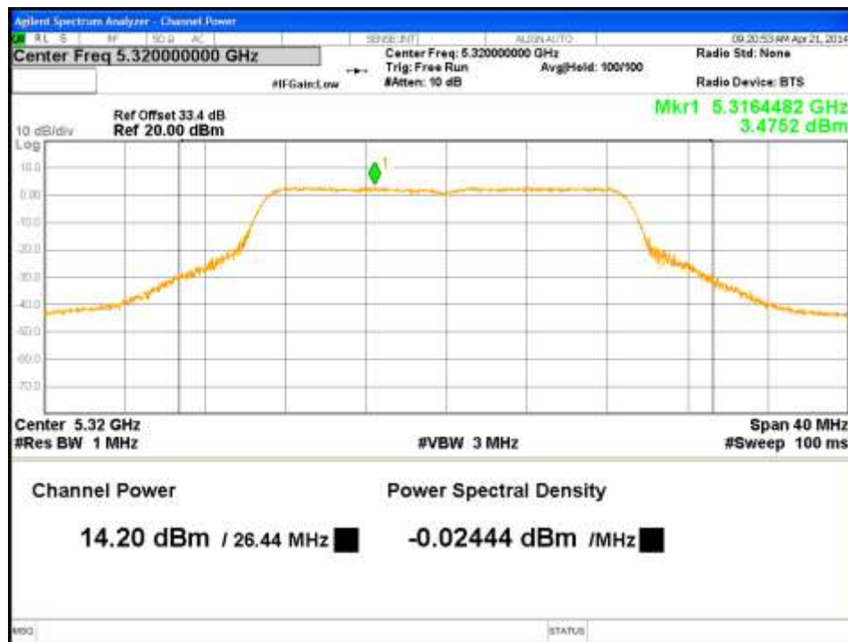
Figure 23: Maximum Conducted Output Power-5320MHz-HT20-MCS0-Ch2
