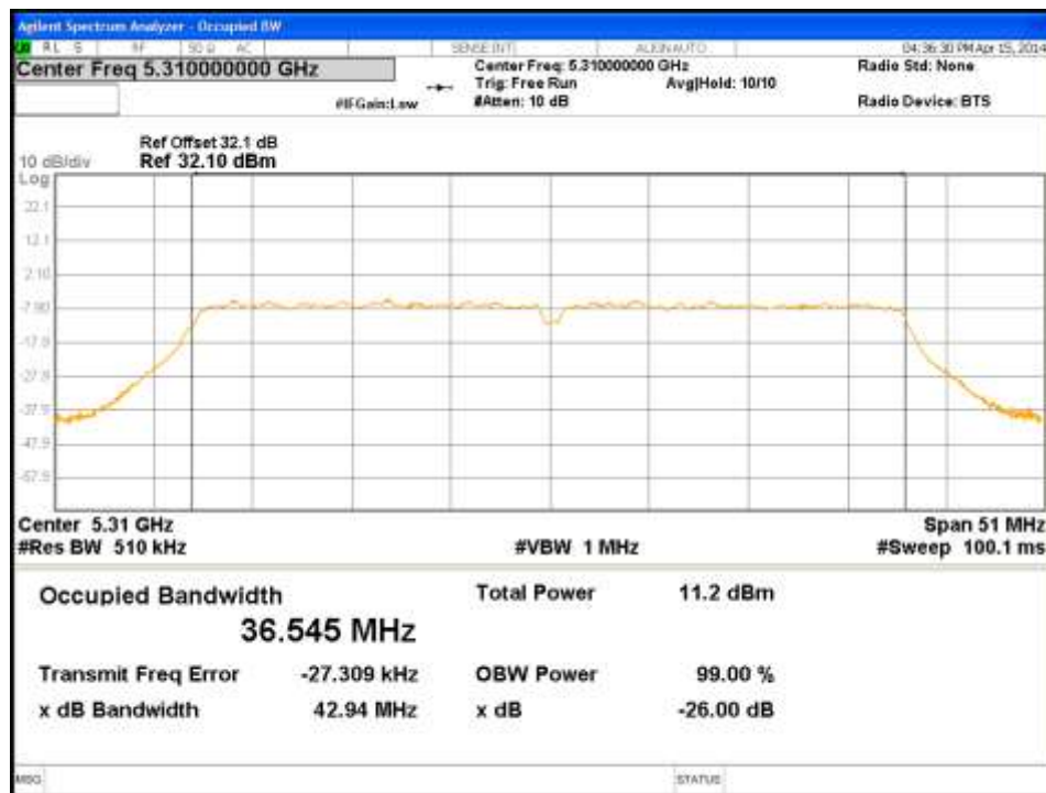
Figure 107: Occupied Bandwidth-5310MHz-VHT40-MCS0-Ch2
