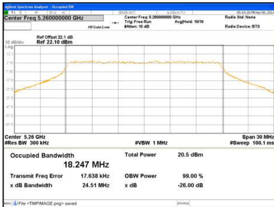
Figure 69: Occupied Bandwidth-5260MHz-HT20-MCS0-Ch0
