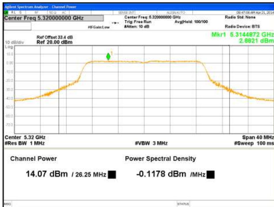
Figure 44: Maximum Conducted Output Power-5320MHz-VHT20-MCS0-Ch3
