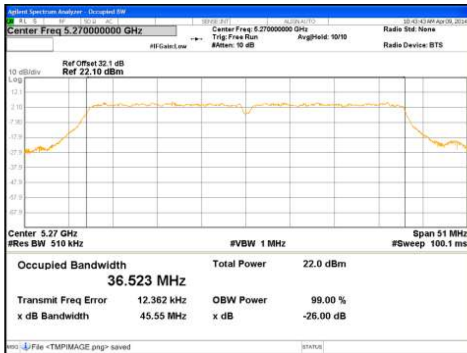
Figure 83: Occupied Bandwidth-5270MHz-HT40-MCS0-Ch2
