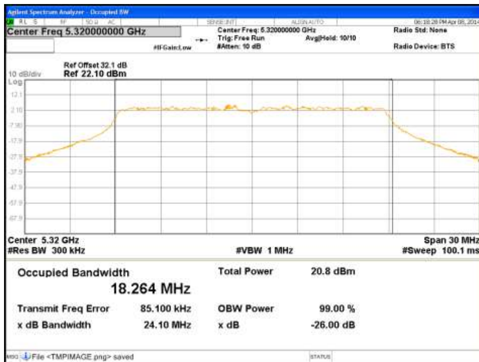
Figure 80: Occupied Bandwidth-5320MHz-HT20-MCS0-Ch3
