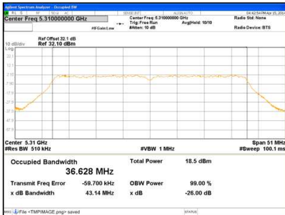
Figure 108: Occupied Bandwidth-5310MHz-VHT40-MCS0-Ch3
