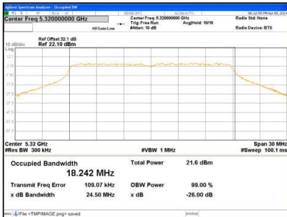
Figure 78: Occupied Bandwidth-5320MHz-HT20-MCS0-Ch1
