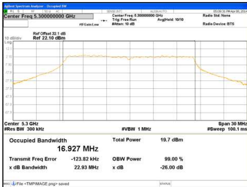
Figure 61: Occupied Bandwidth-5300MHz-11a-6Mbps-Ch0
