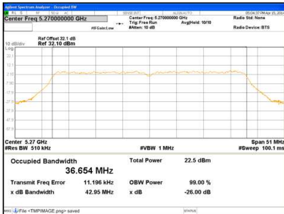
Figure 102: Occupied Bandwidth-5270MHz-VHT40-MCS0-Ch1
