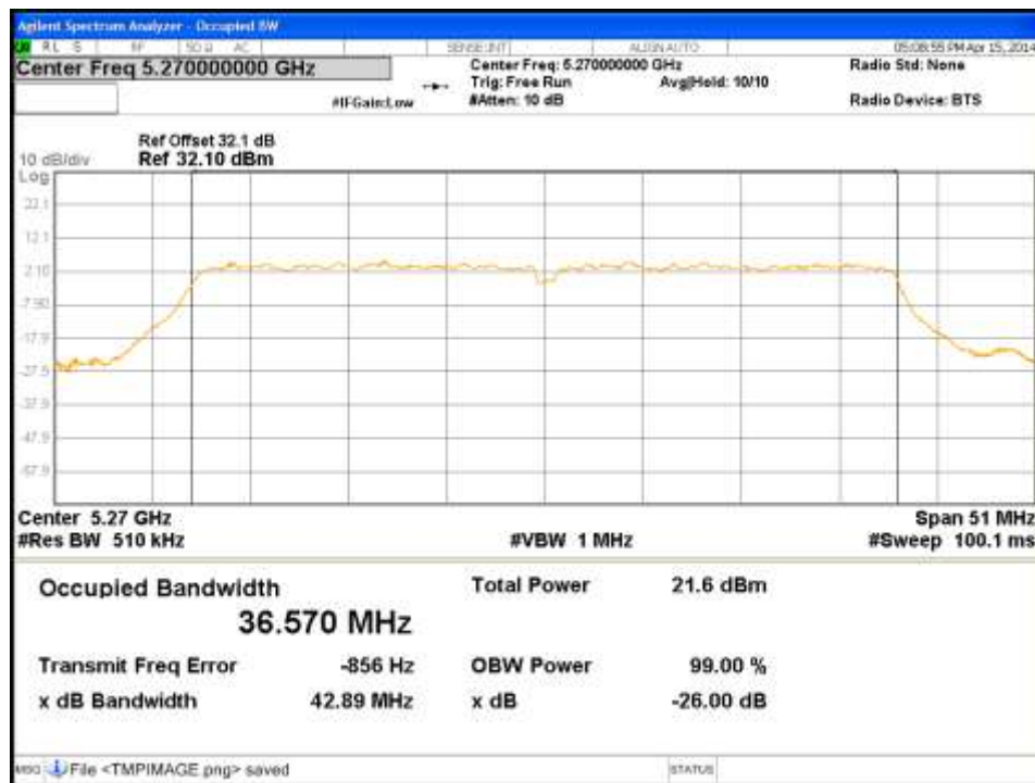
Figure 103: Occupied Bandwidth-5270MHz-VHT40-MCS0-Ch2
