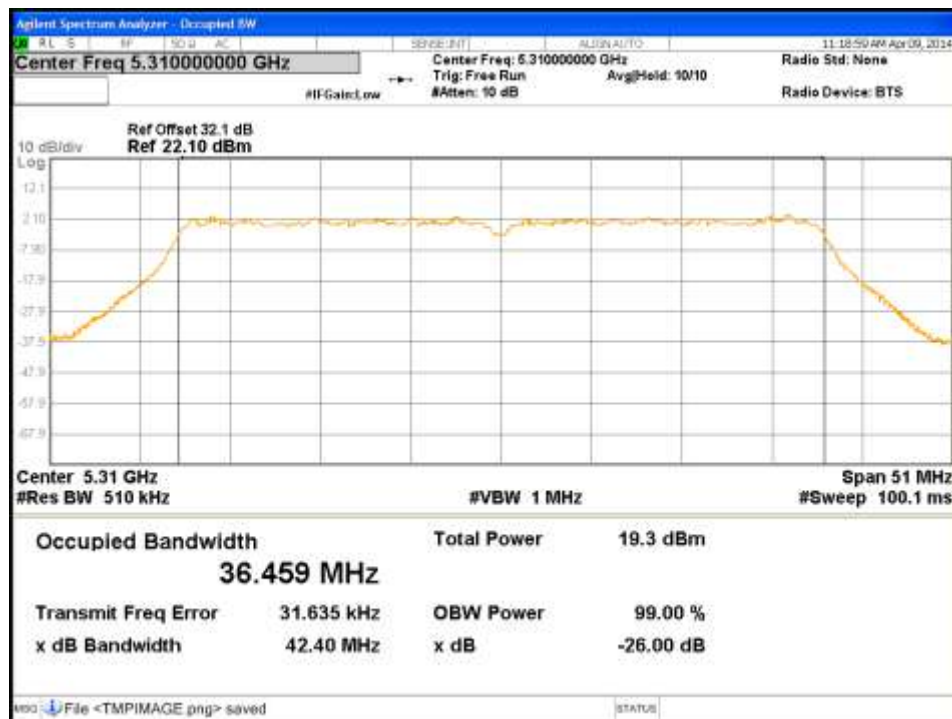
Figure 86: Occupied Bandwidth-5310MHz-HT40-MCS0-Ch1
