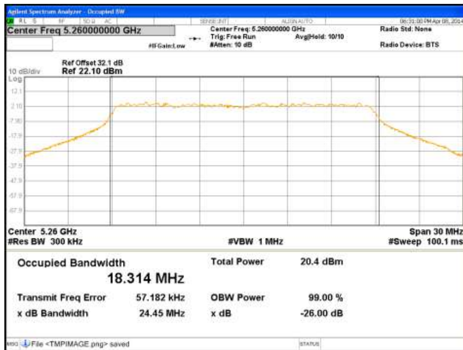
Figure 91: Occupied Bandwidth-5260MHz-VHT20-MCS0-Ch2
