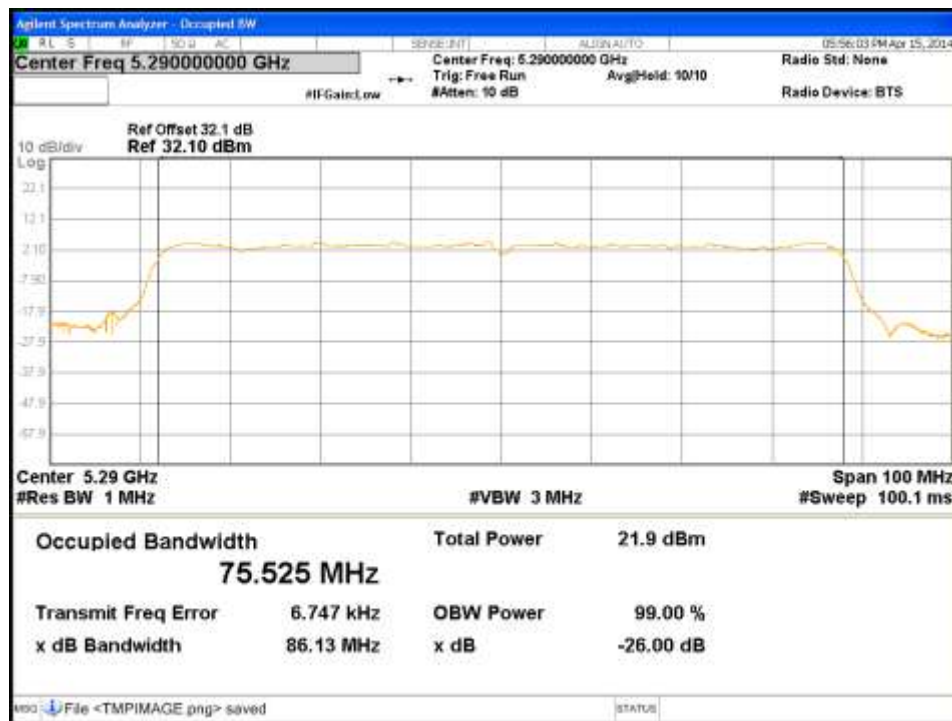
Figure 111: Occupied Bandwidth-5290MHz-VHT80-MCS0-Ch2
