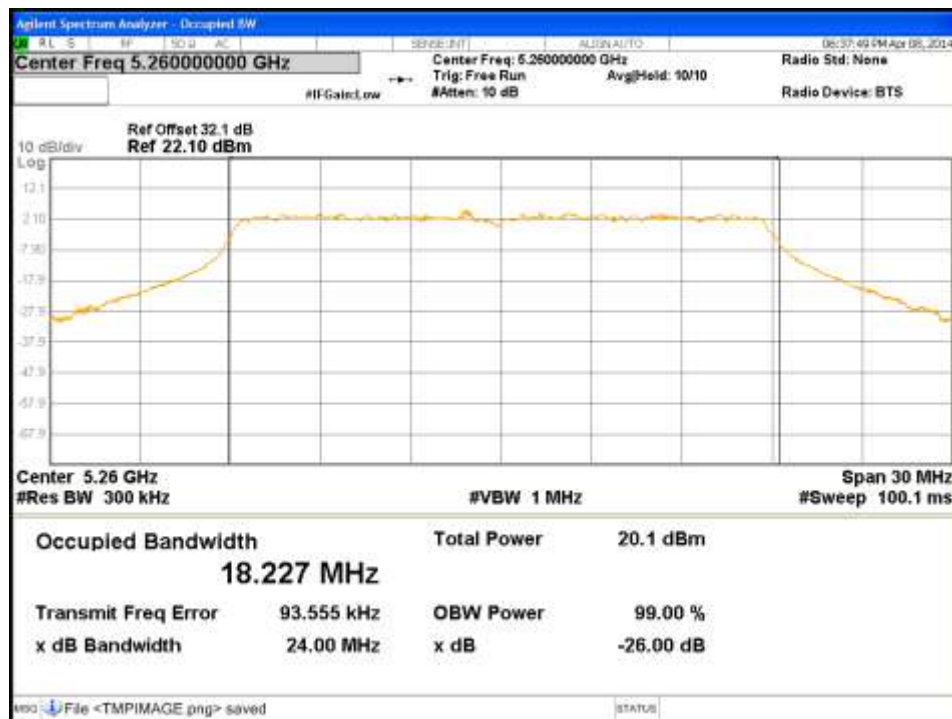
Figure 92: Occupied Bandwidth-5260MHz-VHT20-MCS0-Ch3
