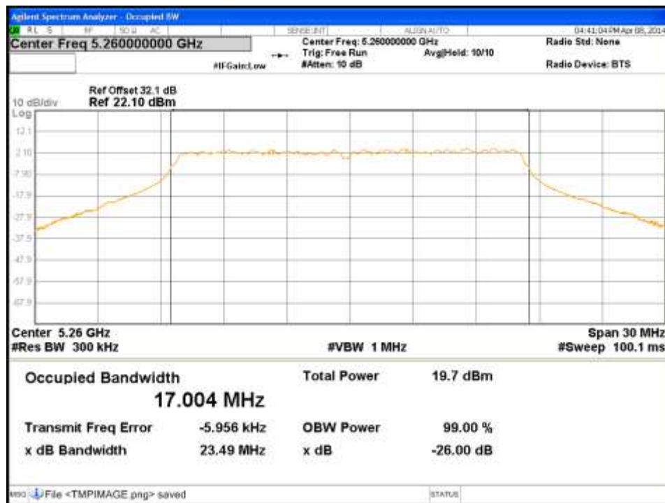
Figure 57: Occupied Bandwidth-5260MHz-11a-6Mbps-Ch0
