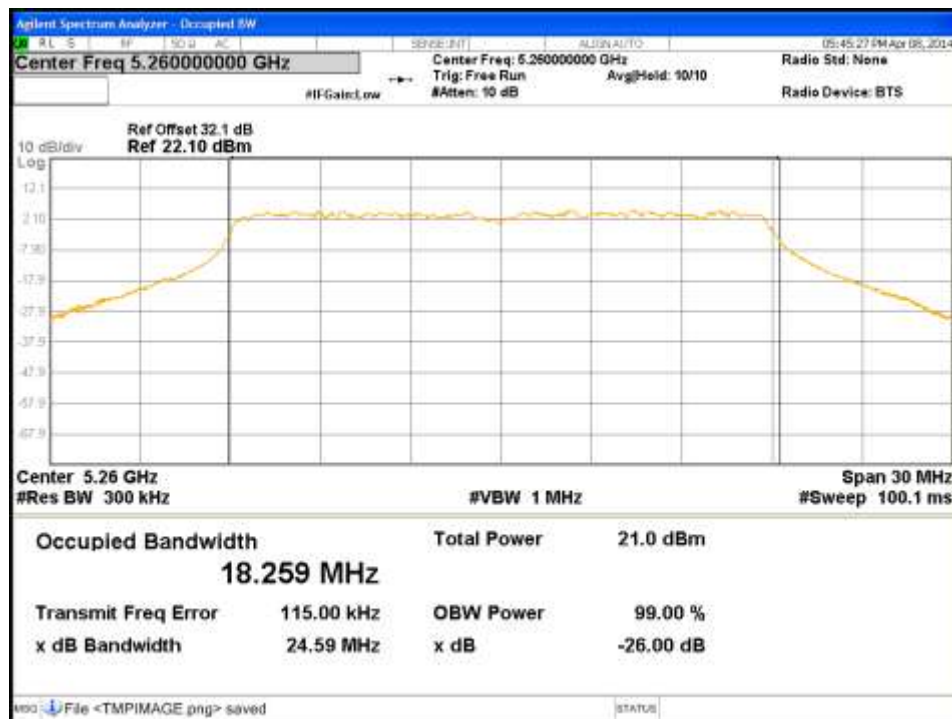
Figure 70: Occupied Bandwidth-5260MHz-HT20-MCS0-Ch1
