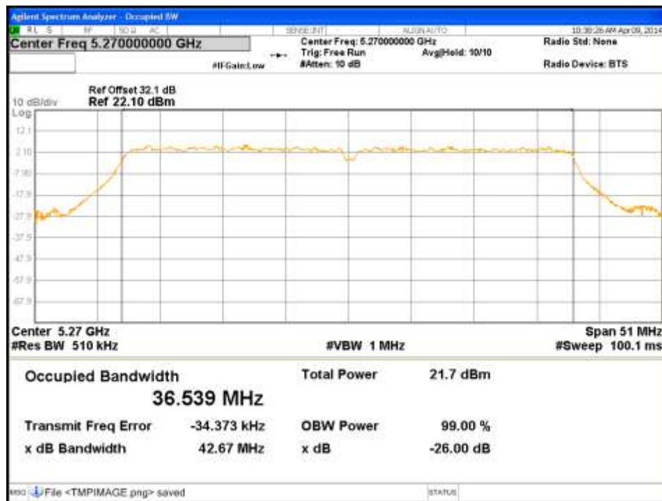
Figure 81: Occupied Bandwidth-5270MHz-HT40-MCS0-Ch0
