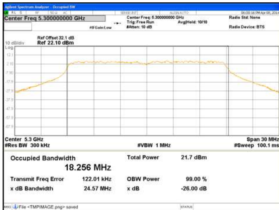
Figure 74: Occupied Bandwidth-5300MHz-HT20-MCS0-Ch1
