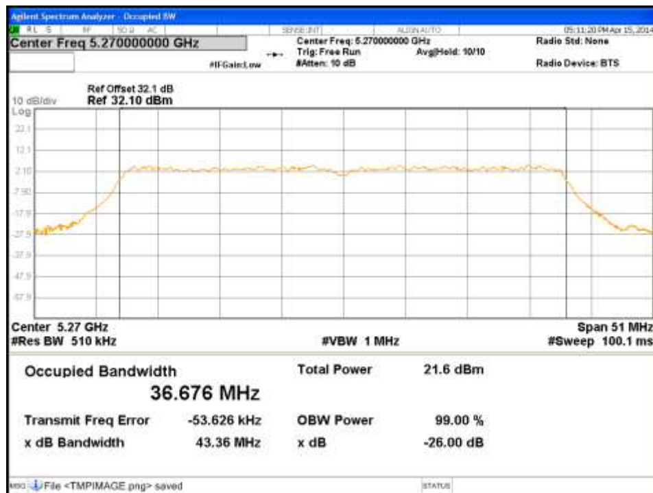
Figure 104: Occupied Bandwidth-5270MHz-VHT40-MCS0-Ch3
