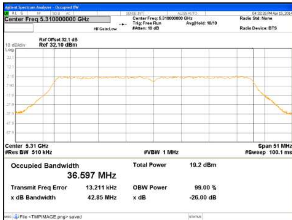
Figure 106: Occupied Bandwidth-5310MHz-VHT40-MCS0-Ch1
