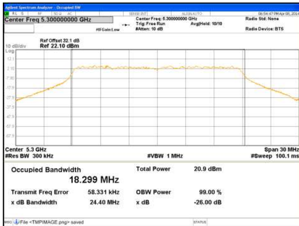
Figure 95: Occupied Bandwidth-5300MHz-VHT20-MCS0-Ch2
