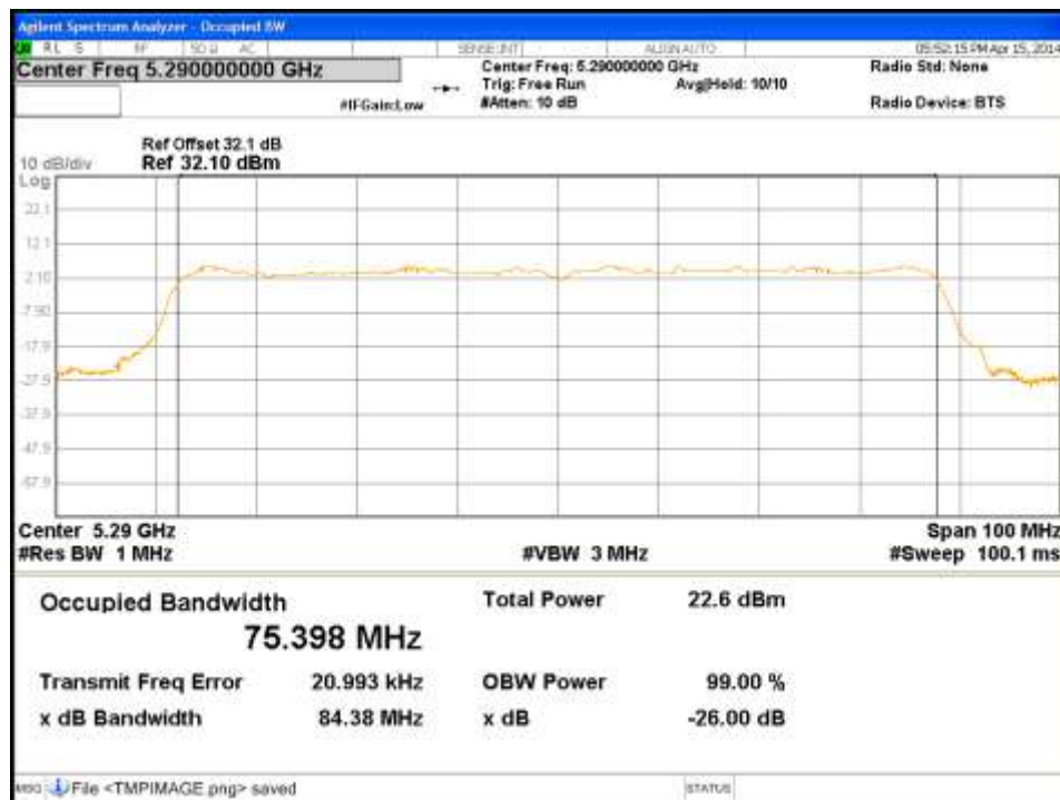
Figure 110: Occupied Bandwidth-5290MHz-VHT80-MCS0-Ch1
