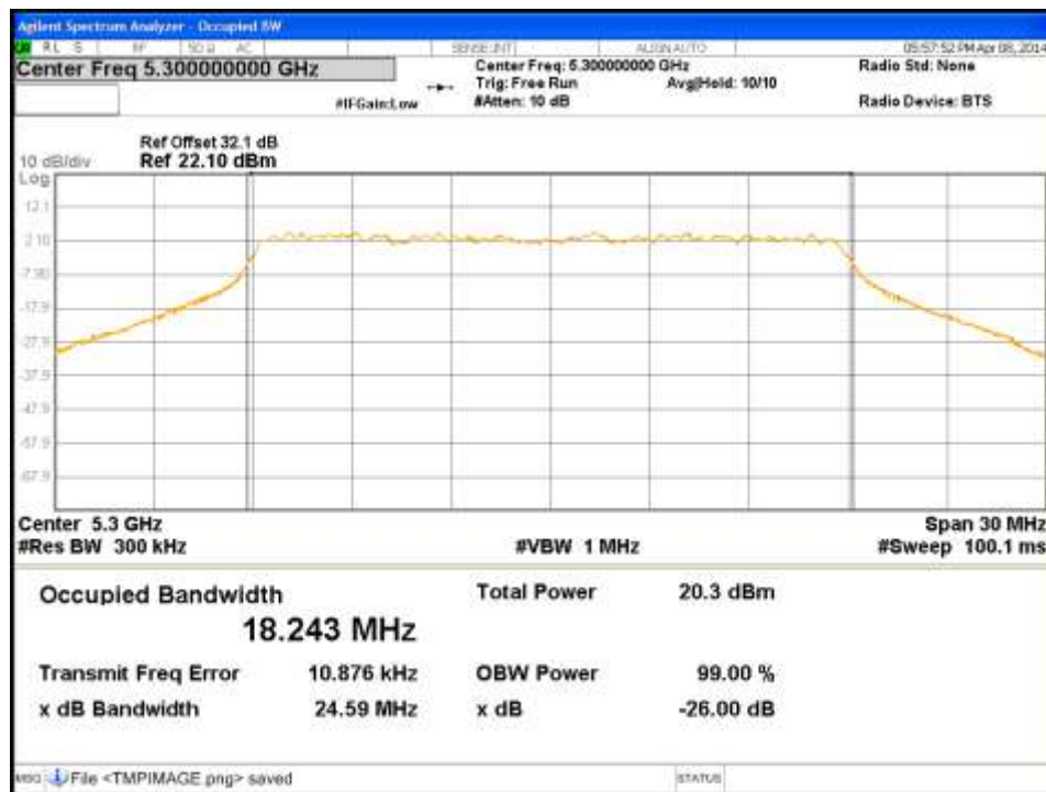
Figure 73: Occupied Bandwidth-5300MHz-HT20-MCS0-Ch0
