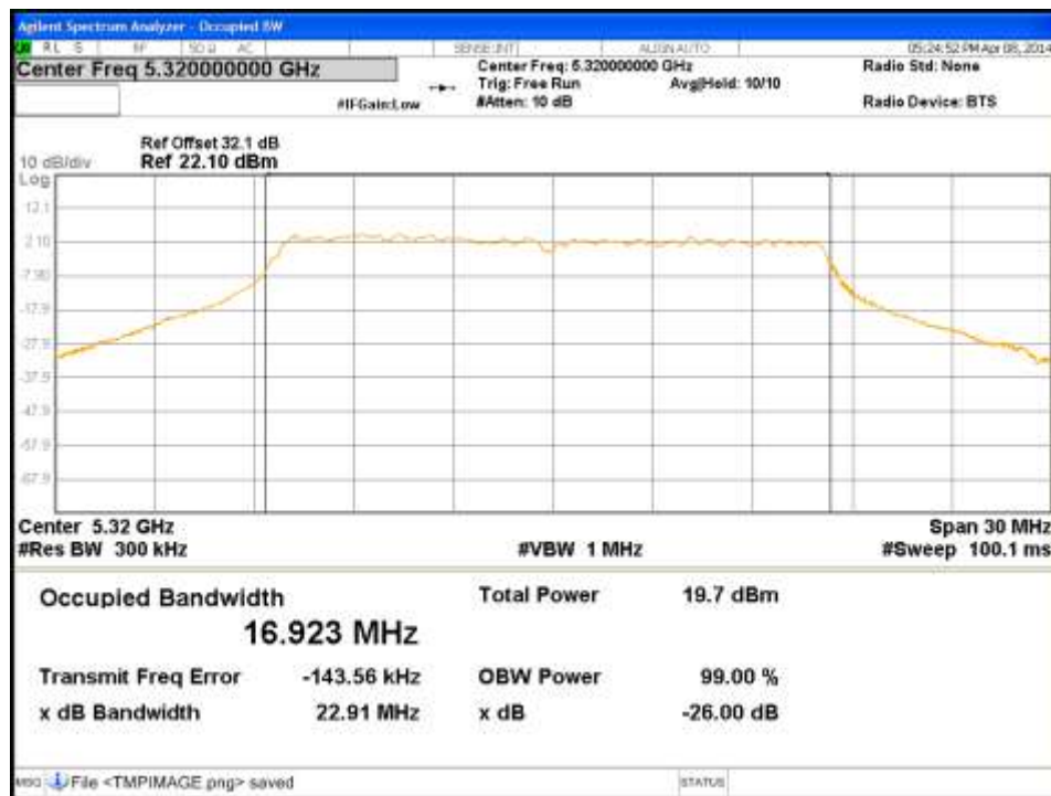
Figure 65: Occupied Bandwidth-5320MHz-11a-6Mbps-Ch0
