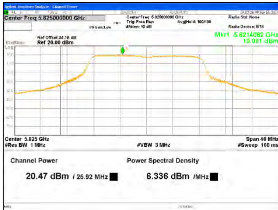
Figure 9: Maximum Conducted Output Power-5825MHz-11a-6Mbps-Ch0
