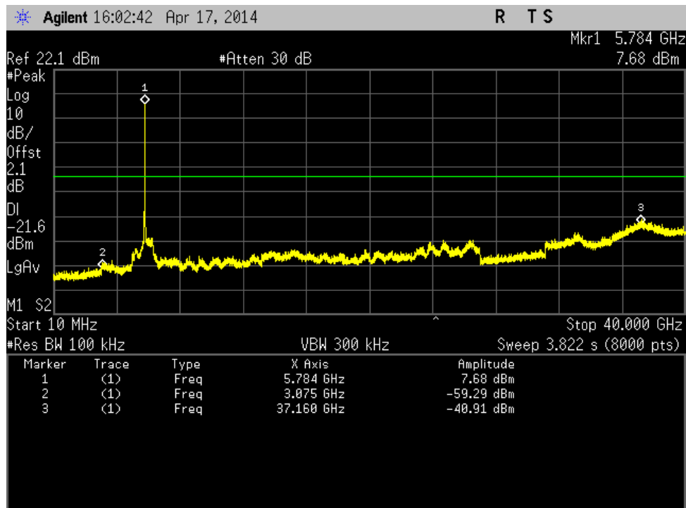
Figure 178: Out of Band Emission-802.11a-5785 MHz-6 Mbps-Ch0
