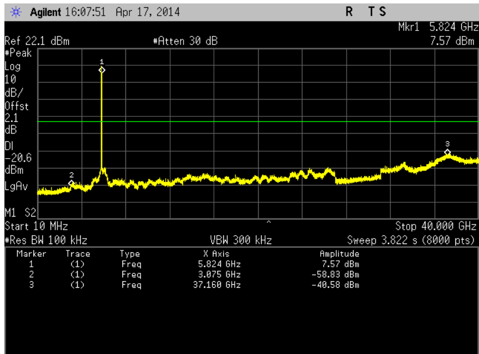
Figure 186: Out of Band Emission-802.11a-5825 MHz-6 Mbps-Ch0
