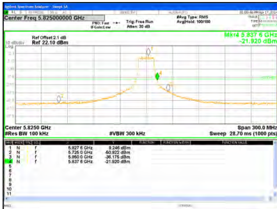
Figure 249: Conducted Band Edge-5825MHz-VHT20-MCS0-Ch0
