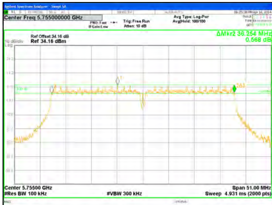
Figure 147: DTS Bandwidth-5755MHz-VHT40-MCS0-Ch2
