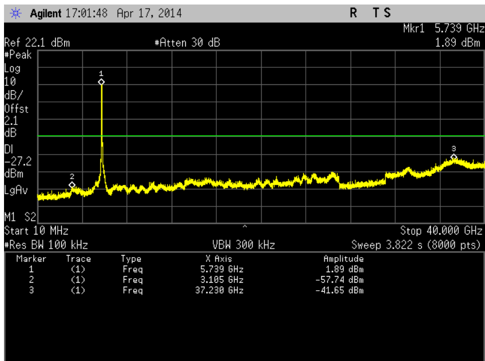
Figure 278: Out of Band Emission-802.11ac VHT80-5775 MHz-MCS0-Ch2
