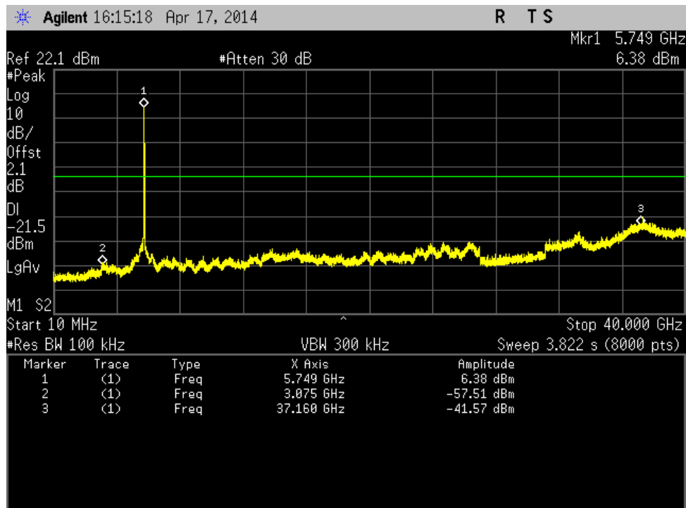
Figure 196: Out of Band Emission-802.11n HT20-5745 MHz-MCS0-Ch1
