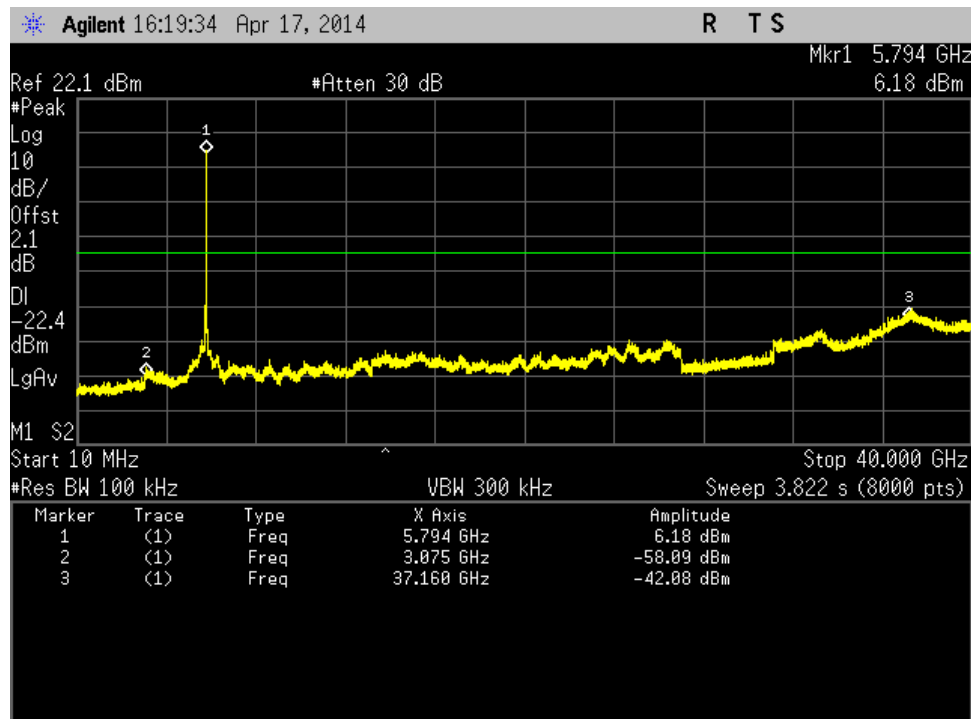
Figure 204: Out of Band Emission-802.11n HT20-5785 MHz-MCS0-Ch1
