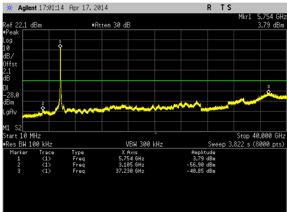
Figure 276: Out of Band Emission-802.11ac VHT80-5775 MHz-MCS0-Ch1
