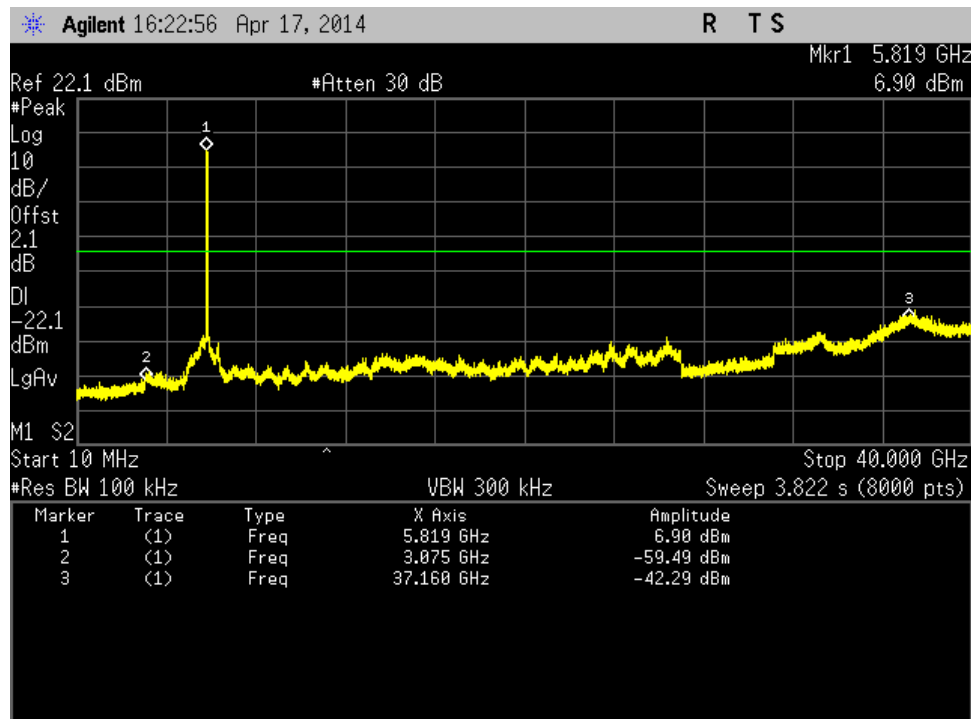
Figure 212: Out of Band Emission-802.11n HT20-5825 MHz-MCS0-Ch1
