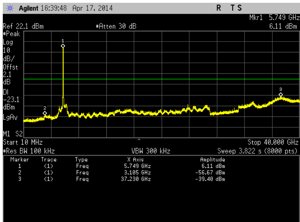
Figure 218: Out of Band Emission-802.11n HT40-5755 MHz-MCS0-Ch0
