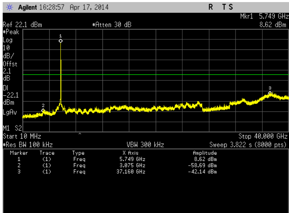
Figure 236: Out of Band Emission-802.11ac VHT20-5745 MHz-MCS0-Ch1
