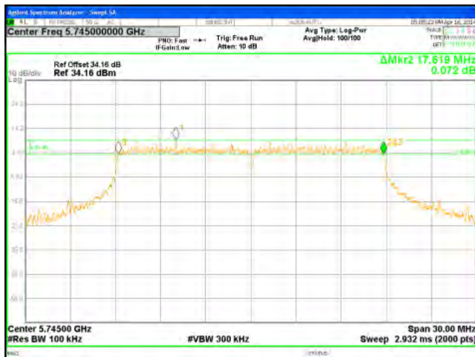
Figure 124: DTS Bandwidth-5745MHz-VHT20-MCS0-Ch3
