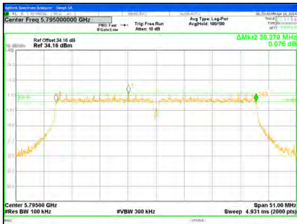
Figure 151: DTS Bandwidth-5795MHz-VHT40-MCS0-Ch2
