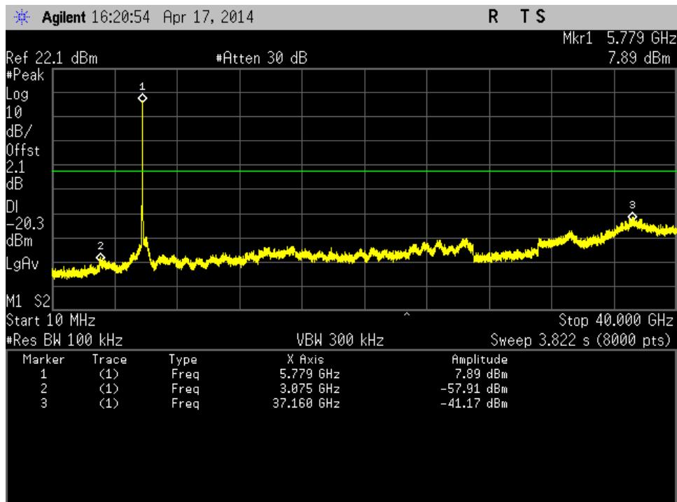
Figure 208: Out of Band Emission-802.11n HT20-5785 MHz-MCS0-Ch3
