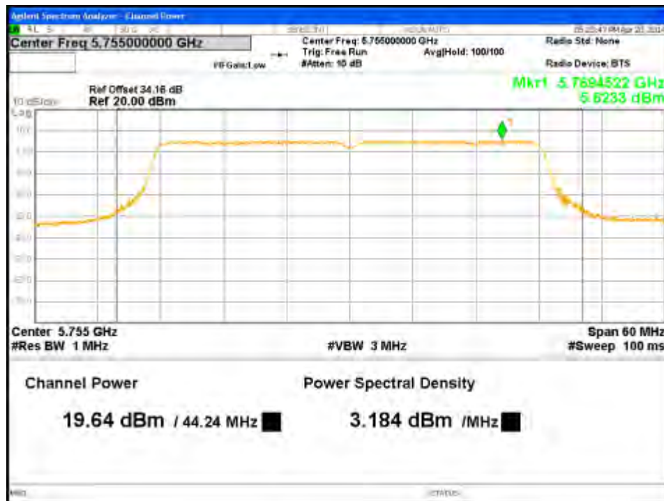
Figure 25: Maximum Conducted Output Power-5755MHz-HT40-MCS0-Ch0
