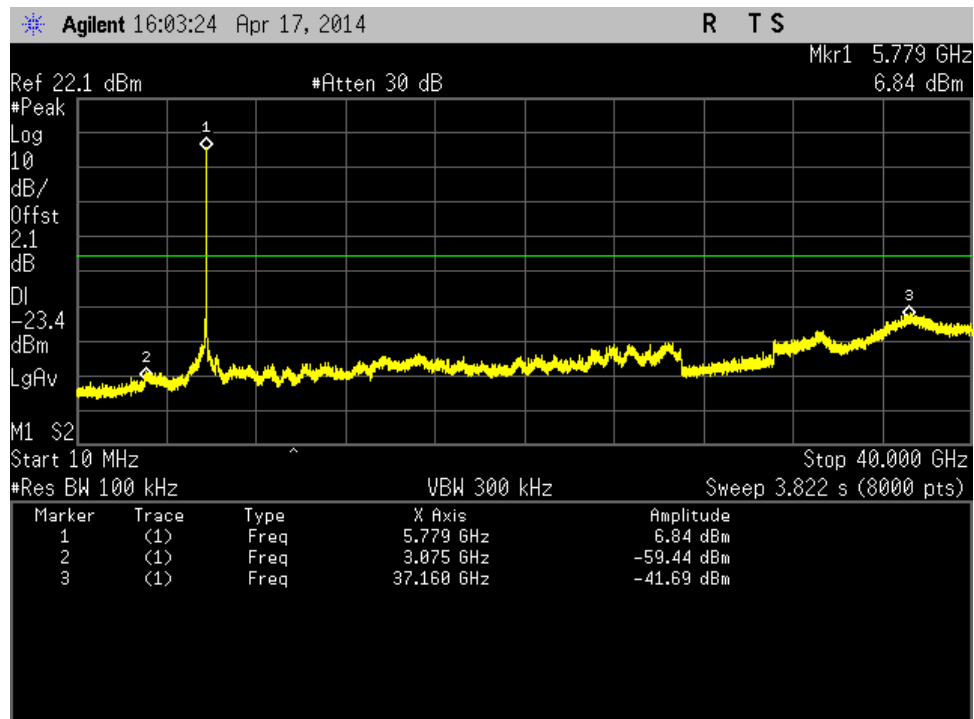
Figure 180: Out of Band Emission-802.11a-5785 MHz-6 Mbps-Ch1
