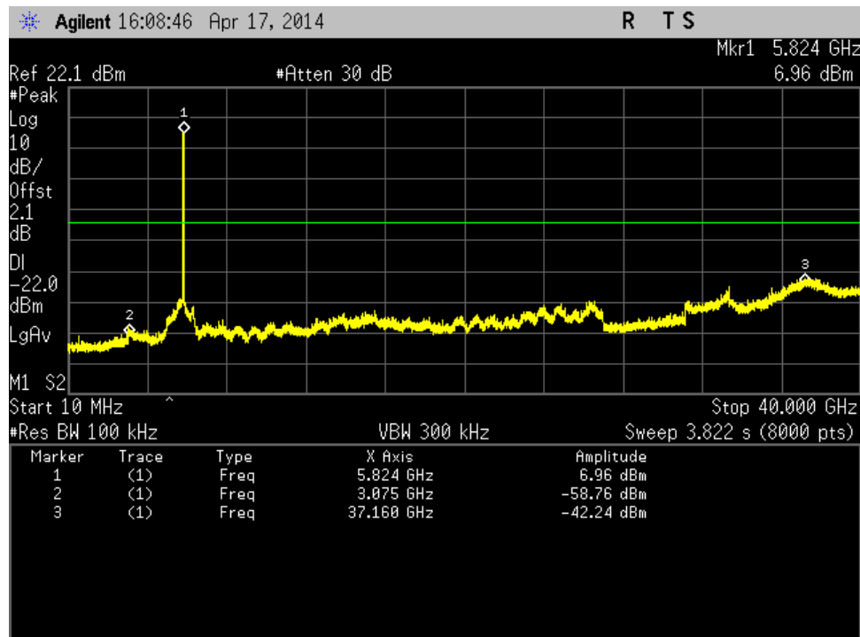
Figure 188: Out of Band Emission-802.11a-5825 MHz-6 Mbps-Ch1
