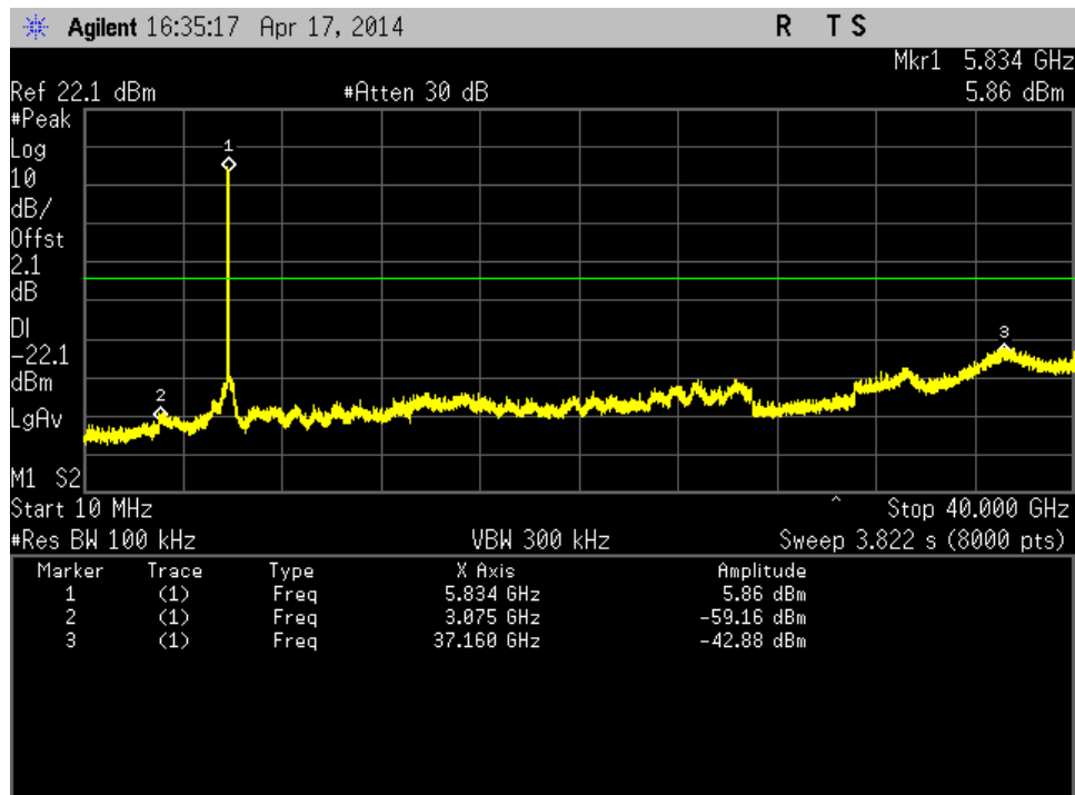
Figure 254: Out of Band Emission-802.11ac VHT20-5825 MHz-MCS0-Ch2
