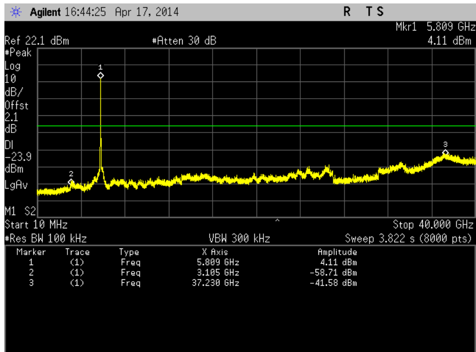
Figure 230: Out of Band Emission-802.11n HT40-5795 MHz-MCS0-Ch2
