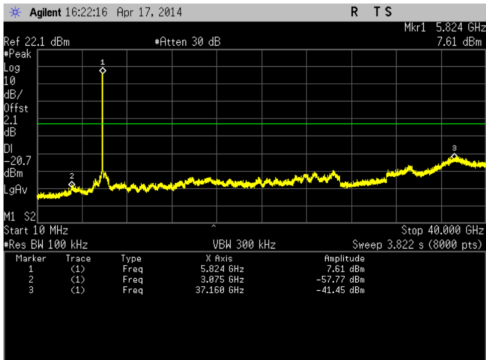
Figure 210: Out of Band Emission-802.11n HT20-5825 MHz-MCS0-Ch0
