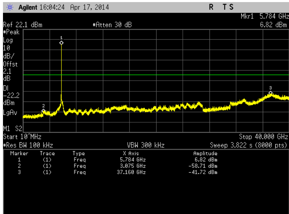
Figure 182: Out of Band Emission-802.11a-5785 MHz-6 Mbps-Ch2
