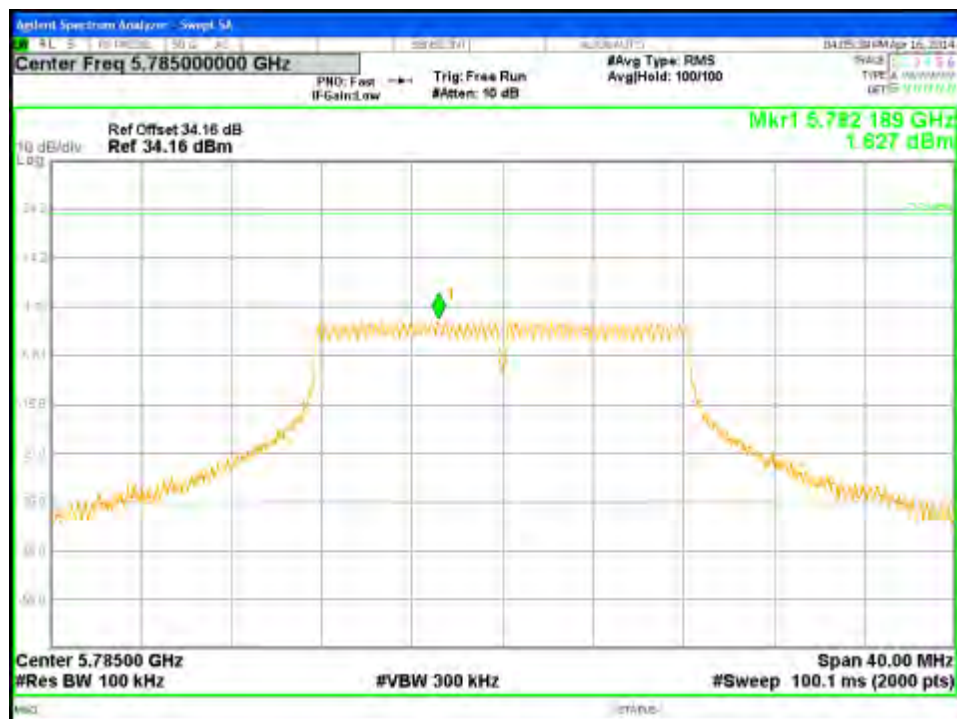
Figure 288: Maximum Power Spectral Density-5785MHz-11a-6Mbps-Ch3
