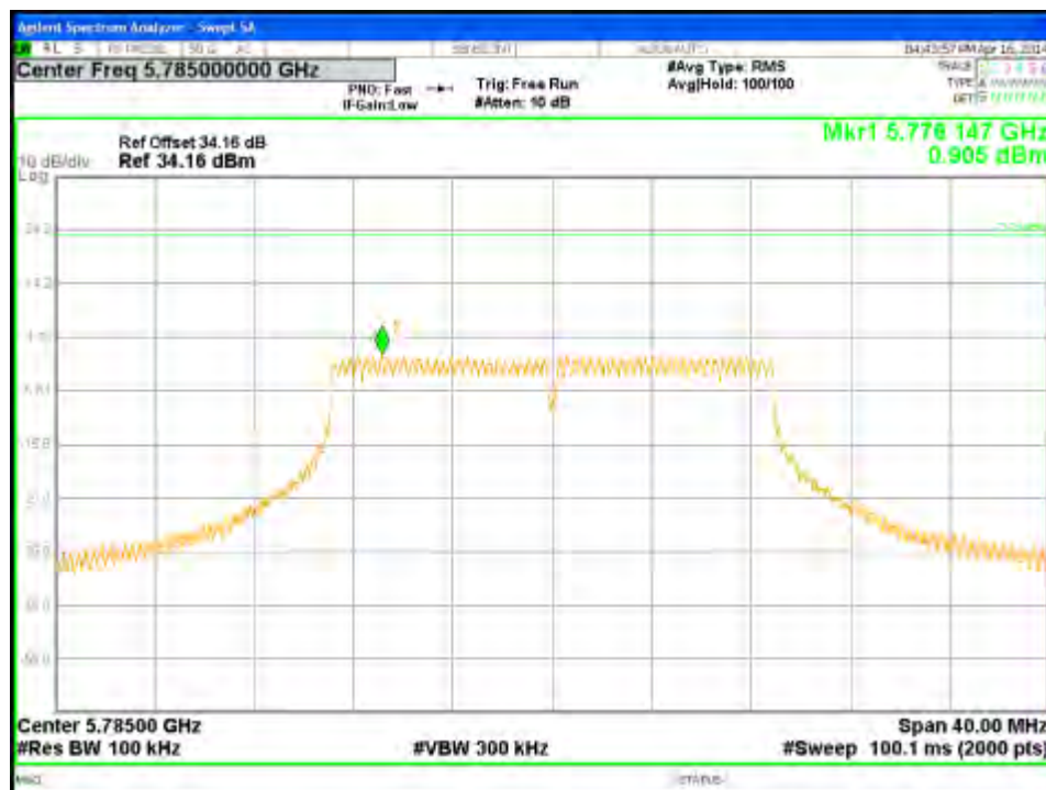
Figure 300: Maximum Power Spectral Density-5785MHz-HT20-MCS0-Ch3
