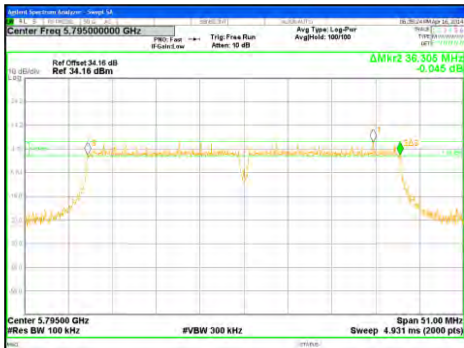
Figure 152: DTS Bandwidth-5795MHz-VHT40-MCS0-Ch3
