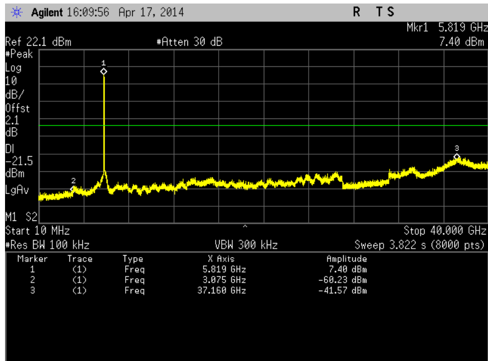
Figure 190: Out of Band Emission-802.11a-5825 MHz-6 Mbps-Ch2
