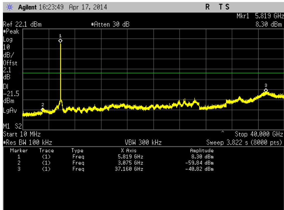
Figure 214: Out of Band Emission-802.11n HT20-5825 MHz-MCS0-Ch2
