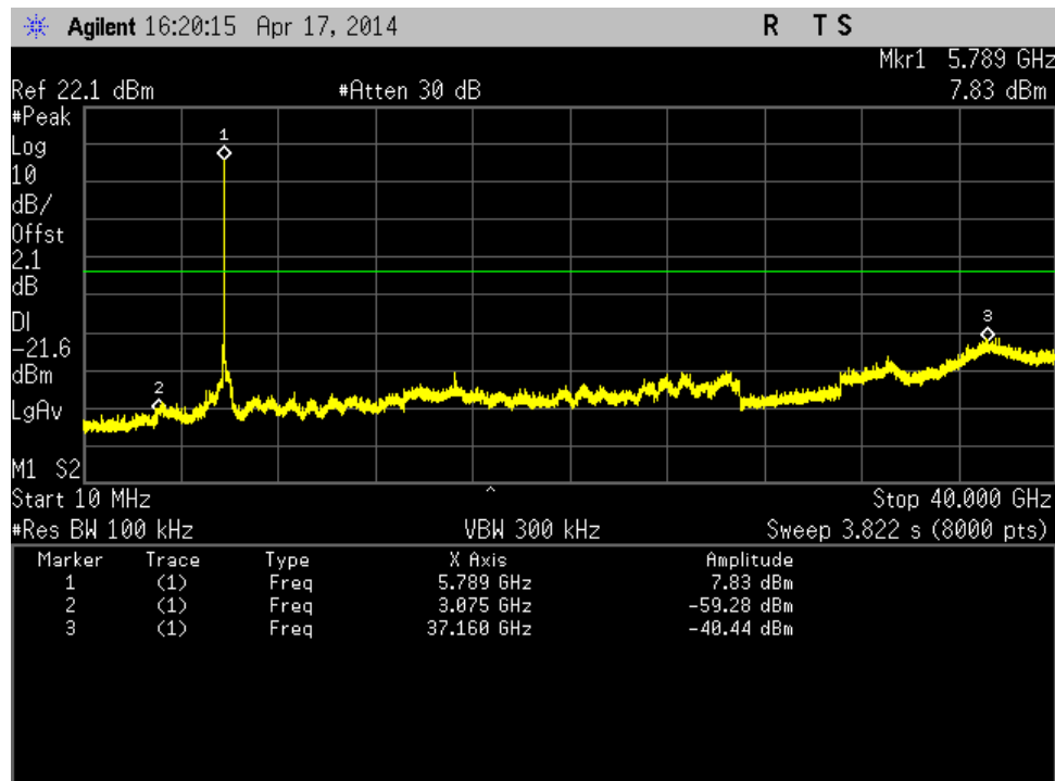
Figure 206: Out of Band Emission-802.11n HT20-5785 MHz-MCS0-Ch2
