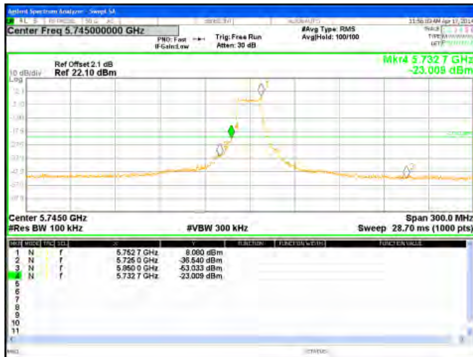
Figure 171: Conducted Band Edge-5745MHz-11a-6 Mbps-Ch1
