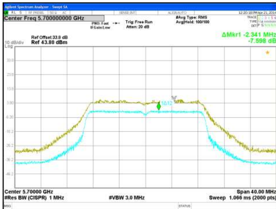
Figure 190: Peak Excursion-5700MHz-HT20-MCS0-Ch1
