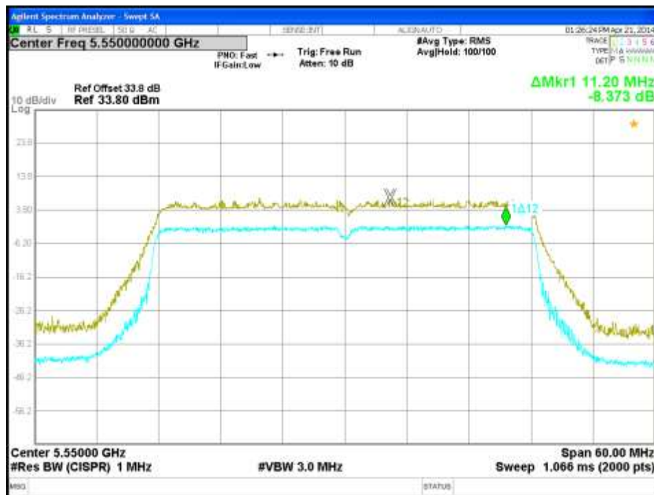
Figure 197: Peak Excursion-5550MHz-HT40-MCS0-Ch0
