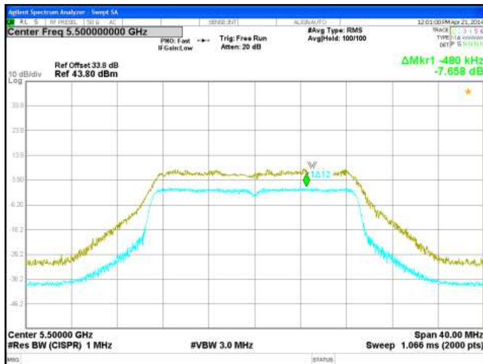
Figure 184: Peak Excursion-5500MHz-HT20-MCS0-Ch3
