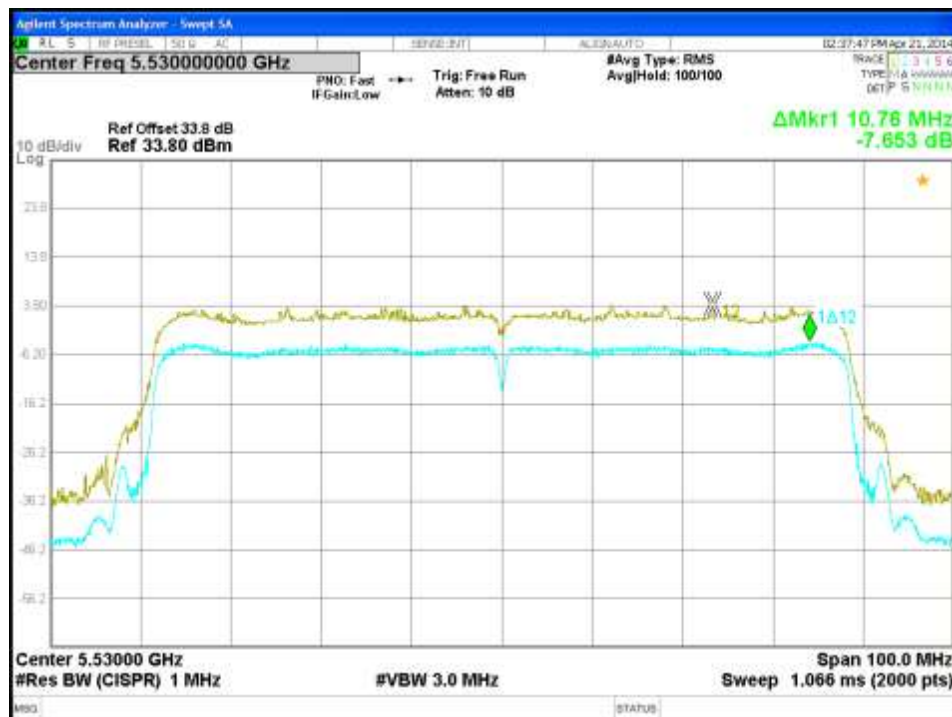
Figure 230: Peak Excursion-5530MHz-VHT80-MCS0-Ch1
