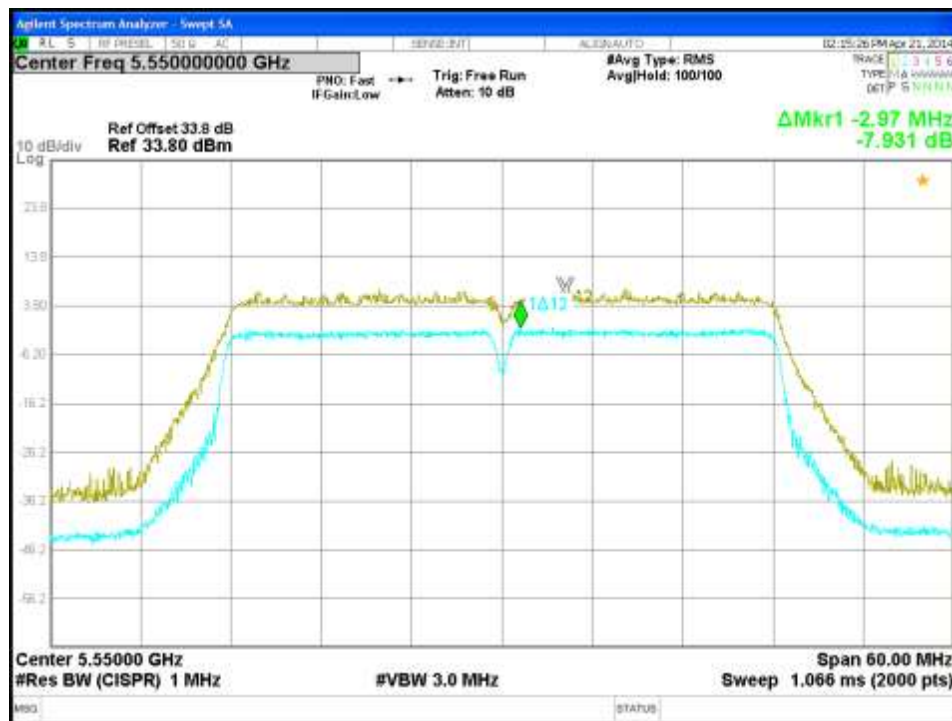
Figure 223: Peak Excursion-5550MHz-VHT40-MCS0-Ch2
