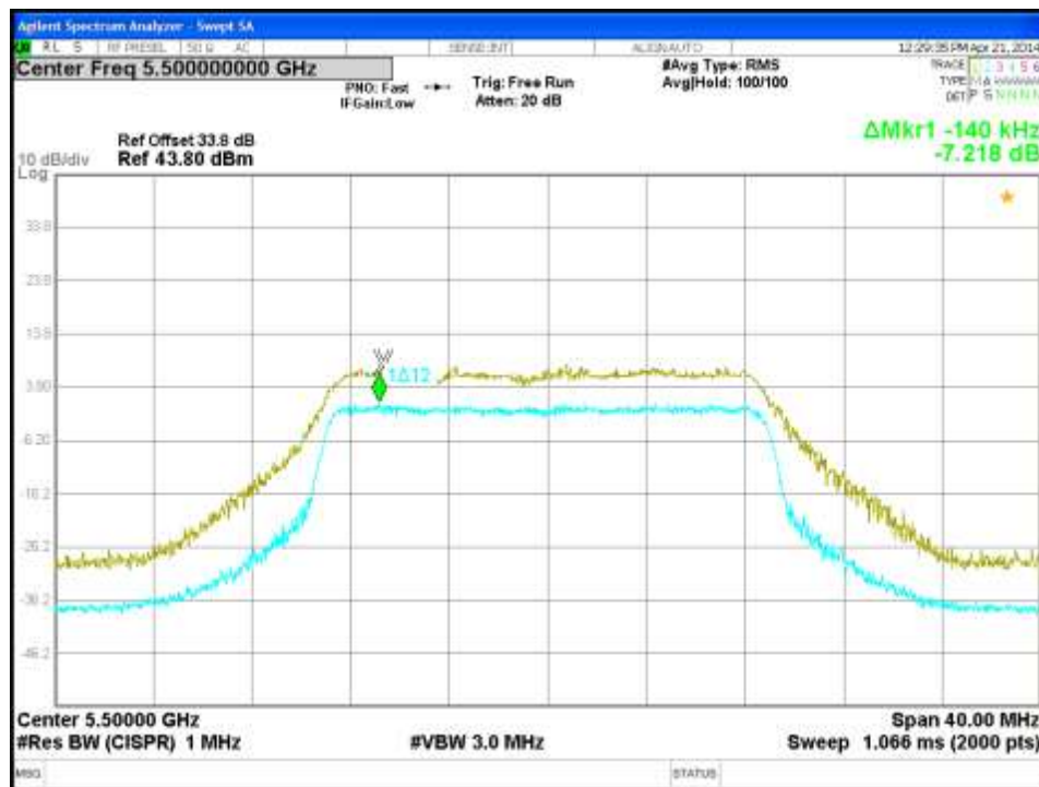
Figure 205: Peak Excursion-5500MHz-VHT20-MCS0-Ch0
