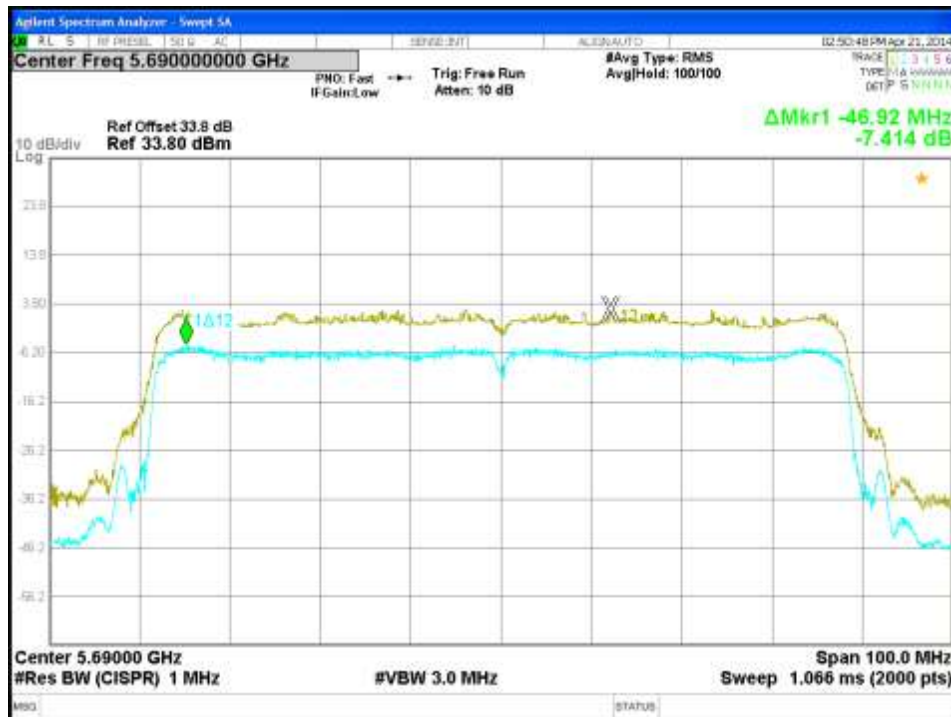
Figure 234: Peak Excursion-5690MHz-VHT80-MCS0-Ch1
