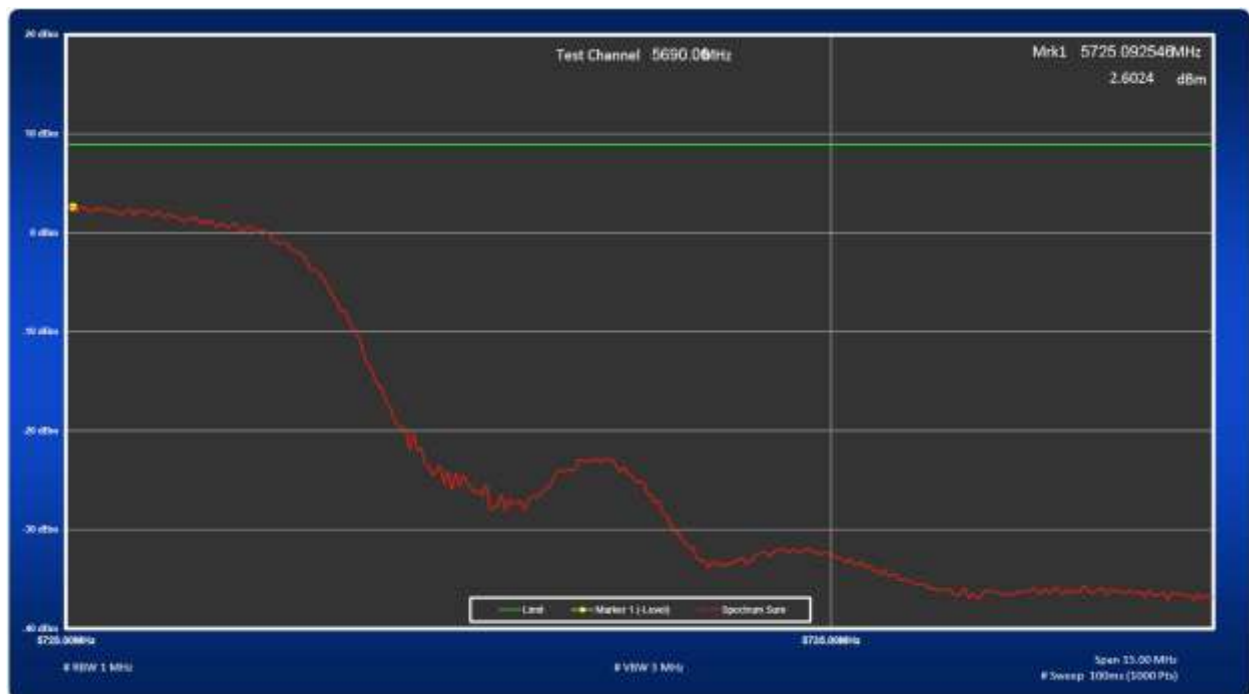
Figure 258: Total Sum of Power Spectral Density, 5690 MHz at 802.11ac VHT80 MCS0 – 2
