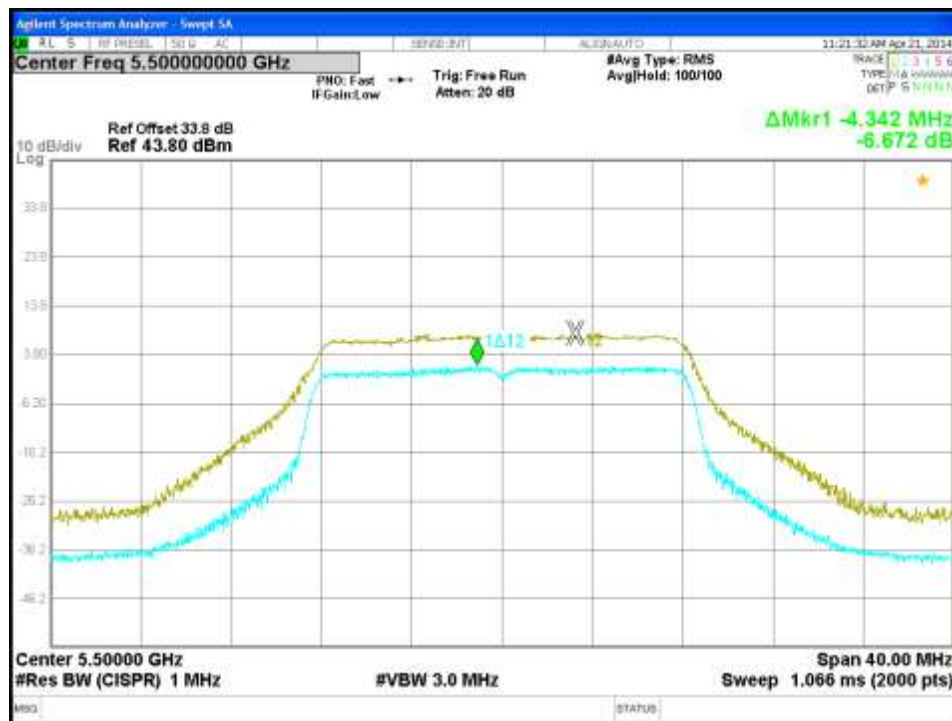
Figure 169: Peak Excursion-5500MHz-11a-6Mbps-Ch0
