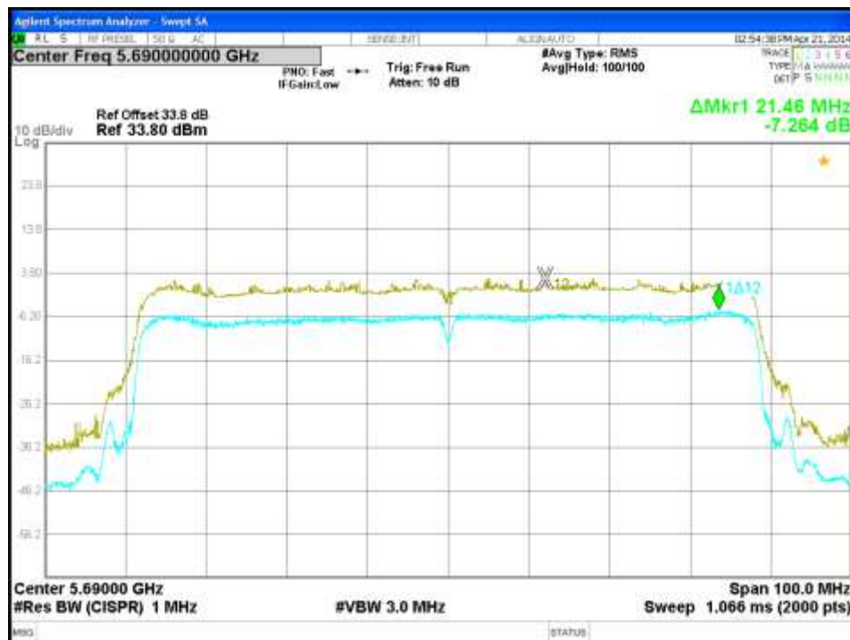
Figure 236: Peak Excursion-5690MHz-VHT80-MCS0-Ch3
