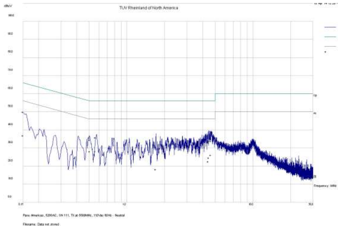
150 kHz to 30 MHz Plot for Line 2 (Neutral)
