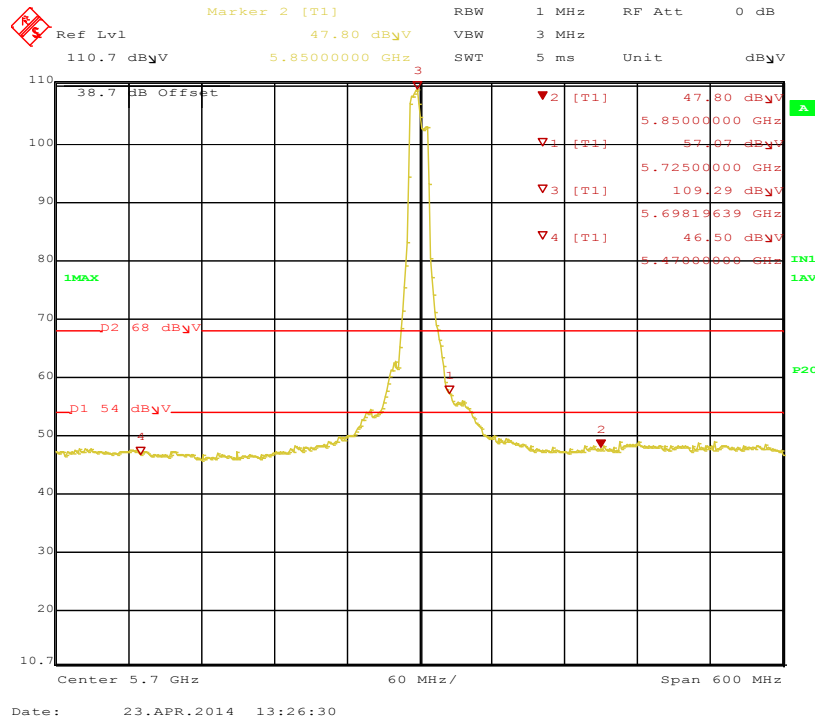
Figure 264: Bandedge-11a-6Mbps-5700 MHz-H-Ave
