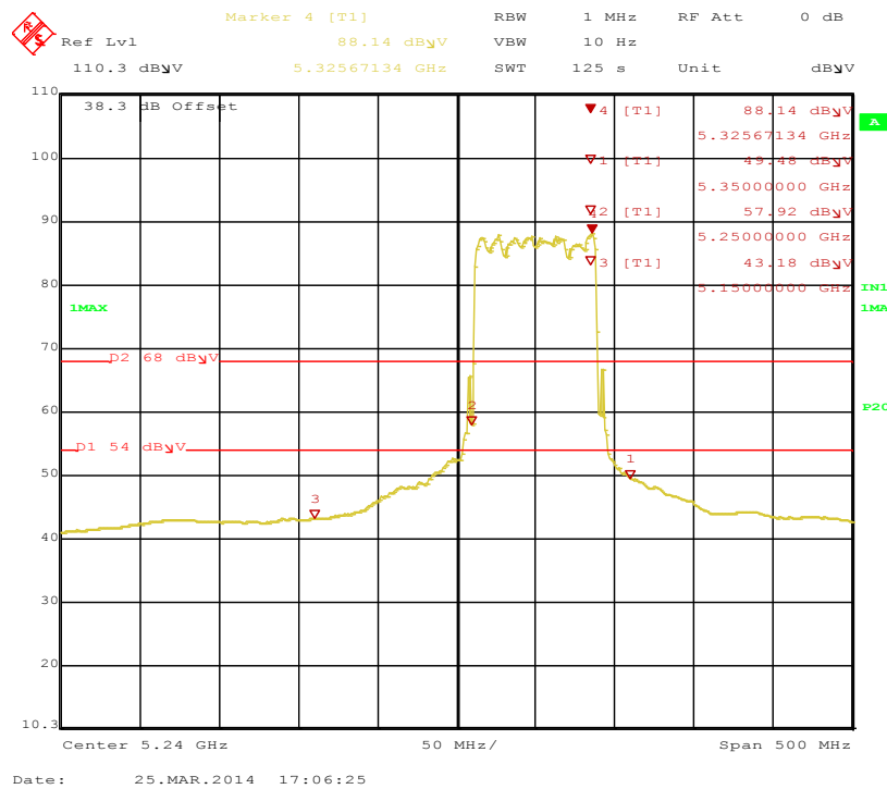
Figure 225: Bandedge-5290MHz-VHT80-MCS0-V-Ave
