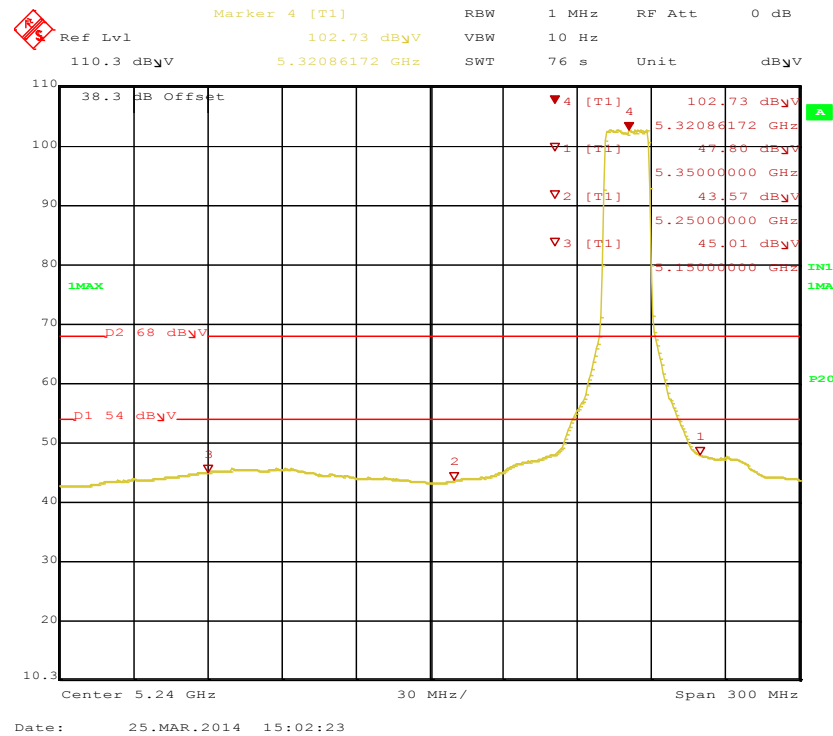
Figure 197: Bandedge-5320MHz-HT20-MCS0-V-Ave
