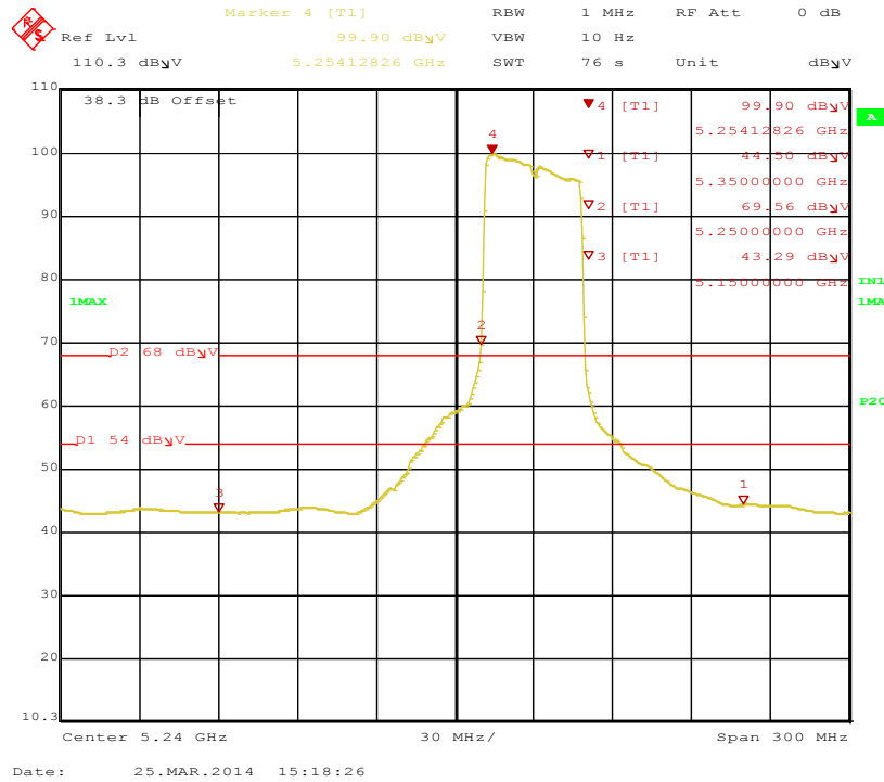
Figure 201: Bandedge-5270MHz-HT40-MCS0-V-ave
