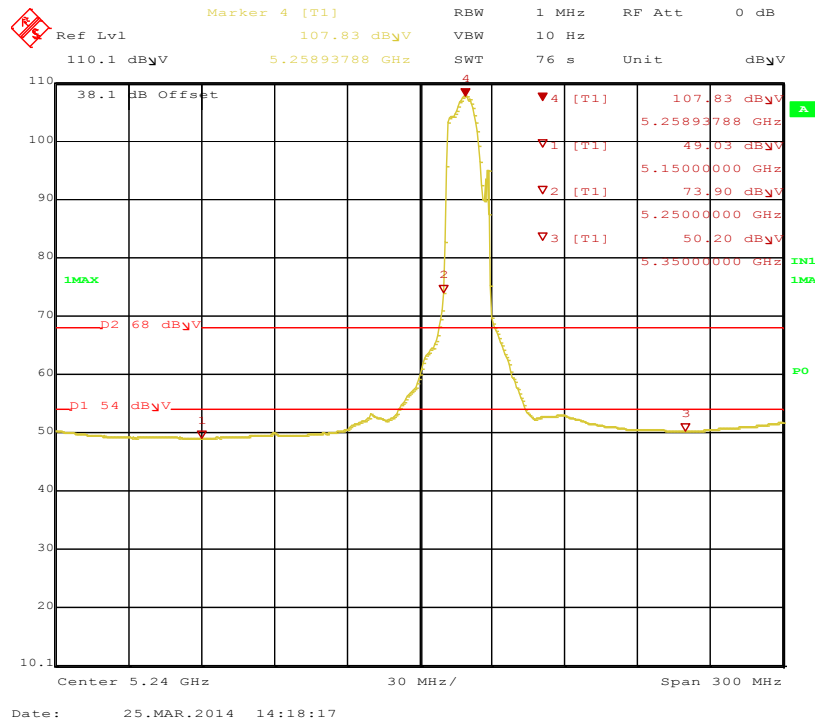
Figure 183: Bandedge-5260MHz-11a-MCS0-H-Ave
