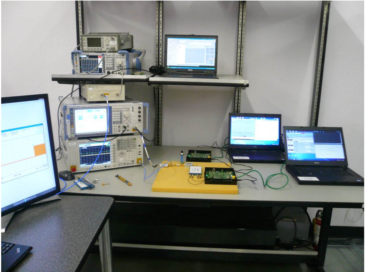
Figure 15: DFS Test Setup Photo
