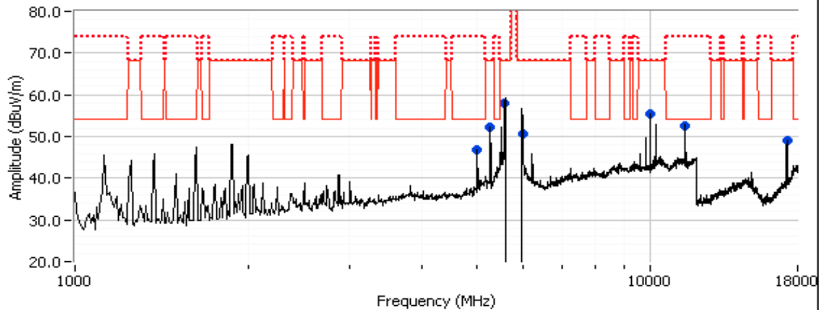
802.11n20, CH149
