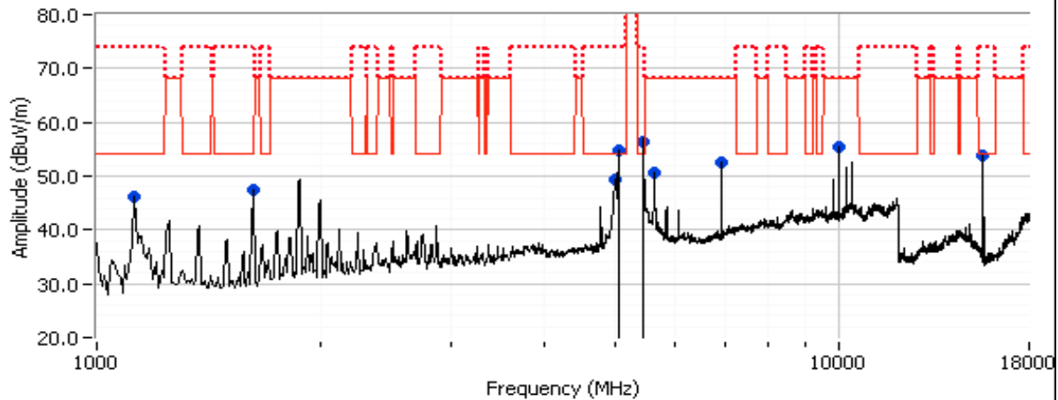
802.11n20, CH40
