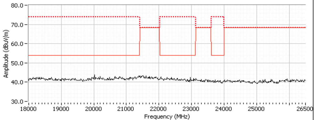
ac80, CH155
