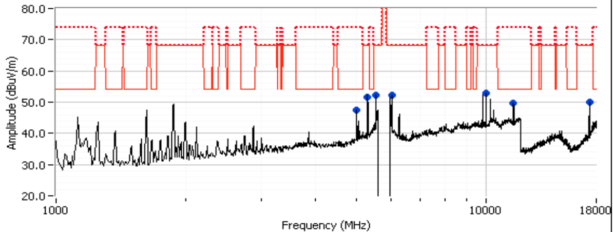
802.11n20, CH157
