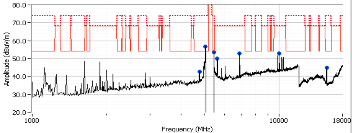
802.11n20, CH36
