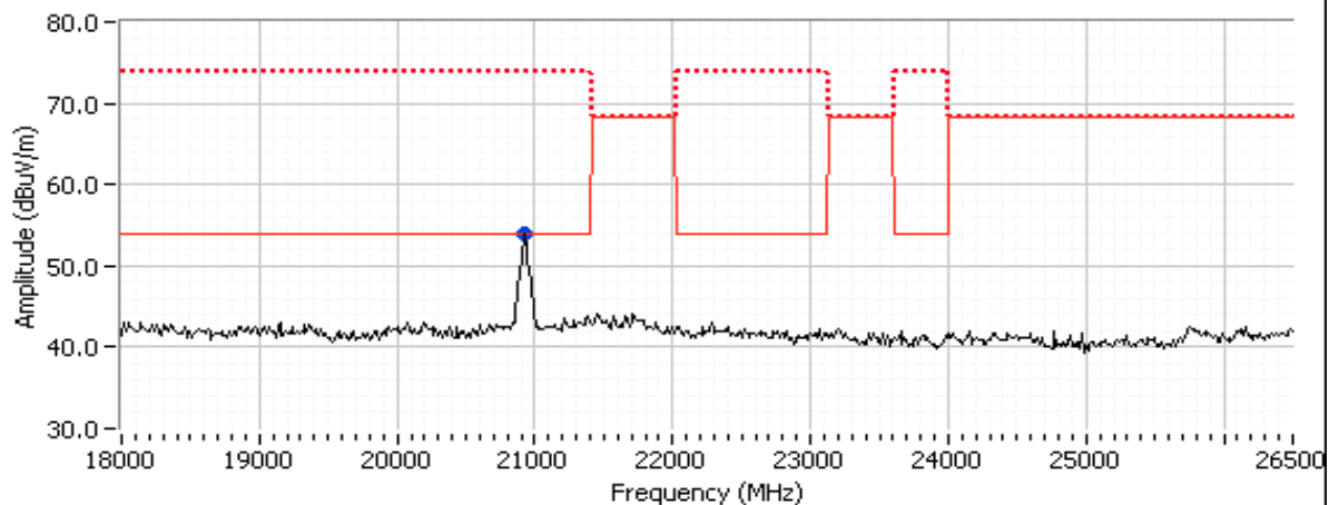
802.11n40, CH46
