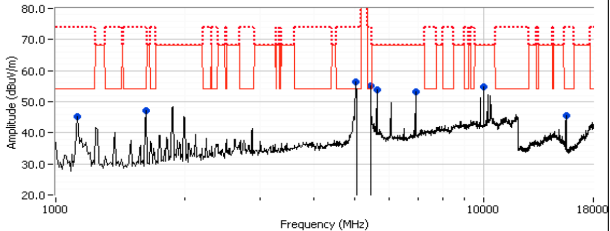
802.11n40, CH38
