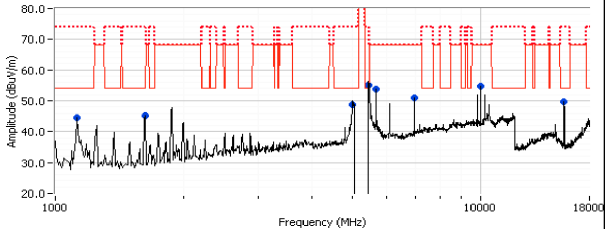
802.11n40, CH46
