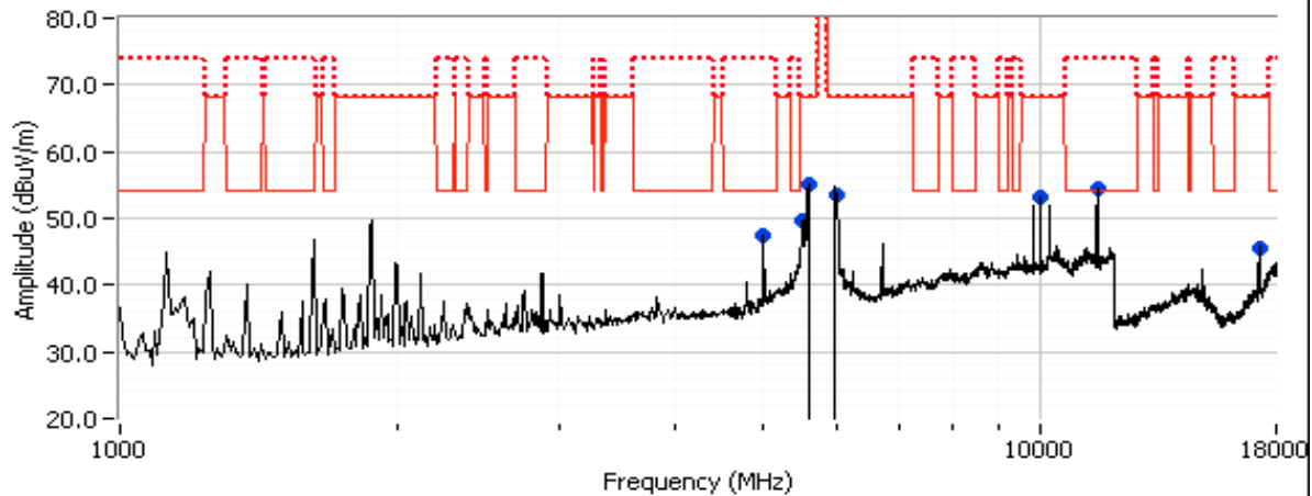
802.11n40, CH151
