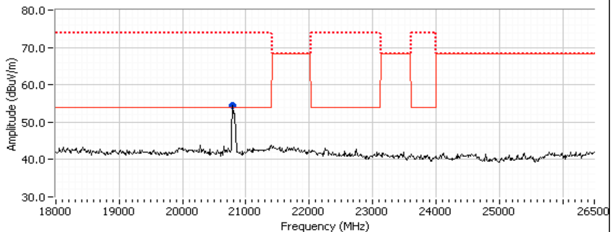
802.11n20, CH40
