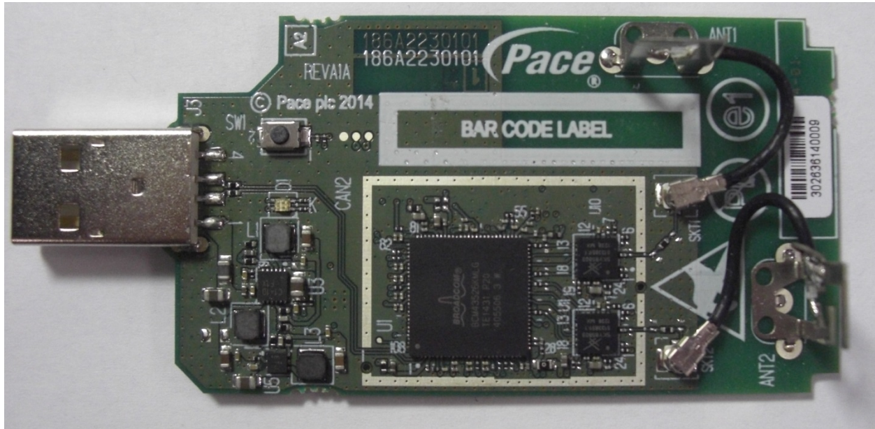
Internal Photo with Shield Removed
