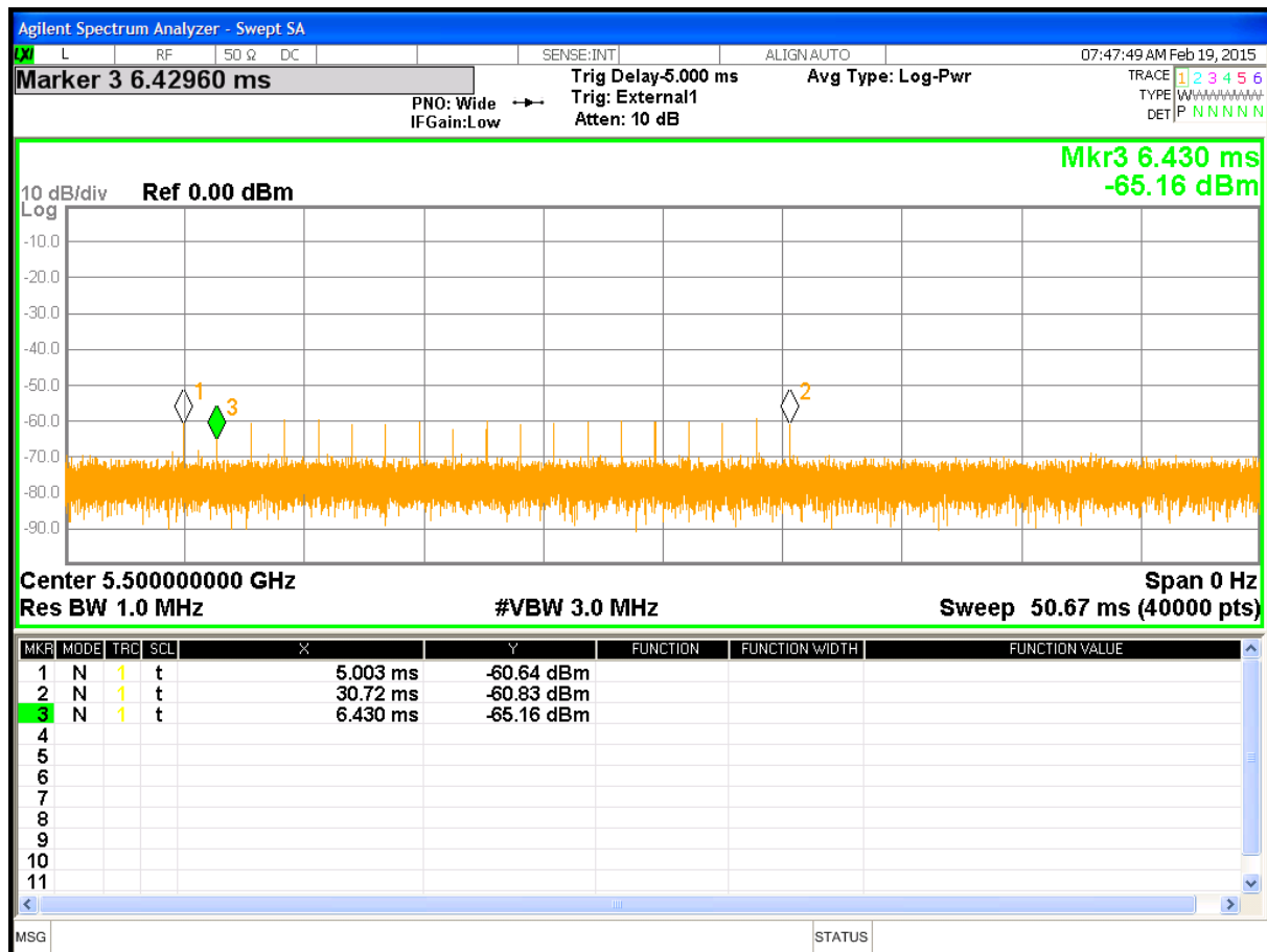
Figure 1: 5500 MHz Radar Pulse Type 0 at Master
