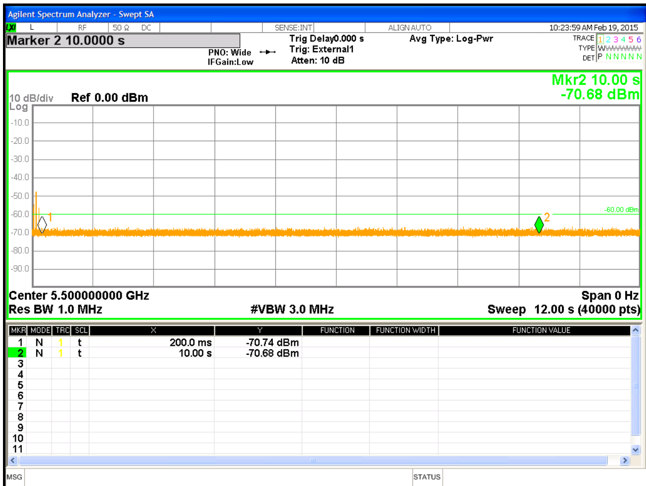
Figure 2: Channel move time, signal plotted 10 secs after radar signal is applied at 5500 MHz for 20MHz BW
