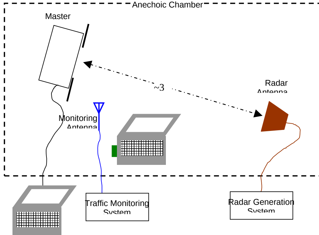
Figure 1 Test Configuration for radiated Measurement Method
