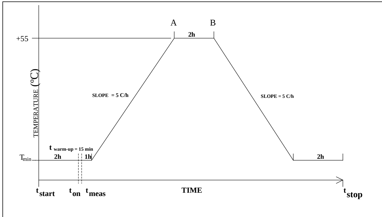
Figure 2-1. Temperature Gradient.
