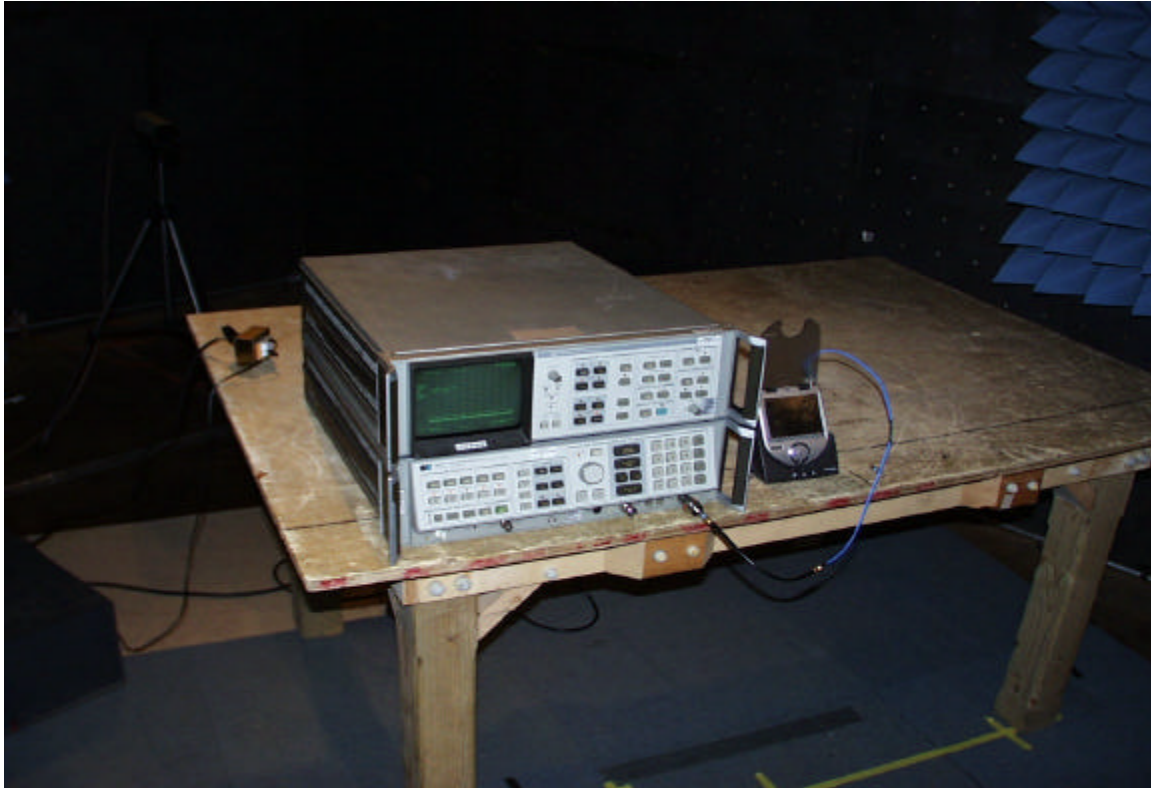
FREQUENCY/VOLTAGE SETUP
