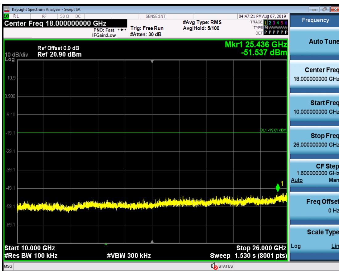
RF Conducted Spurious Emissions 2DH5 2402
