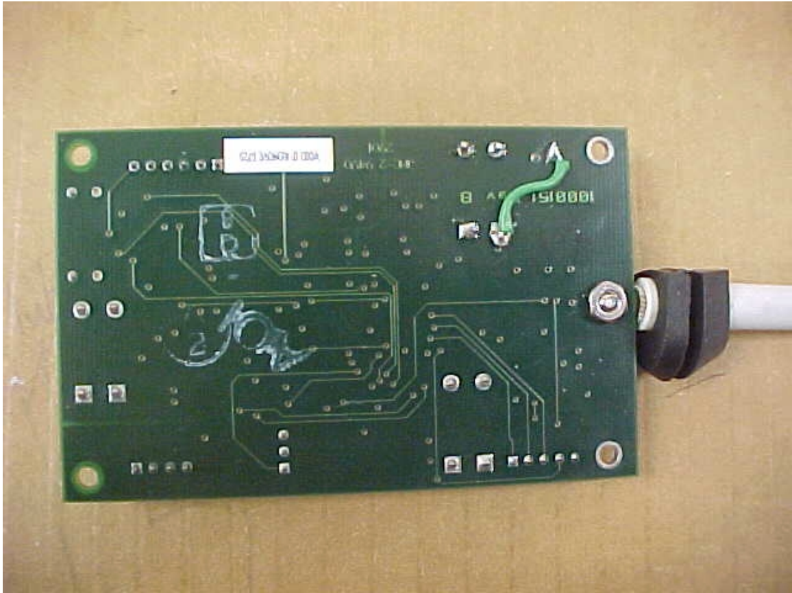
Close look at the Rear EUT Model PTL S 2000152
