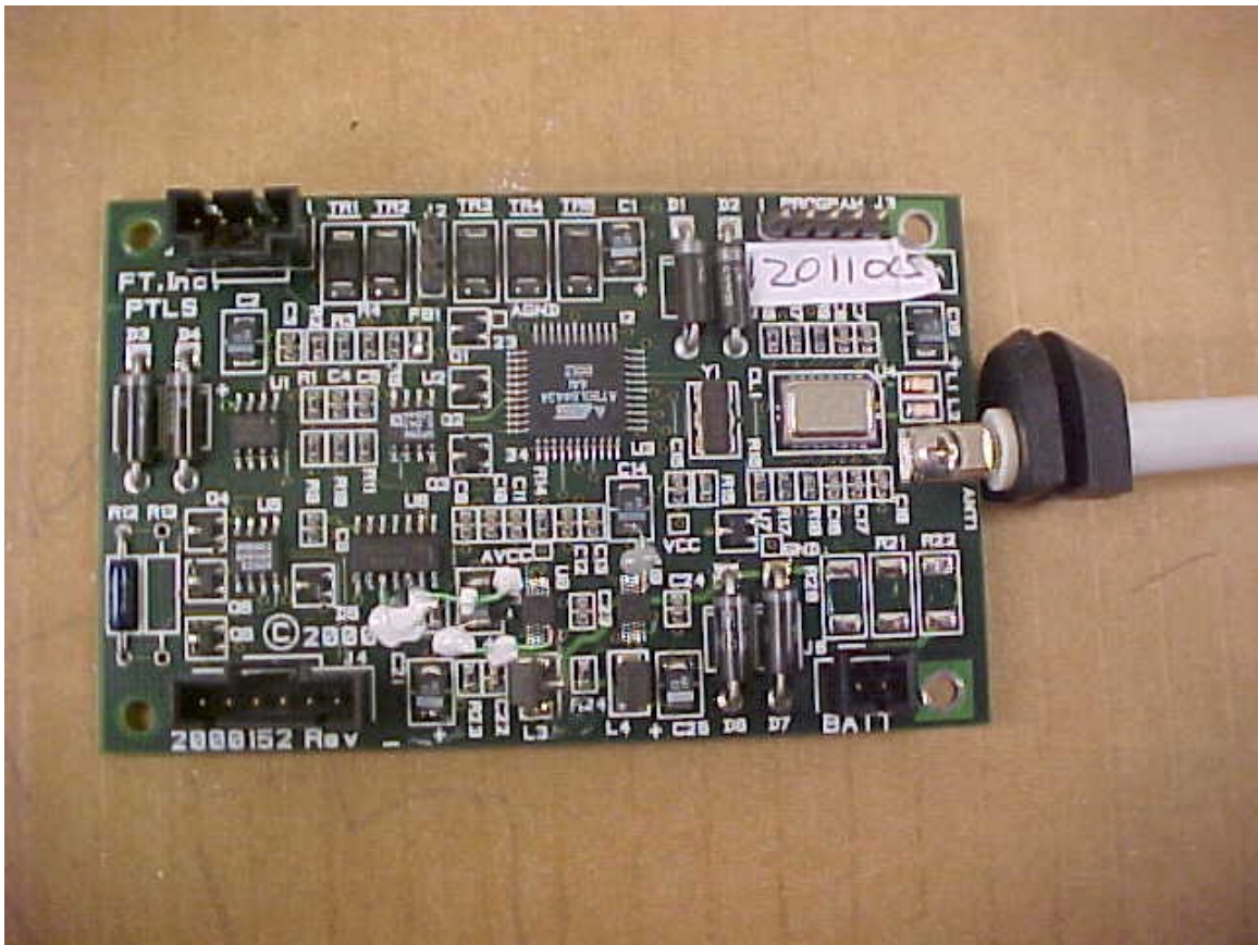
Close Look at the Front EUT Model PTL S 2000152
