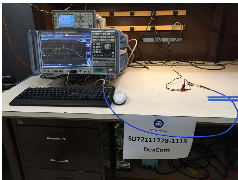
Conducted Testing
