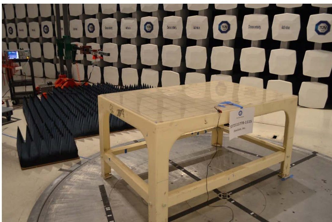
Radiated Emissions
