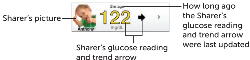
Figure 14. Follower Information
