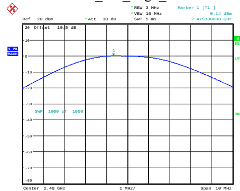
BLE_2M_High_Channel
