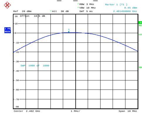
BLE_2M_Low_Channel
