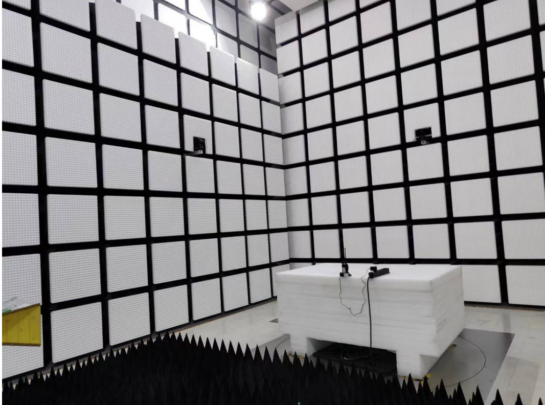
Radiated Emission Above 1GHz View M2
