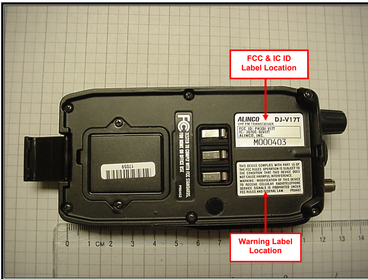
Photograph 1: FCC/IC ID and Warning Label locations
