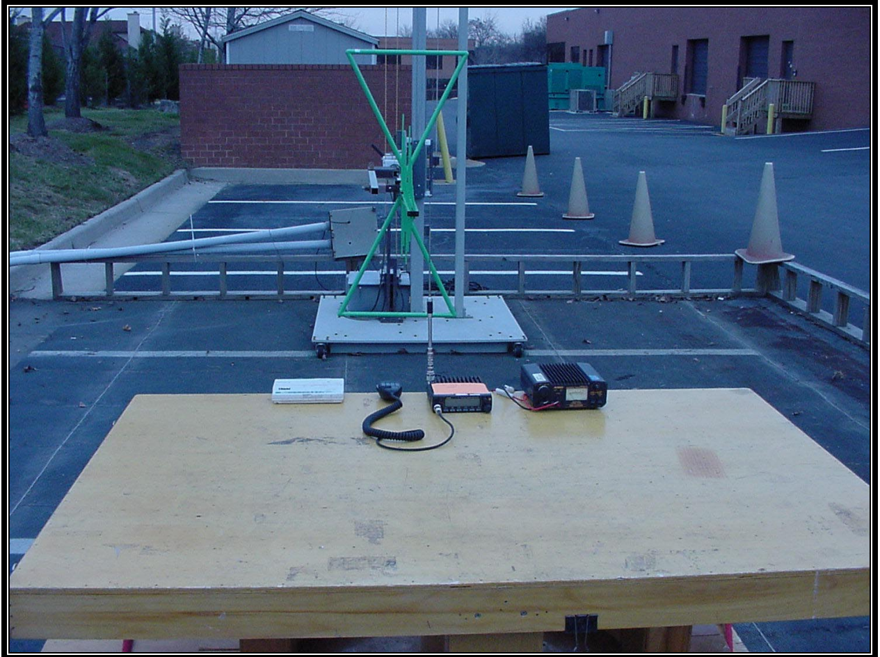
PHOTOGRAPH 2: RADIATED TEST CONFIGURATION (FRONT VIEW)
