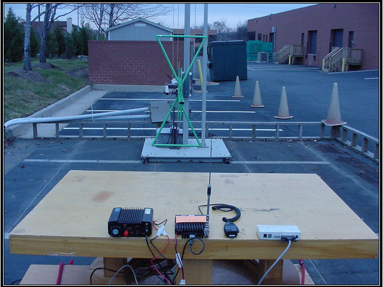
PHOTOGRAPH 3: RADIATED TEST CONFIGURATION (REAR VIEW)
