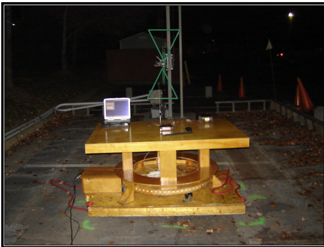
Photograph 3: Radiated Emissions Test Configuration (Front View)
