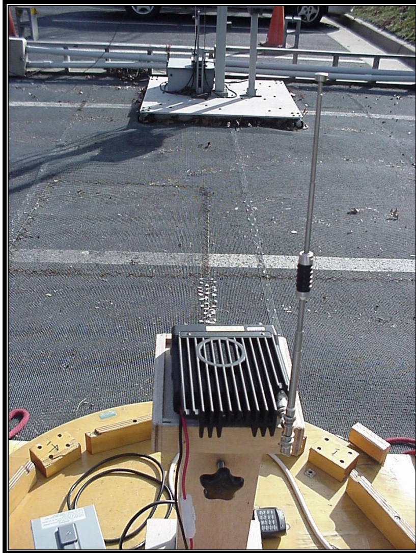
Photograph 4: Radiated Emissions Test Configuration (Rear View)
