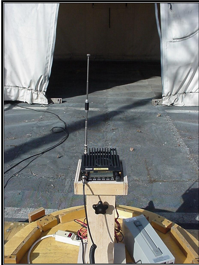
Photograph 3: Radiated Emissions Test Configuration (Front View)
