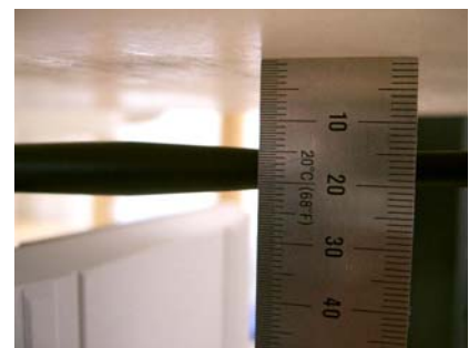
Fig. 21. Body SAR Test Setup with Holster
