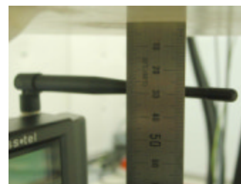
Fig. 21. Body SAR Test Setup with Holster
