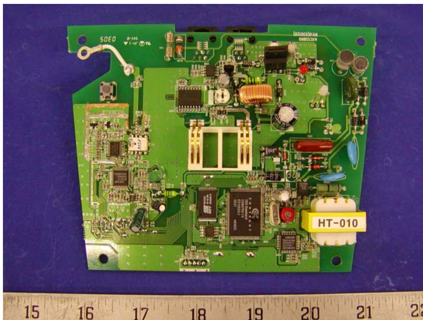
Base - Main Board Component View 2
