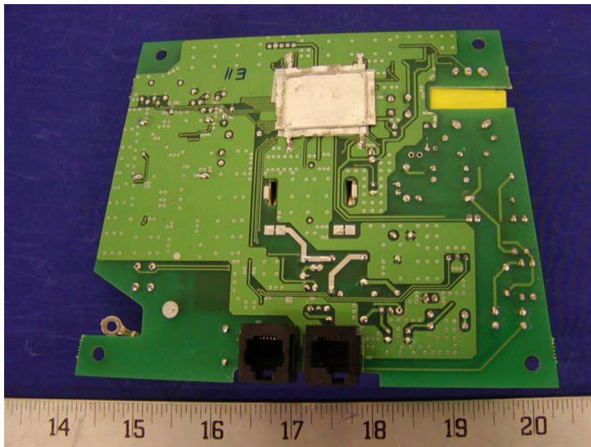
Base - Main Board Solder View 1
