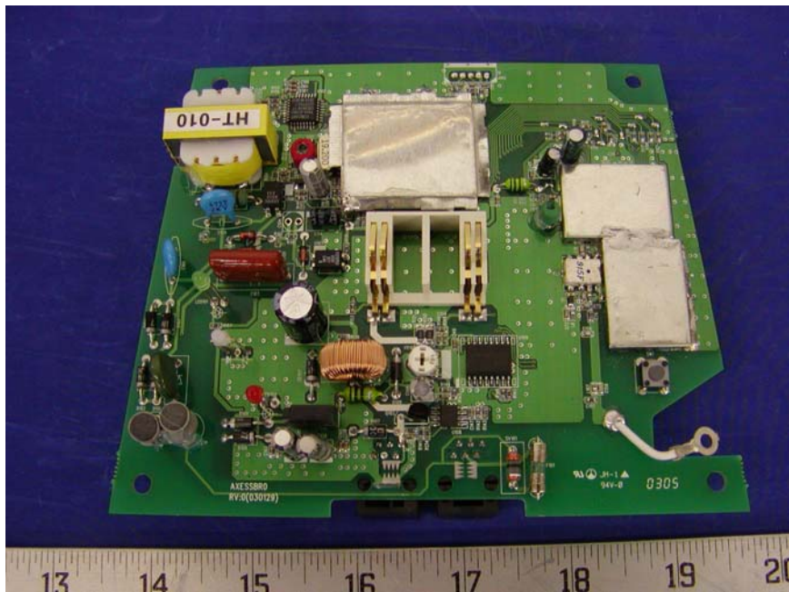
Base - Main Board Component View 1
