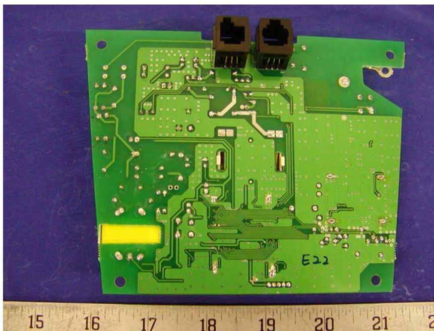
Base - Main Board Solder View 2
