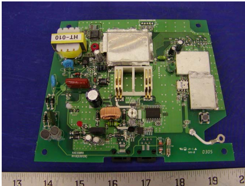
Base - Main Board Component View
