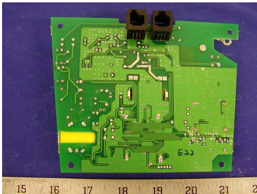
Base - Main Board Solder Shielded Removed View
