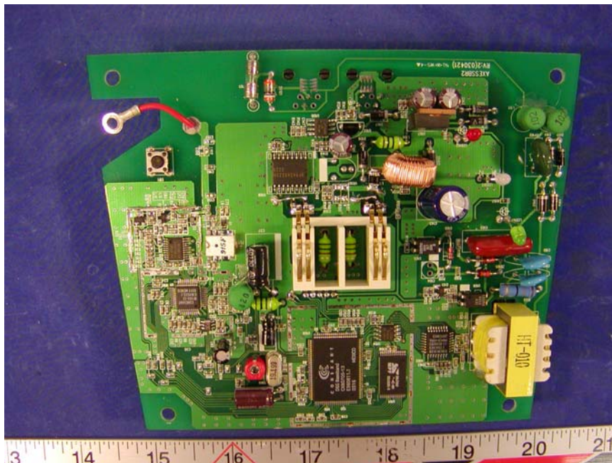
Base - Main Board Component Shielded Removed View
