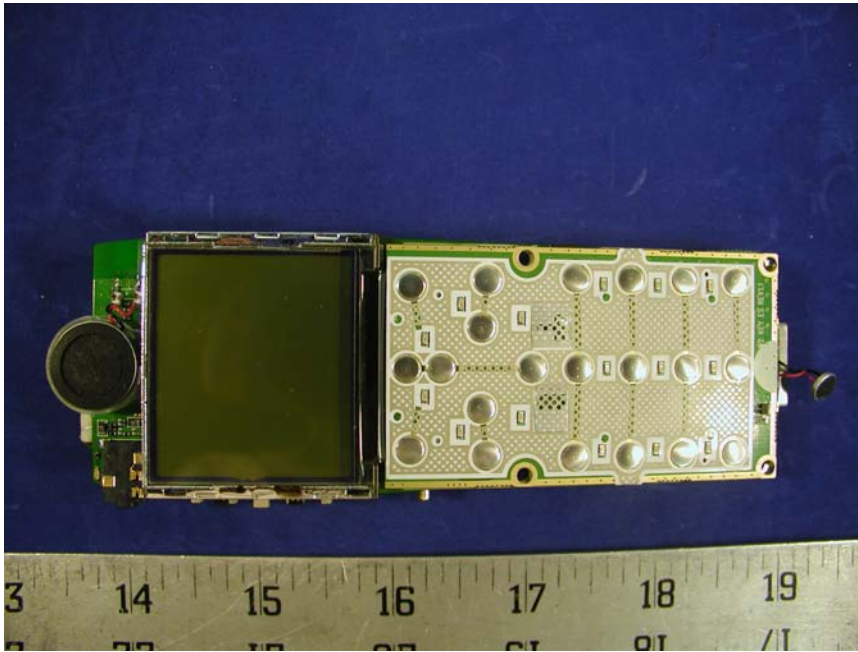
EUT - Main Board Solder View
