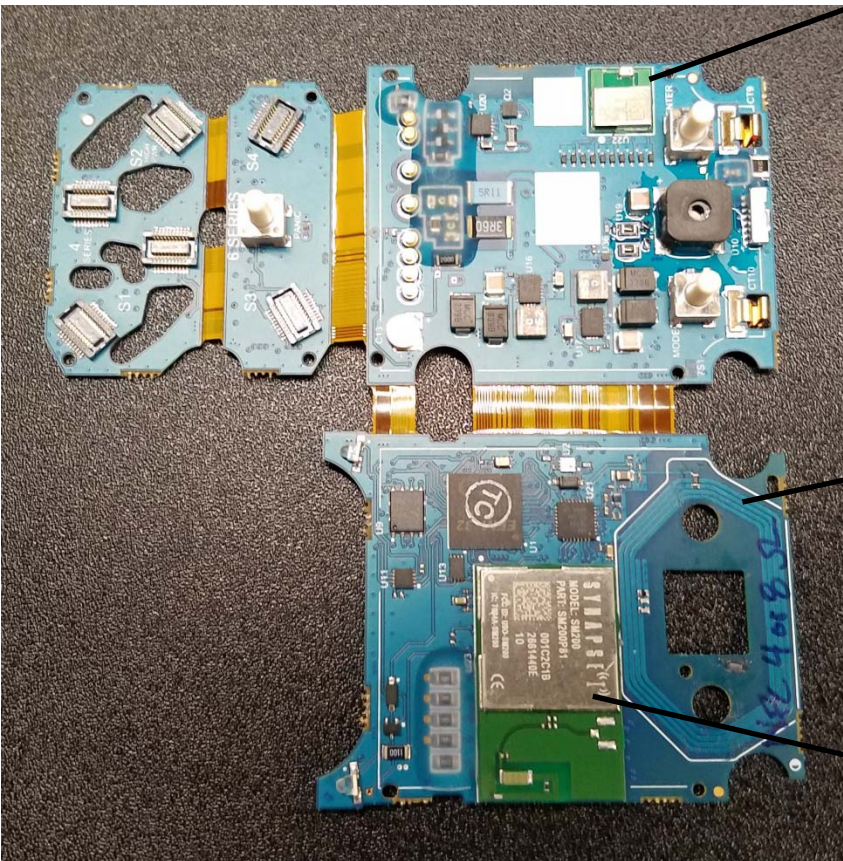
View of circuit board w/o sensors or plastic carrier (side 1)
