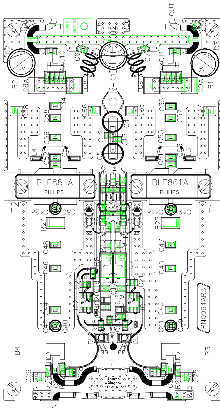
Component layout SCH0192AR0
