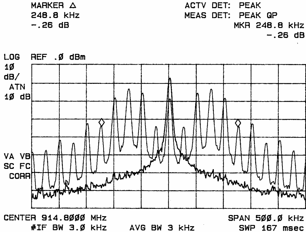
Figure eight 99.5% occupied bandwidth plot
