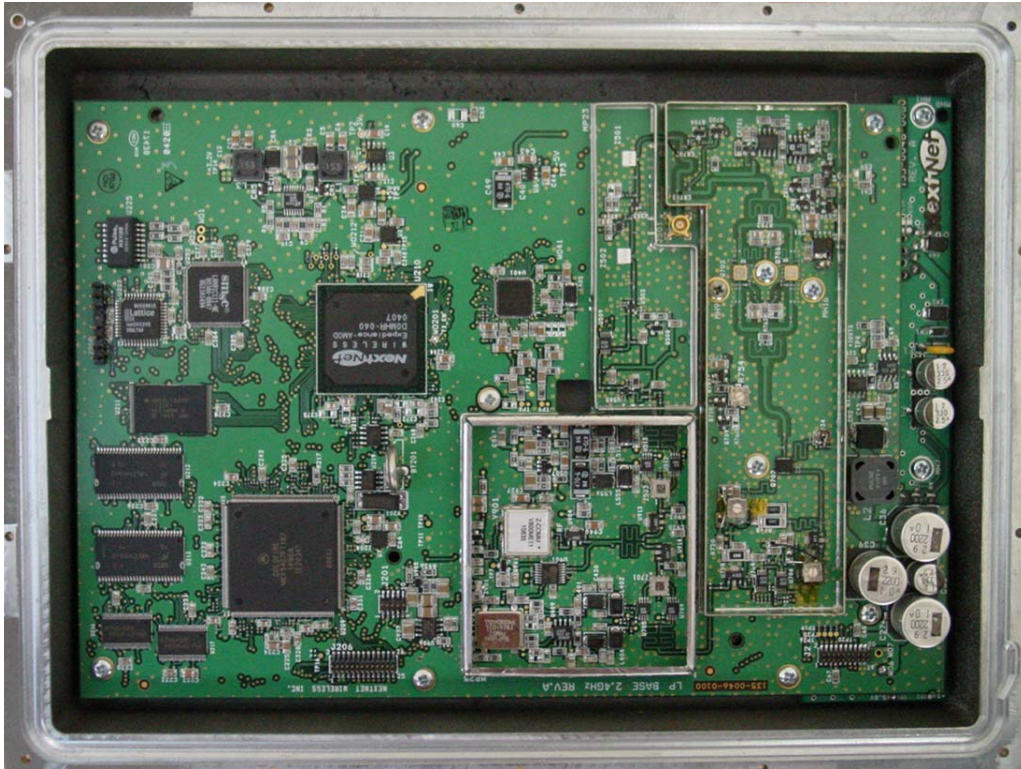
RF Board and Interconnect Board (Component Side / No Shields)
