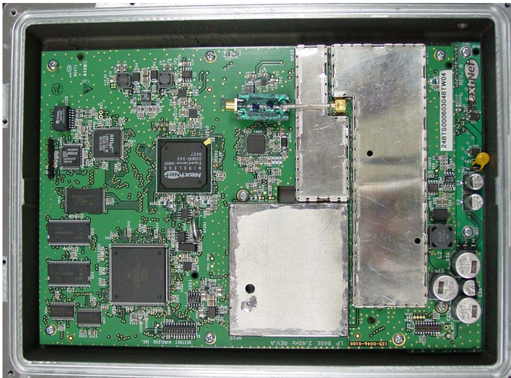
RF Board, Interconnect Board, Low Pass Filter board (Component Side / With Shields)
