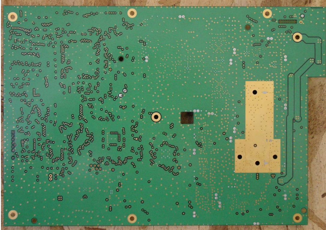
RF Board (Bottom Side)
