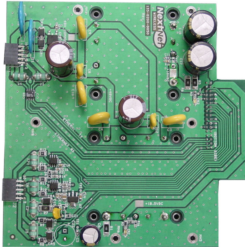
Power Supply Board Top Side View
