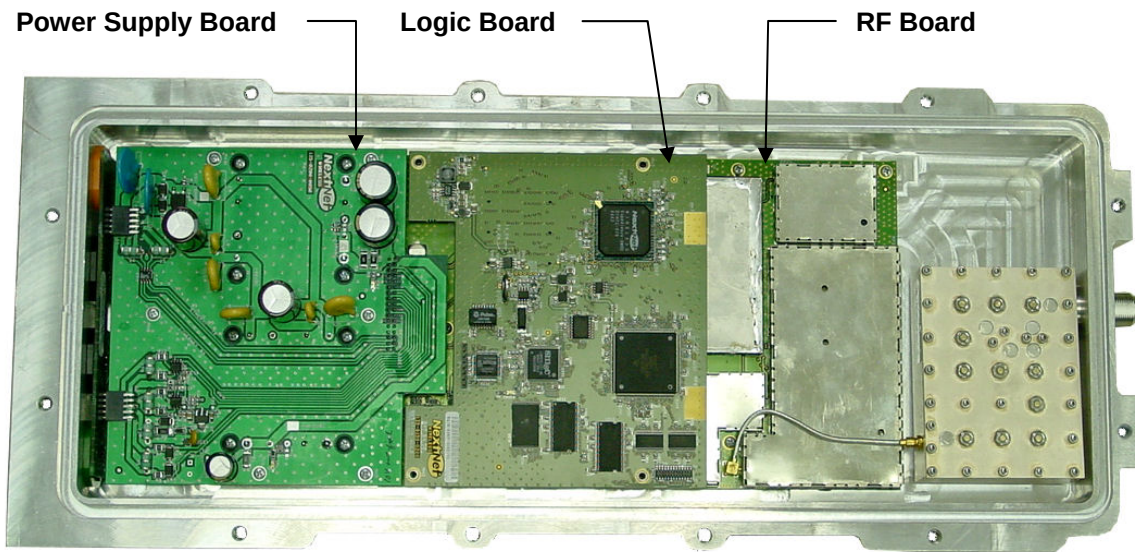
Chassis With Cover Removed
