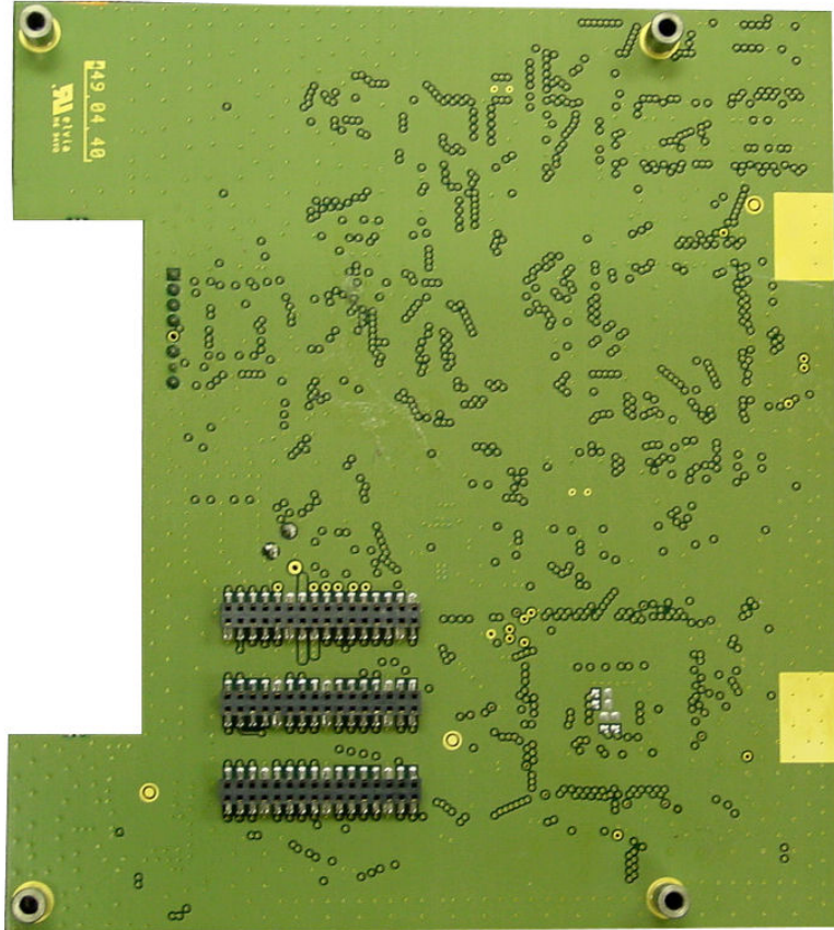
Logic Board Bottom View
