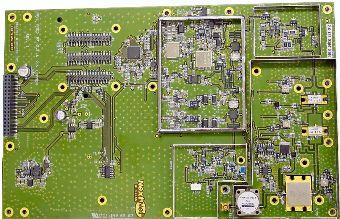
RF Board Top View Without Shields Installed
