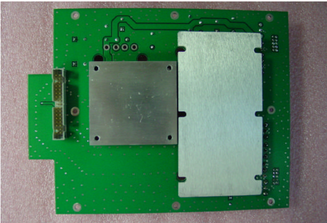
Power Supply Board Solder Side
