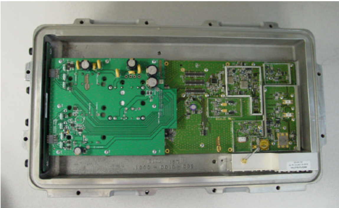
RF Board, Power Supply Board and Input Connector Board
