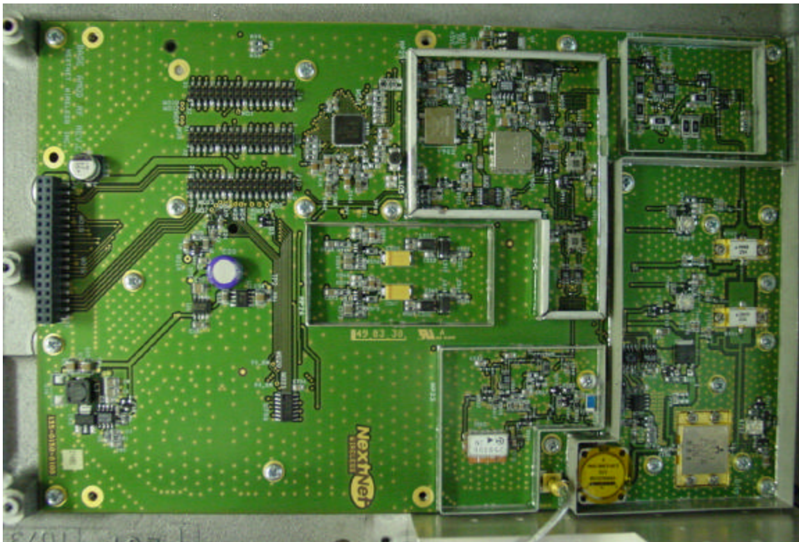
RF Board Component Side (no shields)
