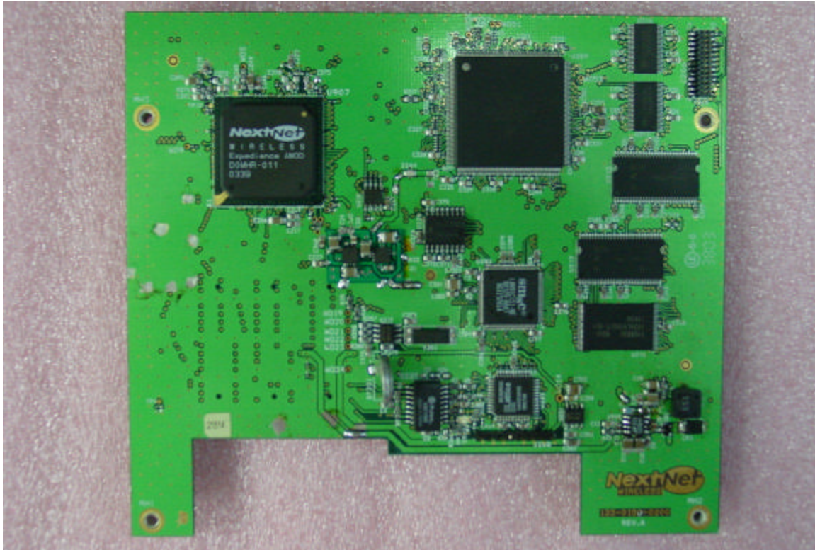
Logic Board Component Side
