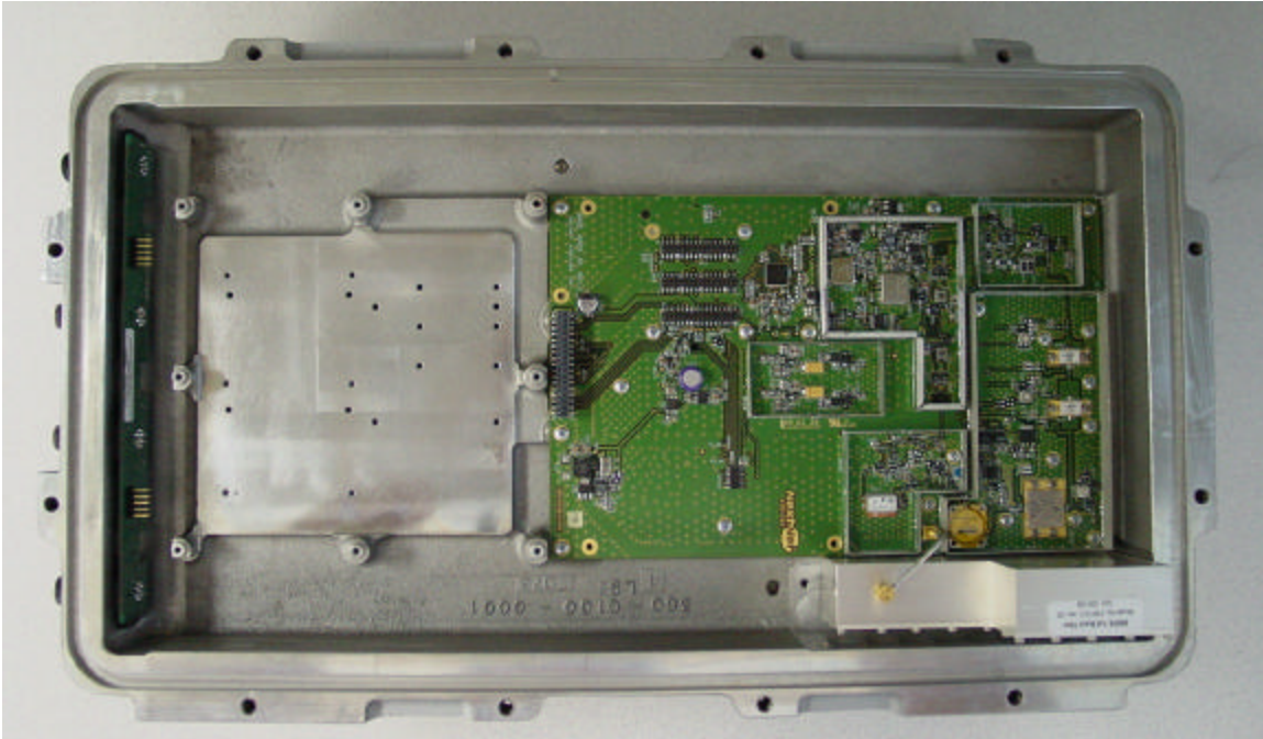
RF Board and Input Connector Board
