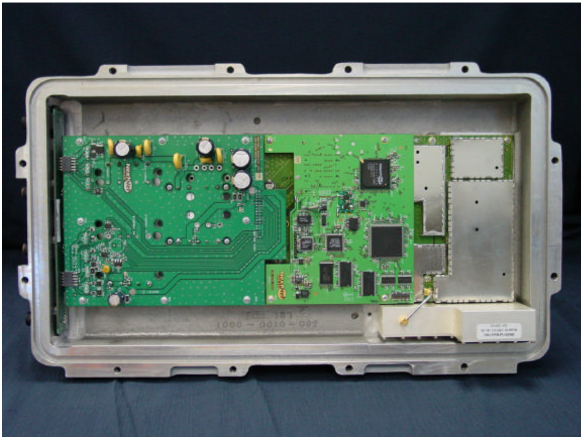
Logic Board, RF Board, Power Supply Board and Input Connector Board
