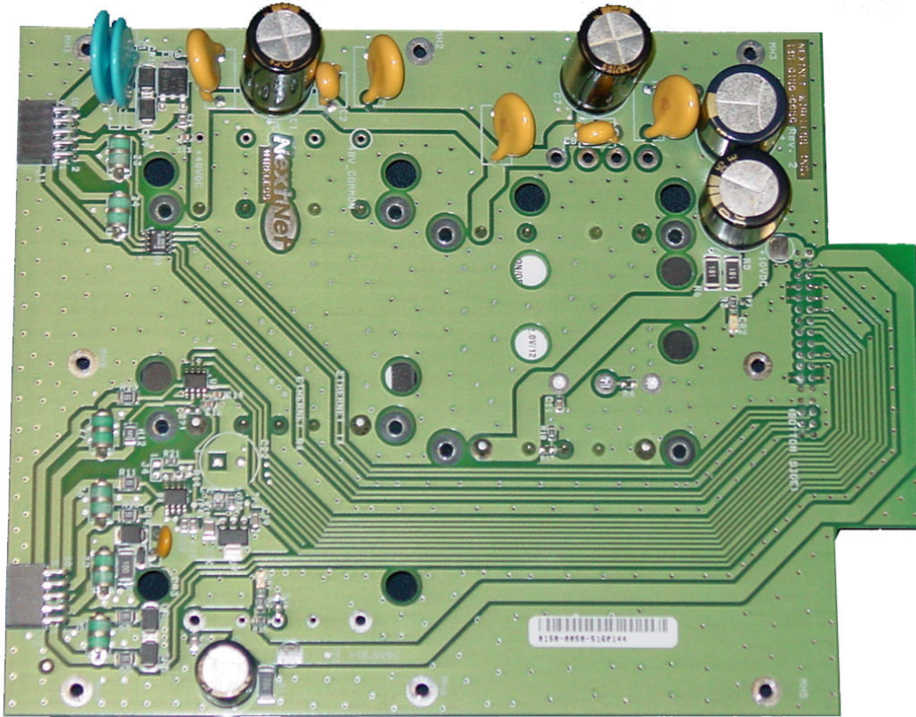
Power Supply Board Top Side View
