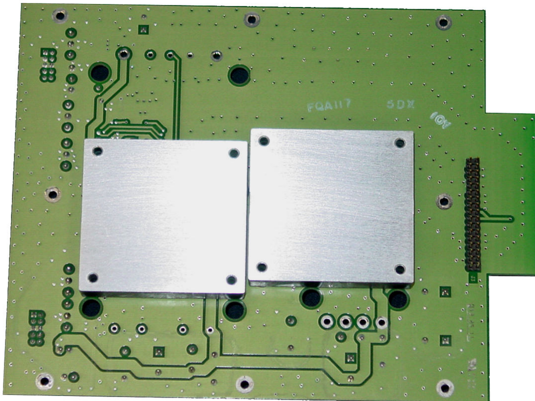
Power Supply Board Bottom View
