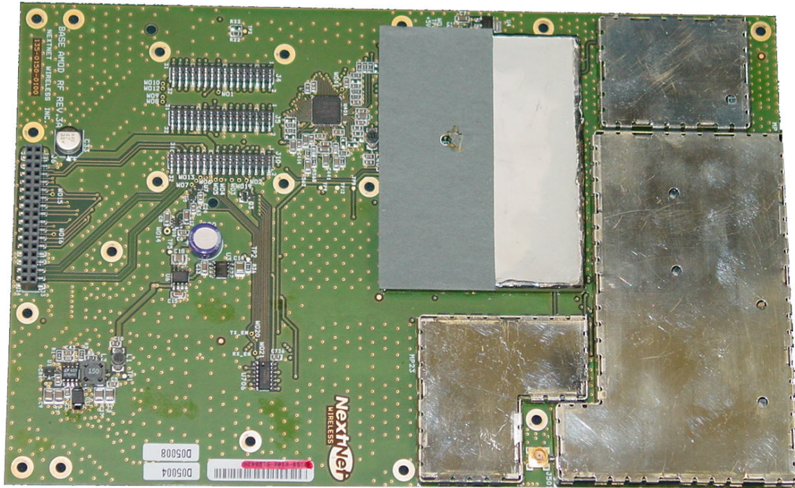
RF Board Top View With Shields Installed
