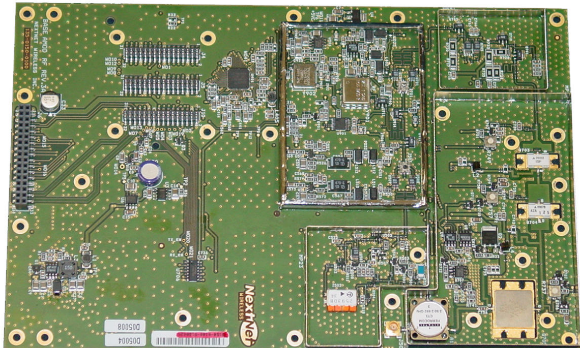
RF Board Top View Without Shields Installed
