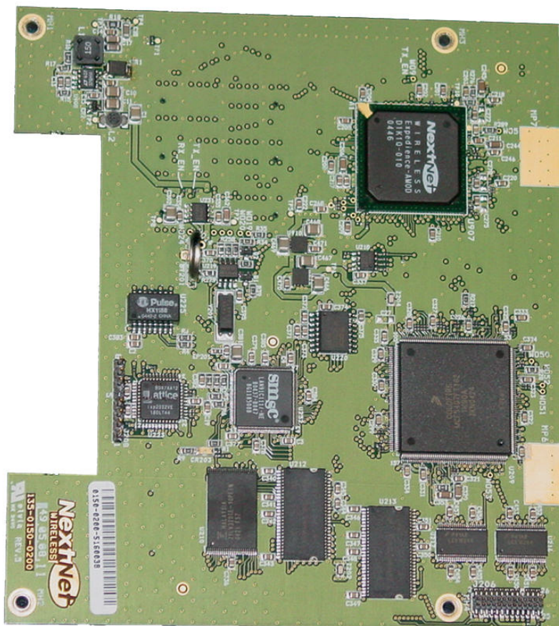
Logic Board Top View
