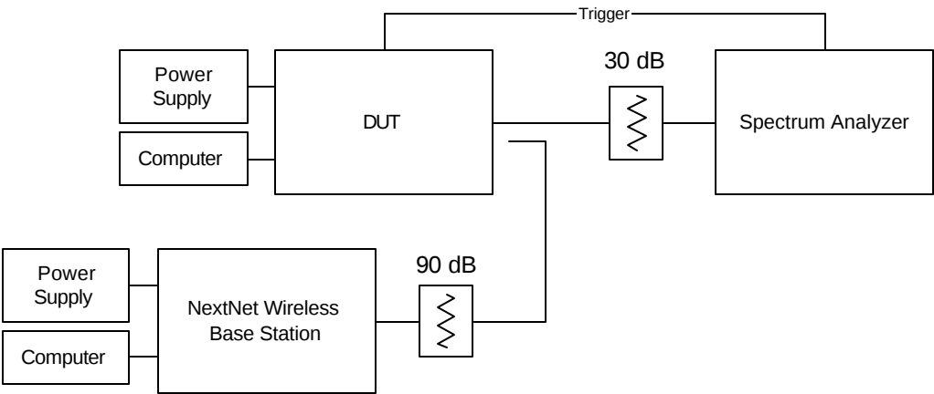
CPE power measurement
