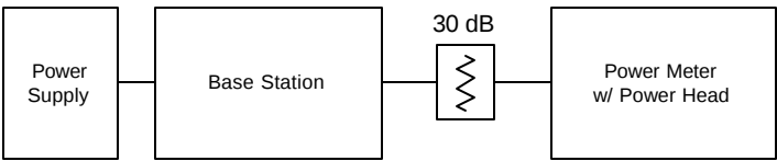
Base Station power verification
